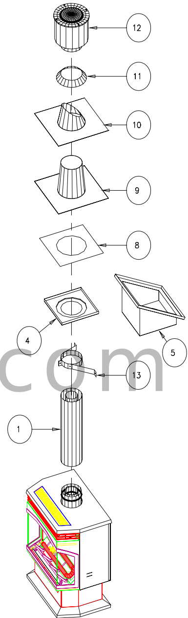
VERTICAL TERMINATION
