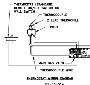
Figure 11: Thermostat Wiring
