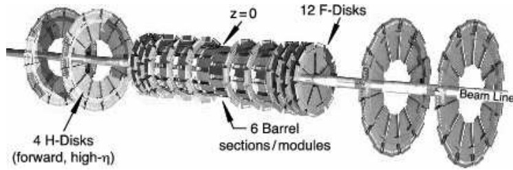
Figure 3.4: The disk/barrel configurations of the SMT sensors.
