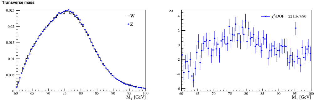
Figure 7.7: Identical comparison as in Fig 7.6, except that the comparison is between Z and true W events. Notice the proper extra smearing of hard recoil of Z events in Fig 7.6 appears to be slightly under-smearred, with respect to the true W events.
