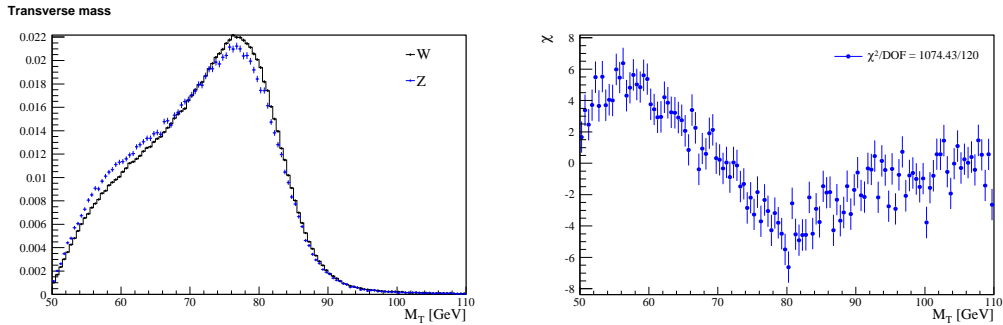
Figure 6.25: M_T comparison of W and Z . p_T^e > 25 \text{ GeV} and \cancel{E}_T > 25 \text{ GeV} , tight electron in EC, loose electron in CC or EC (full acceptance).
