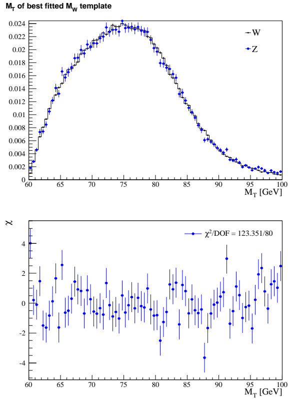
Figure 9.5: Comparison between M_T of W data and the best fitted M_T template from Z data, which is 80435 MeV. Range between 66 GeV and 96 GeV is used in the mass fitting.
