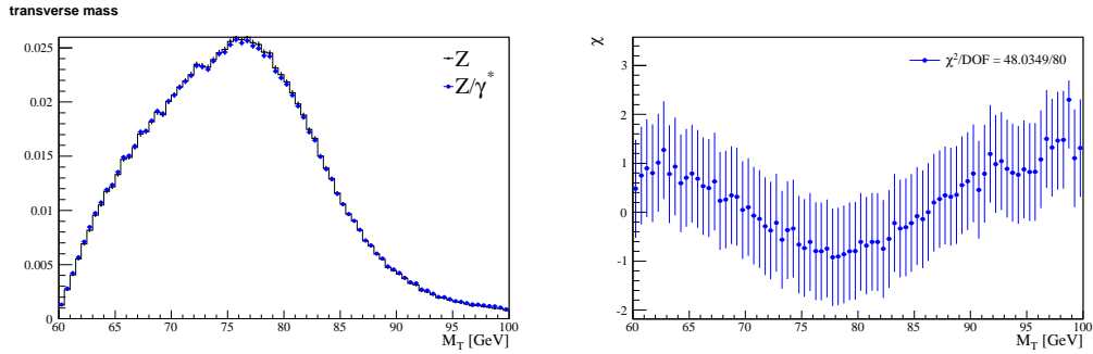
Figure 5.25: Transverse mass of Z \rightarrow ee and Z/\gamma^* \rightarrow ee events in resbos . They are fast Monte Carlo simulation with realistic smearing after final event selections. Z \rightarrow ee events are subset of the 5 \text{ fb}^{-1} Z/\gamma^* sample.
