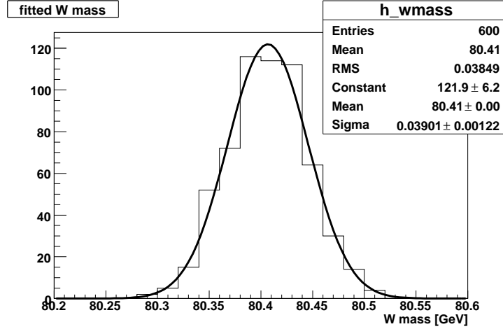
Figure 6.13: 1Z1W. Fitted M_W of the 600 ensemble tests (each of 1 \text{ fb}^{-1} events) on the generator level, no cuts. \sigma(M_W) = 39 \text{ MeV} is the true statistical uncertainty.
