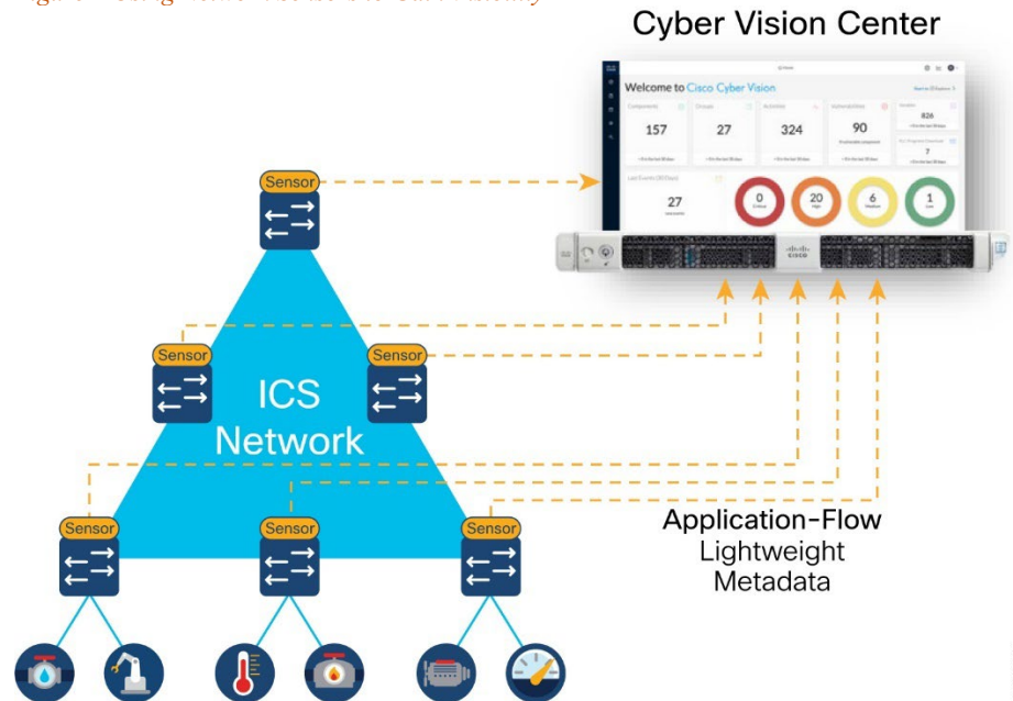
Figure 2 Using Network Sensors to Gain Visibility
