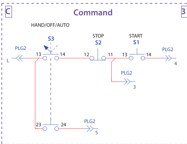
Figure 38 - Hand-OFF-Auto and Start-Stop Command Kit Wiring Diagram
