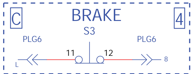
Figure 42 - Command Bypass Kit Wiring Diagram
