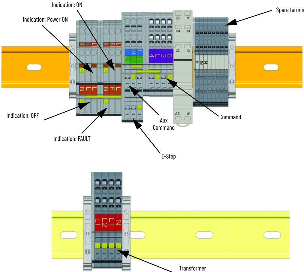
Figure 14 - SMC Flex Controller Snap-together Wiring
