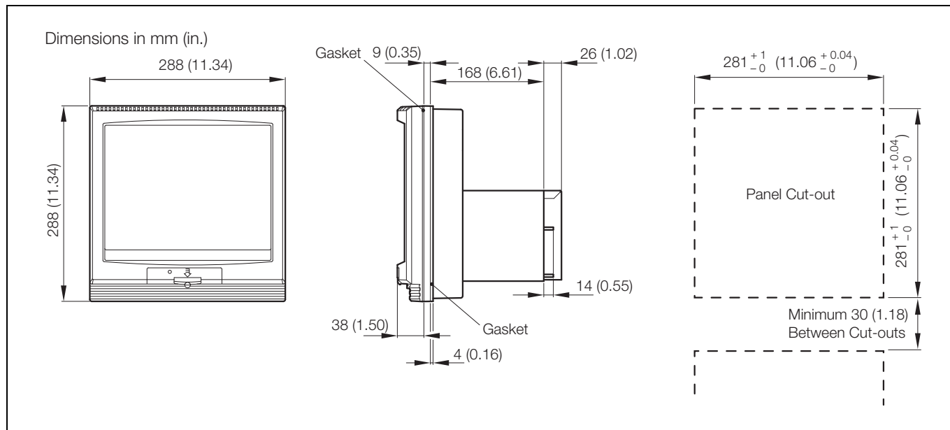
Fig. 7.3 Mounting Dimensions
