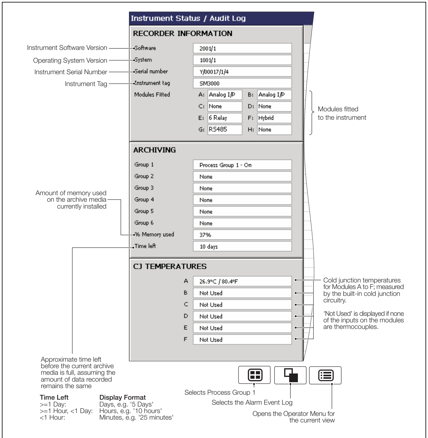
Fig. 4.11 Instrument Status
