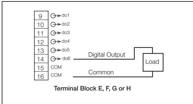
Fig. 7.13 Digital Output Connections
