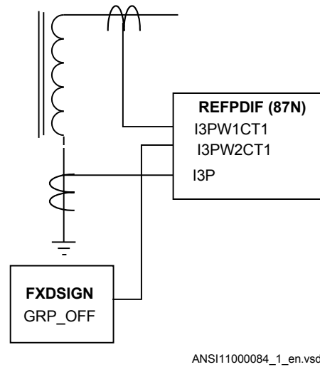
Figure 98: REFPDIF (87N) function inputs for normal transformer application
