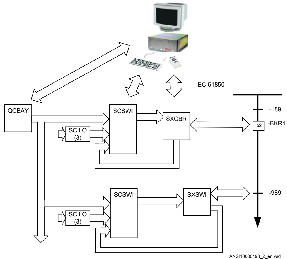
Figure 49: Signal flow between apparatus control function blocks
