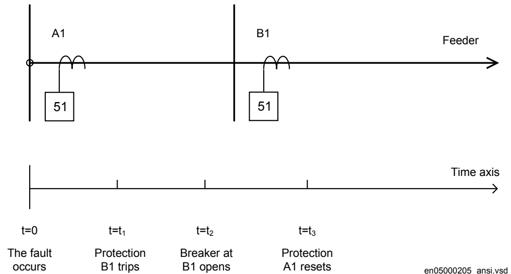
Figure 32: Sequence of events during fault
