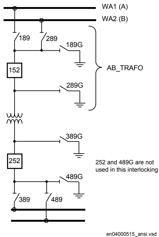
Figure 92: Switchyard layout AB_TRAFO (3)
