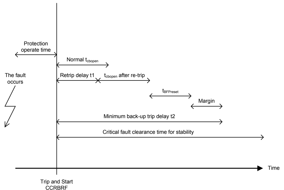
Figure 7: Time sequences for breaker failure protection setting
