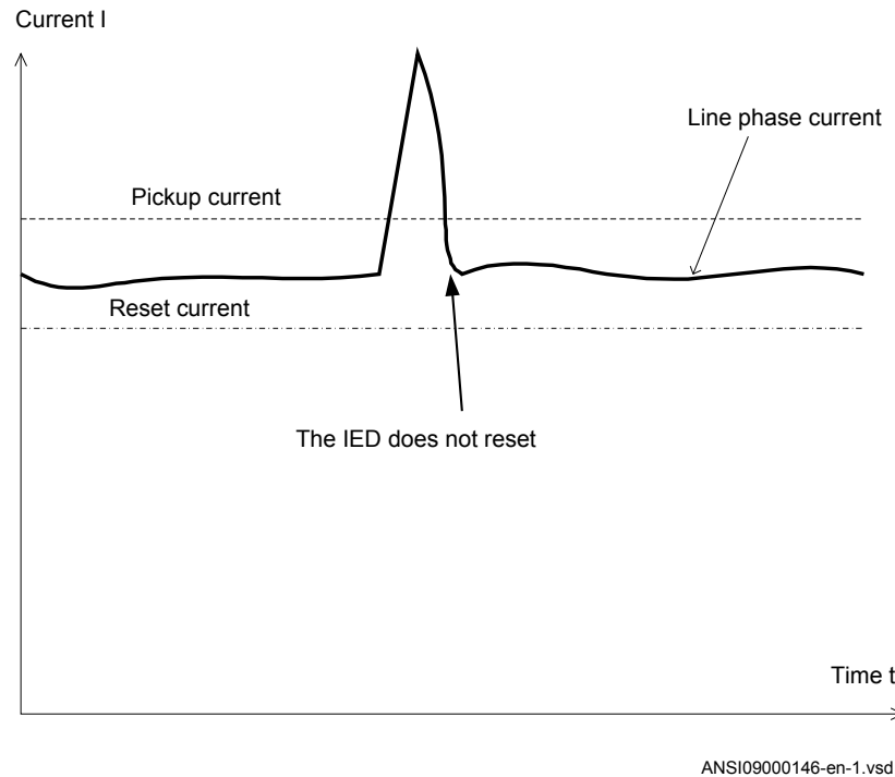
Figure 30: Pickup and reset current for an overcurrent protection
