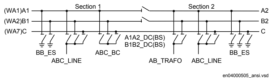
Figure 56: Busbars divided by bus-section disconnectors (circuit breakers)
