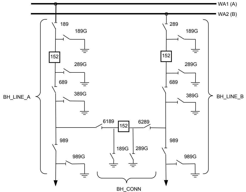
Figure 86: Switchyard layout breaker-and-a-half
