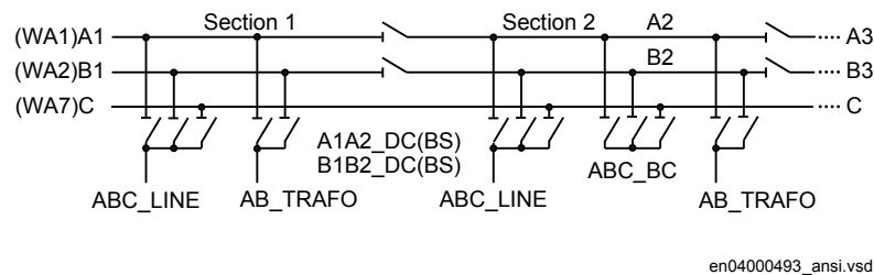
Figure 69: Busbars divided by bus-section disconnectors (circuit breakers)
