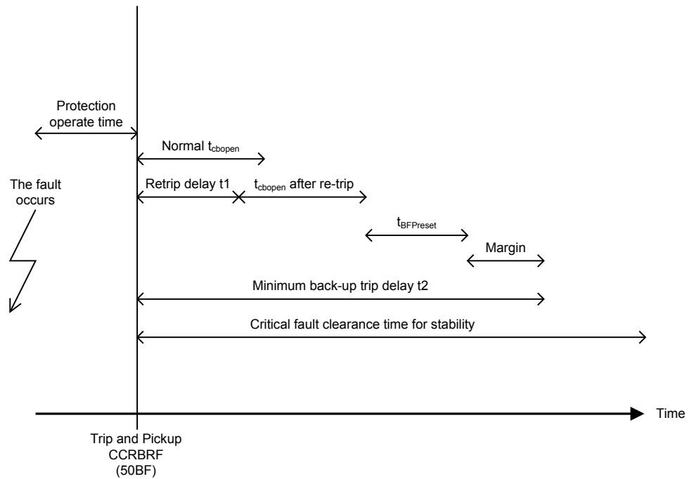
Figure 35: Time sequence
