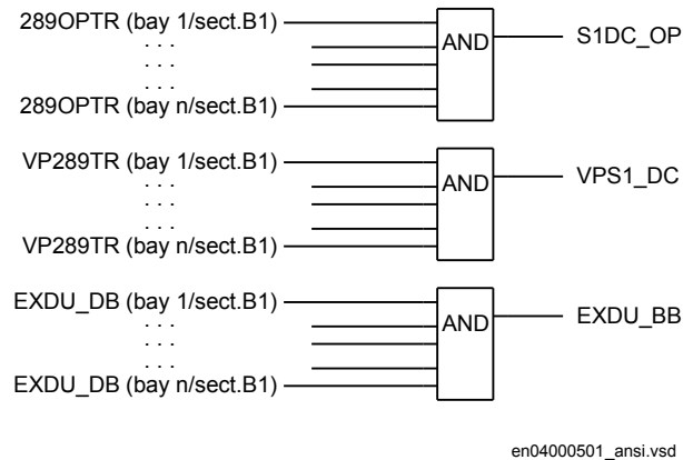
Figure 77: Signals from double-breaker bays in section B1 to a bus-section disconnecter
