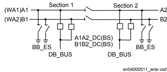
Figure 62: Busbars divided by bus-section disconnectors (circuit breakers)
