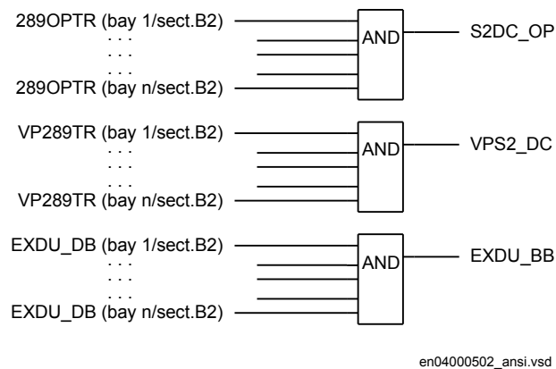
Figure 78: Signals from double-breaker bays in section B2 to a bus-section disconnecter
