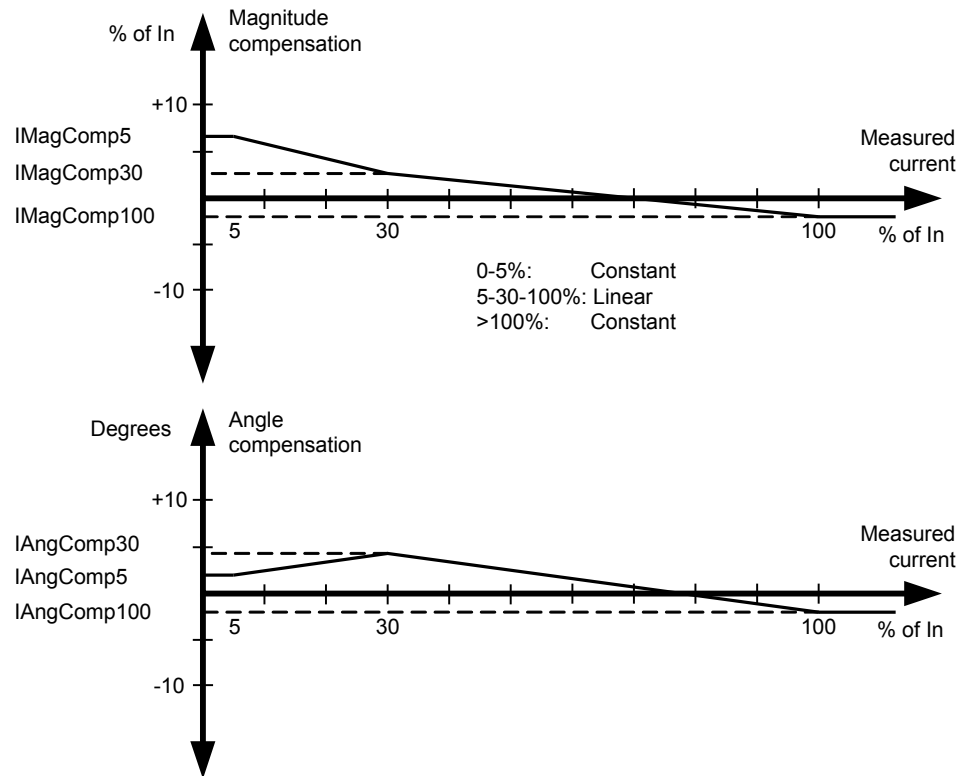
Figure 99: Calibration curves
