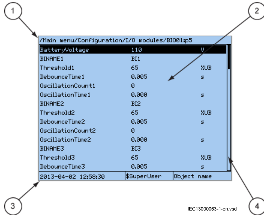
Figure 18: Display layout
