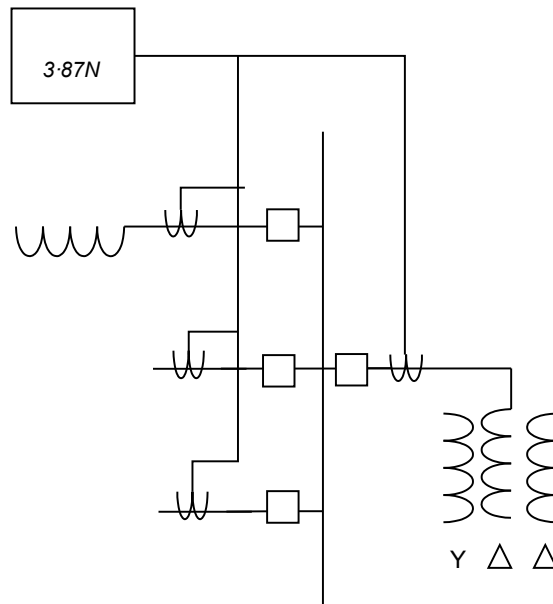
Figure 23: Application of a 1Ph High impedance differential protection HYPDIF (87) function as busbar protection
