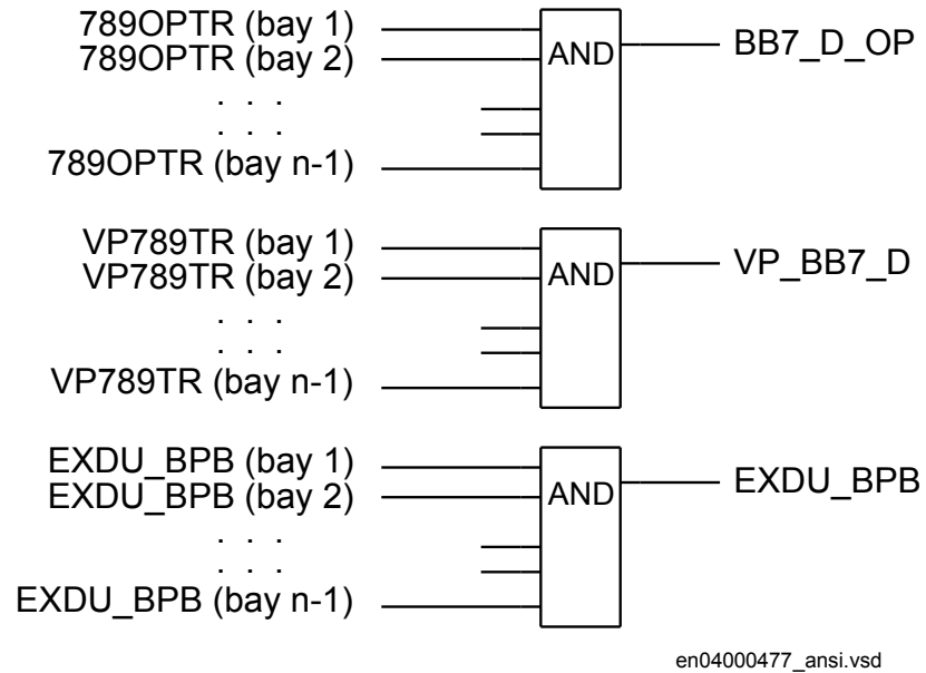
Figure 89: Signals from bypass busbar in line bay n
