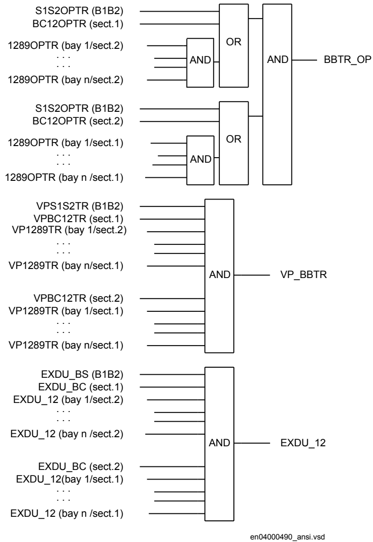
Figure 66: Signals from any bays for a bus-section circuit breaker between sections A1 and A2
