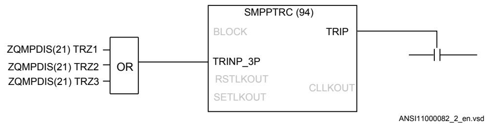
Figure 95: Tripping logic common 3-phase output SMPPTRC (94) is used for a simple three-pole tripping application
