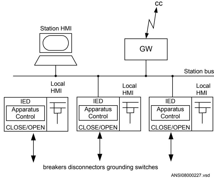
Figure 48: Overview of the apparatus control functions
