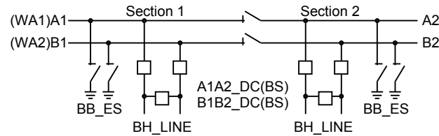
Figure 63: Busbars divided by bus-section disconnectors (circuit breakers)
