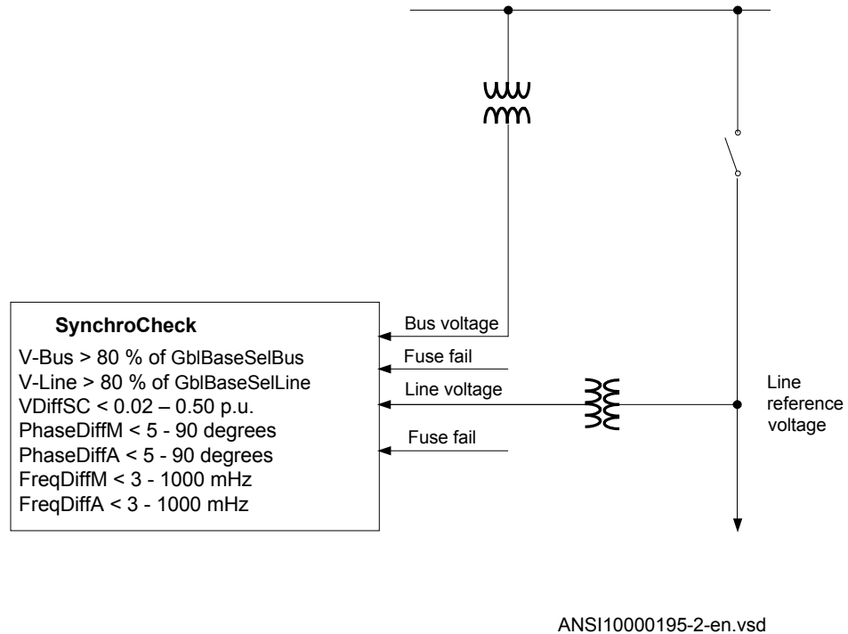
Figure 42: Principle for the synchronism check function
