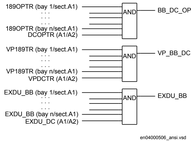
Figure 57: Signals from any bays in section A1 to a busbar grounding switch in the same section
