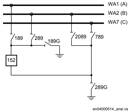
Figure 80: Switchyard layout ABC_BC (3)
