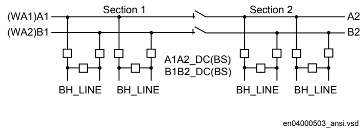
Figure 79: Busbars divided by bus-section disconnectors (circuit breakers)
