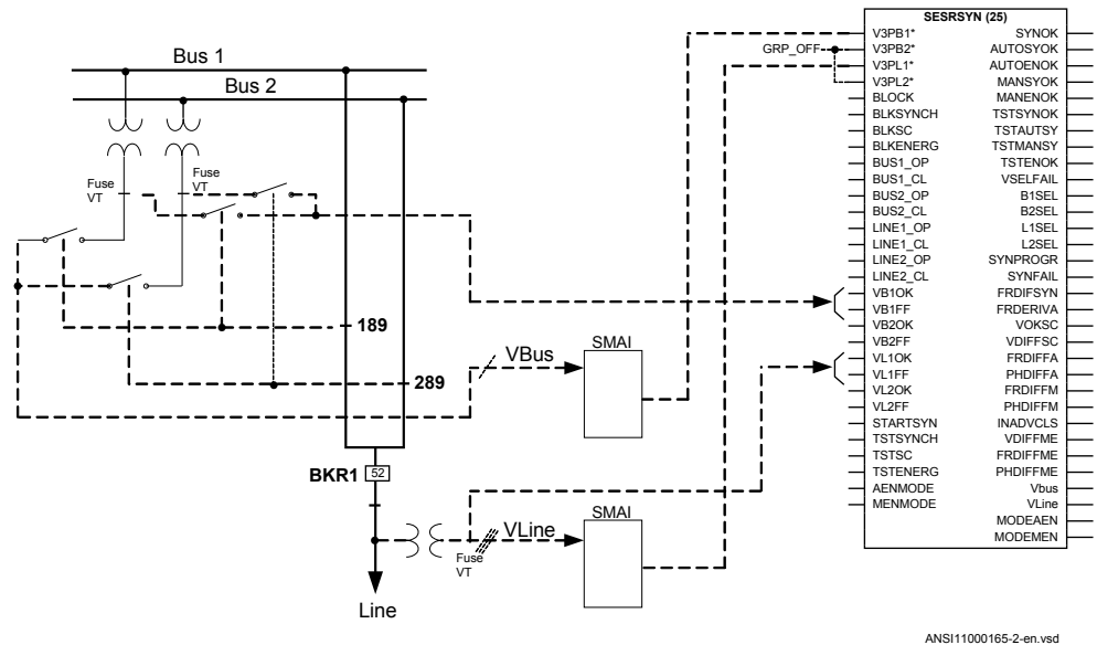
Figure 46: Connection of SESRSYN (25) function block in a single breaker, double busbar arrangement with external voltage selection
