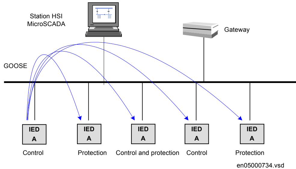
Figure 105: Example of a broadcasted GOOSE message
