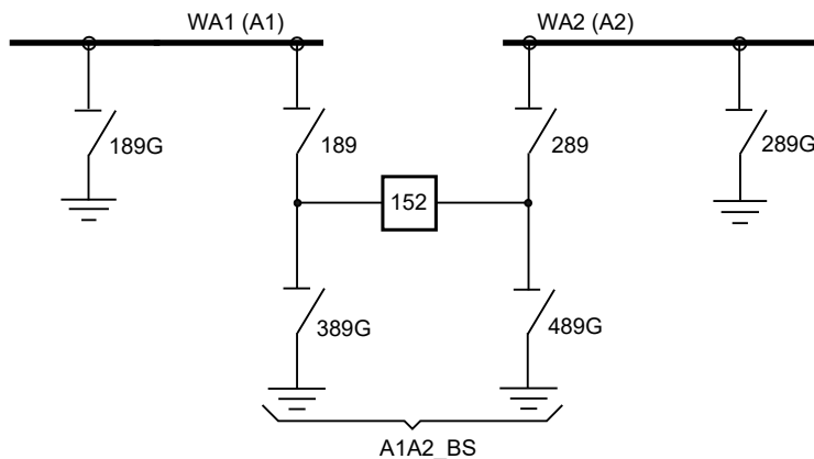
Figure 64: Switchyard layout A1A2_BS (3)
