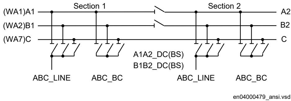
Figure 90: Busbars divided by bus-section disconnectors (circuit breakers)
