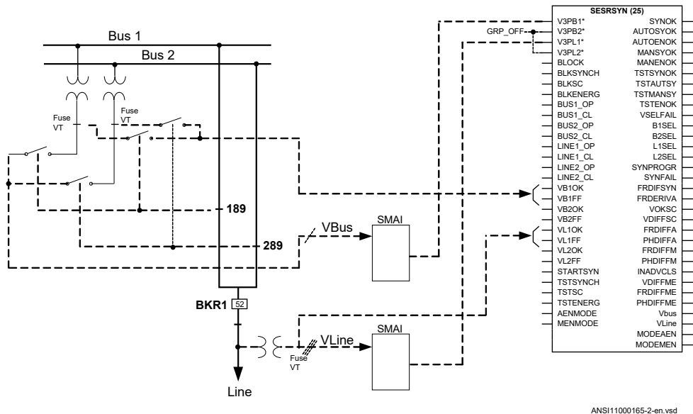
Figure 46: Connection of SESRSYN (25) function block in a single breaker, double busbar arrangement with external voltage selection
