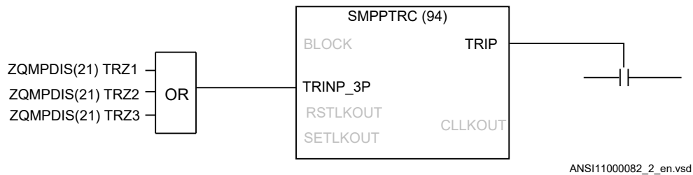
Figure 95: Tripping logic common 3-phase output SMPPTRC (94) is used for a simple three-pole tripping application
