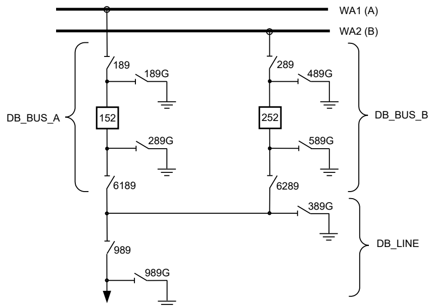
Figure 87: Switchyard layout double circuit breaker
