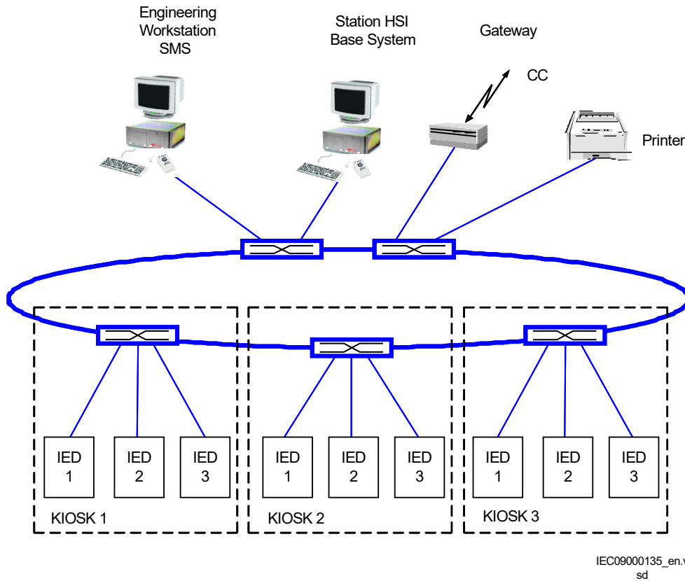
Figure 104: Example of a communication system with IEC 61850-8-1
