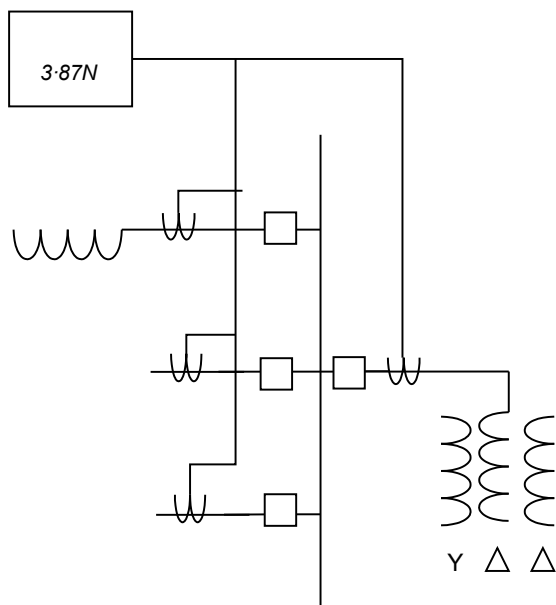
Figure 23: Application of a 1Ph High impedance differential protection HZPDIF (87) function as busbar protection
