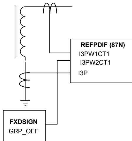
Figure 98: REFDPDIF (87N) function inputs for normal transformer application
