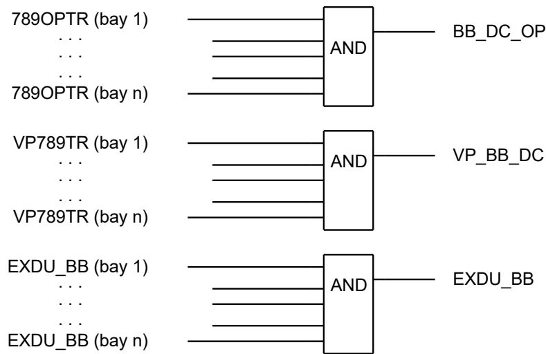
Figure 61: Signals from bypass busbar to busbar grounding switch
