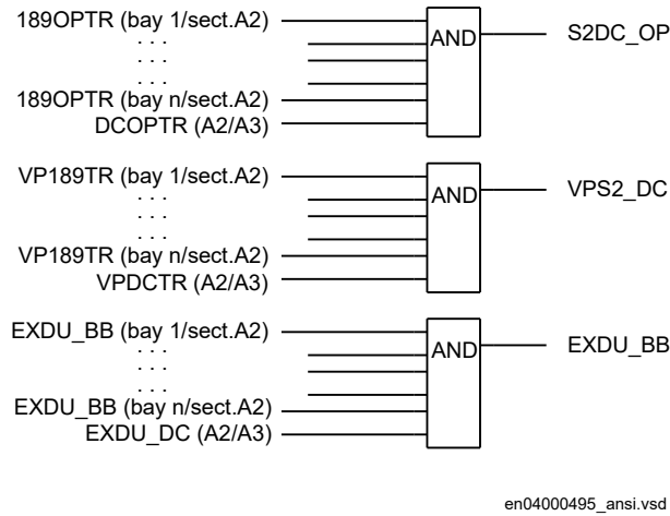
Figure 71: Signals from any bays in section A2 to a bus-section disconnecter
