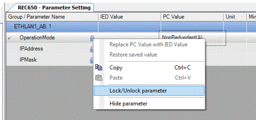
Figure 110: PRP1 Configured in the Parameter Setting tool
