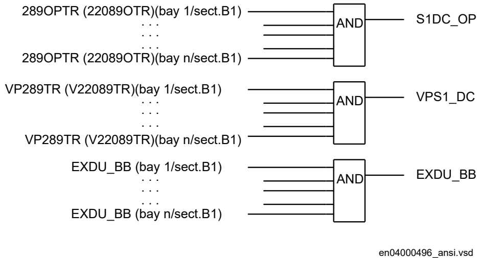
Figure 72: Signals from any bays in section B1 to a bus-section disconnecter
