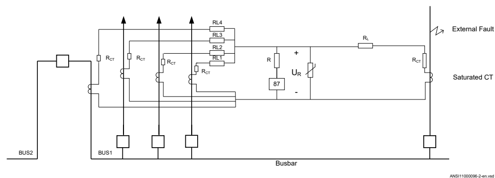
Figure 6: Connection of the high impedance differential protection and external fault
