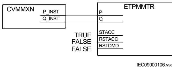
Figure 103: Connection of energy calculation and demand handling function ETPMMTR to the measurements function (CVMMXN)
