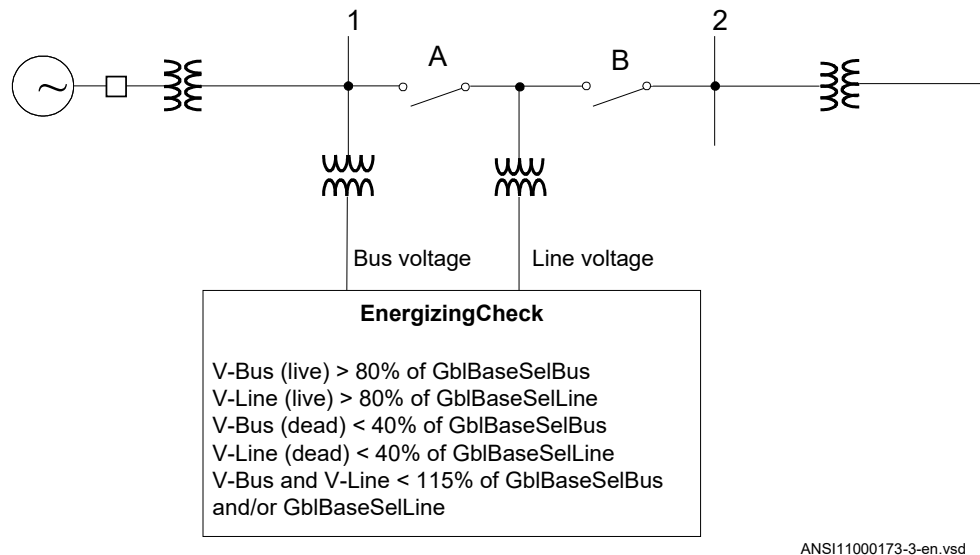
Figure 43: Principle for the energizing check function
