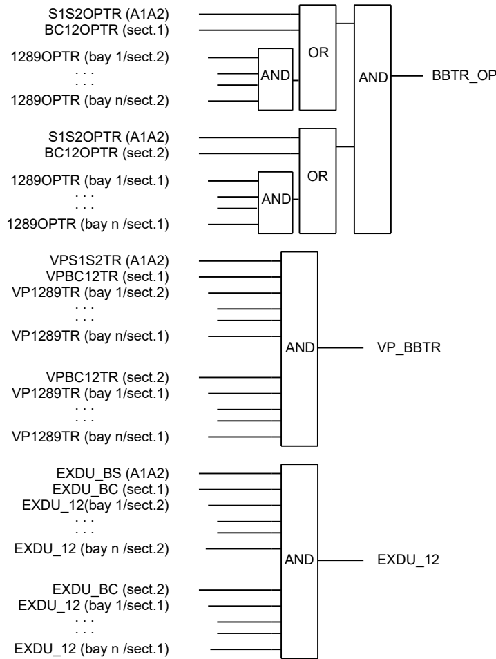
Figure 67: Signals from any bays for a bus-section circuit breaker between sections B1 and B2
