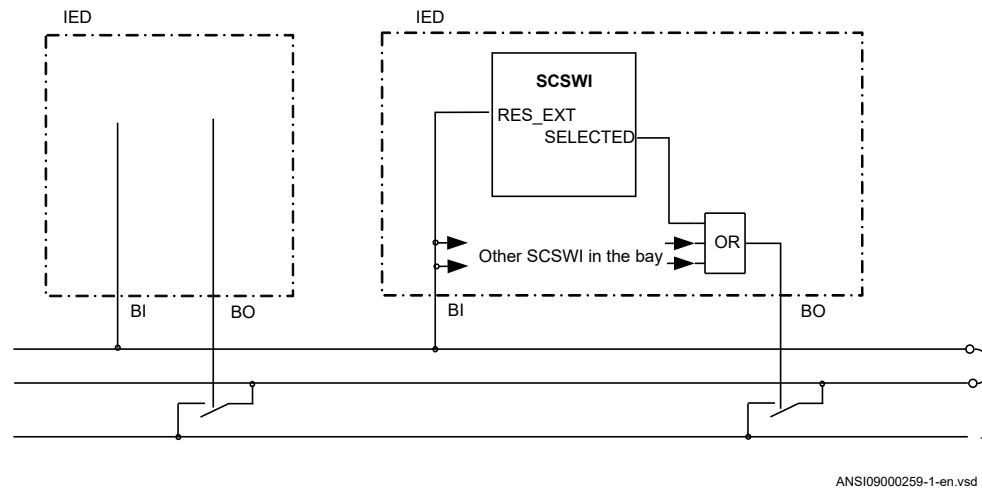
Figure 51: Application principles for reservation with external wiring
