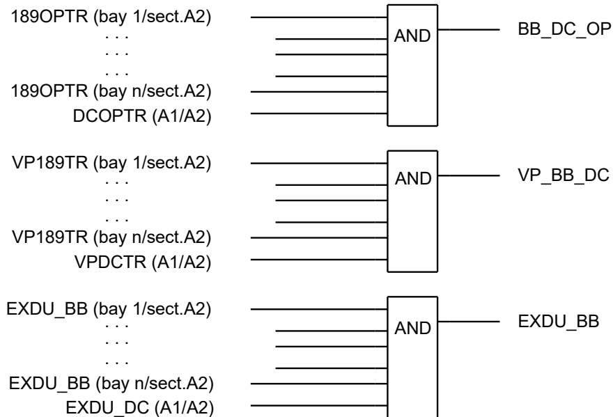
Figure 58: Signals from any bays in section A2 to a busbar grounding switch in the same section
