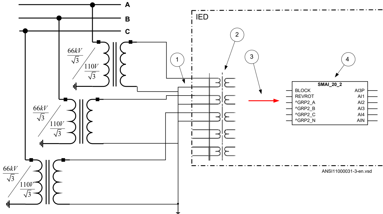
Figure 15: A Three phase-to-ground connected VT
