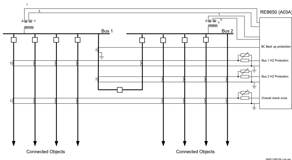
Figure 3: Two-section busbar in a High Voltage (HV) system
