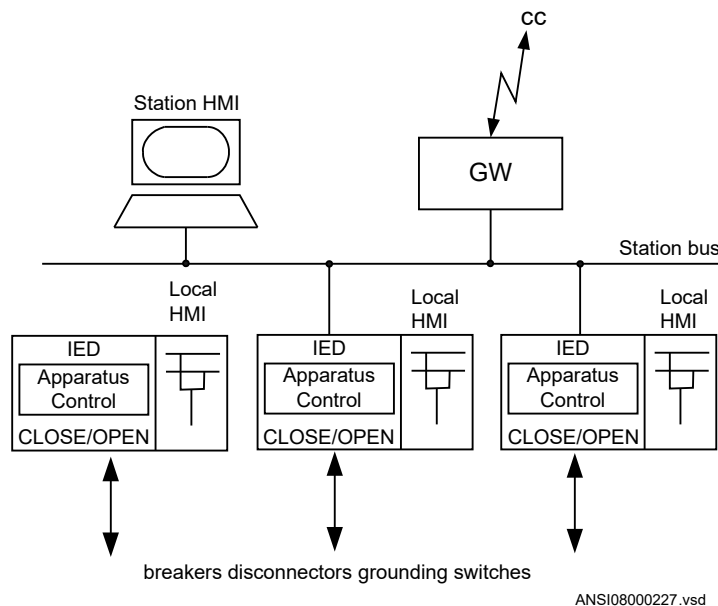
Figure 48: Overview of the apparatus control functions
