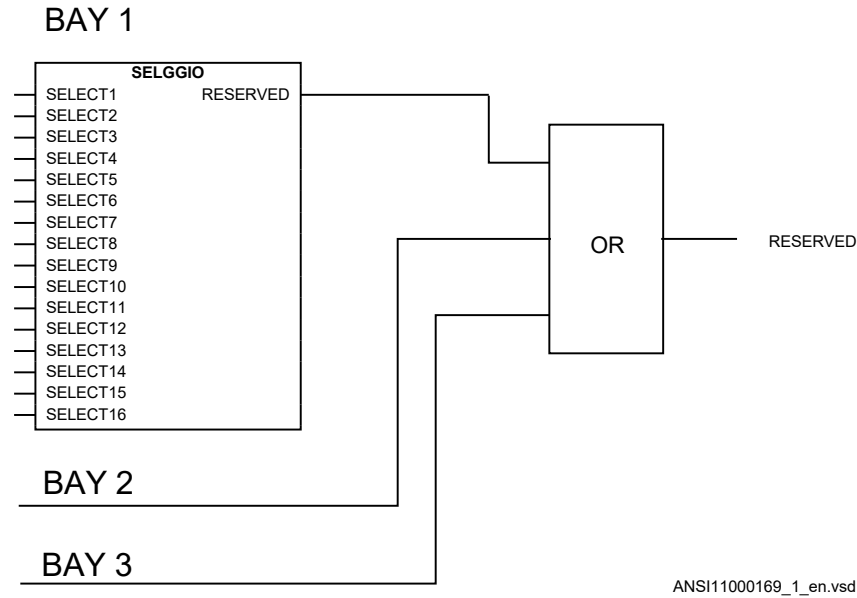
Figure 50: Reservations from own and other bays
