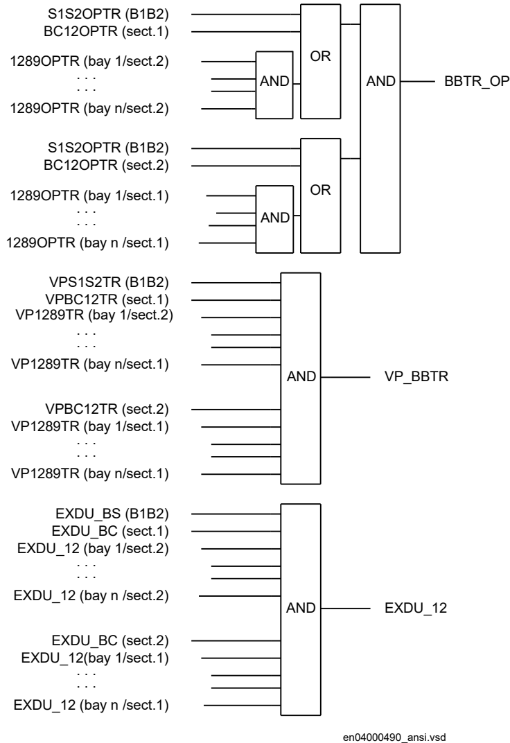
Figure 66: Signals from any bays for a bus-section circuit breaker between sections A1 and A2
