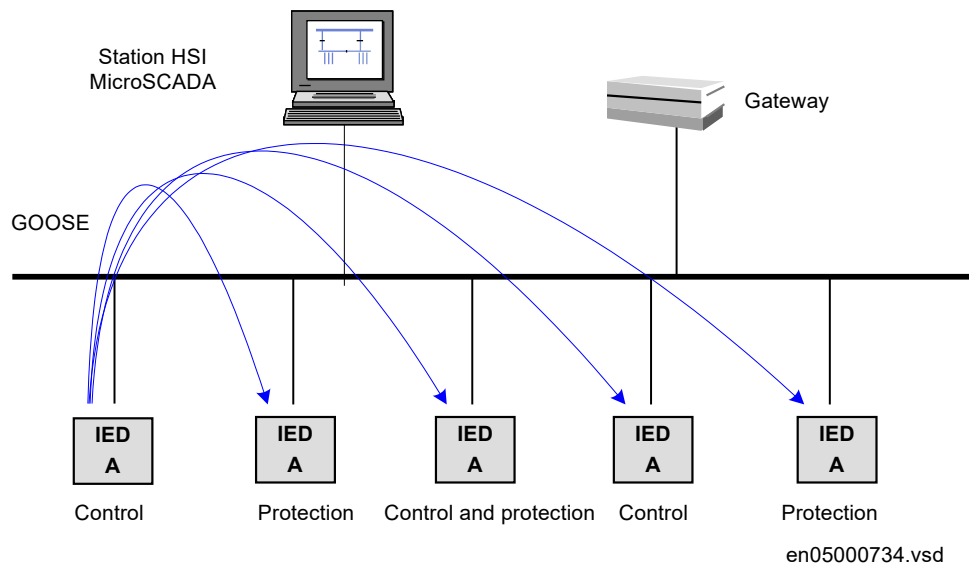
Figure 105: Example of a broadcasted GOOSE message
