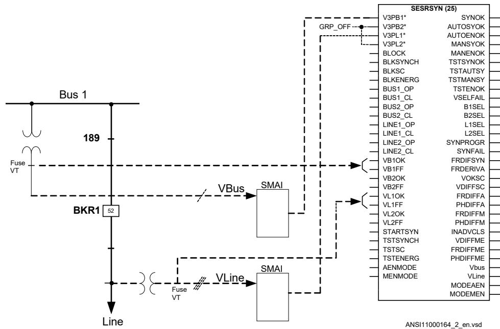
Figure 45: Connection of SESRSYN (25) function block in a single busbar arrangement
