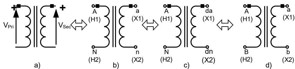
Figure 14: Commonly used markings of VT terminals
