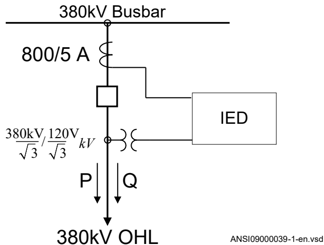
Figure 100: Single line diagram for 380kV OHL application
