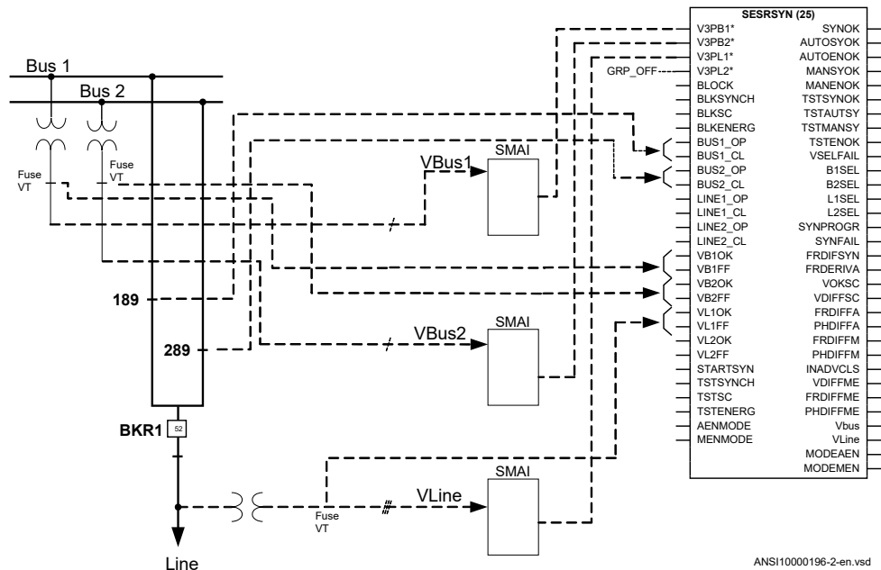
Figure 47: Connection of the SESRSYN (25) function block in a single breaker, double busbar arrangement with internal voltage selection.
