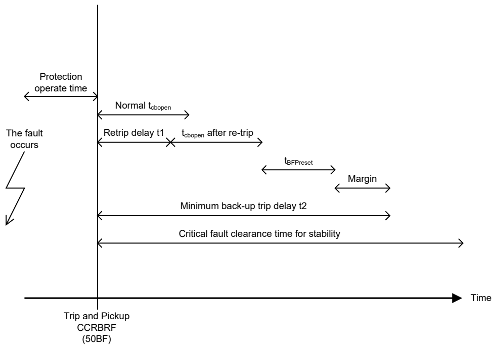
Figure 35: Time sequence
