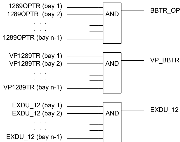
Figure 81: Signals from any bays in bus-coupler bay n
