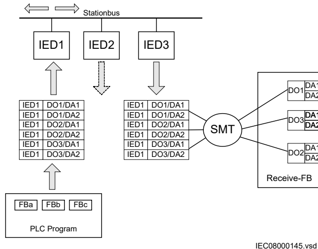
Figure 106: SMT: GOOSE principle and signal routing with SMT
