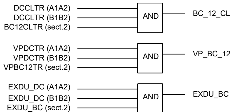
Figure 85: Signals to a bus-coupler bay in section 1 from a bus-coupler bay in another section
