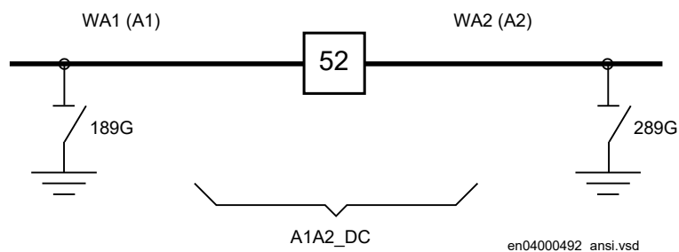
Figure 68: Switchyard layout A1A2_DC (3)
