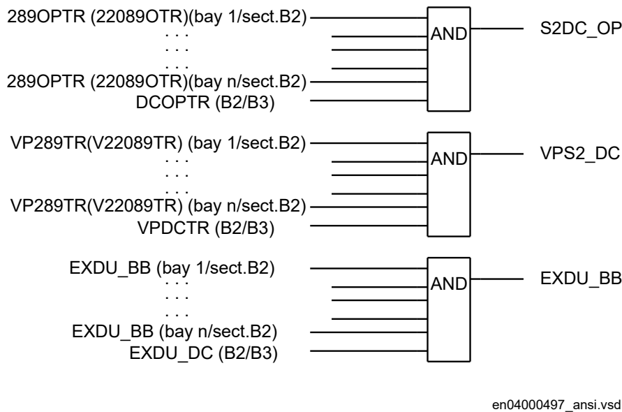
Figure 73: Signals from any bays in section B2 to a bus-section disconnecter
