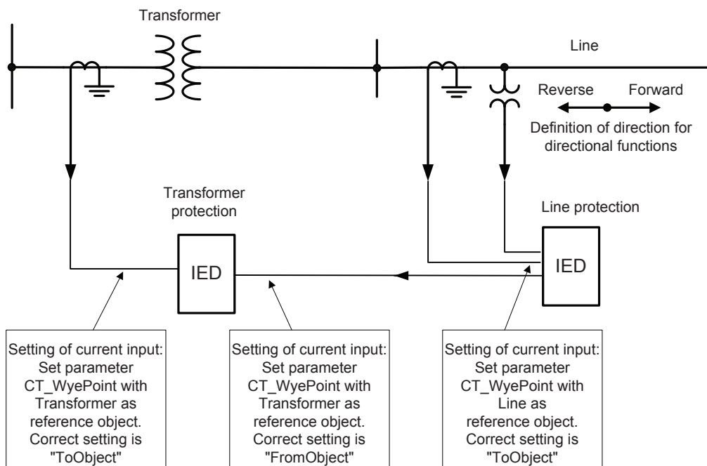
Figure 10: Example how to set CT_WyePoint parameters in the IED
