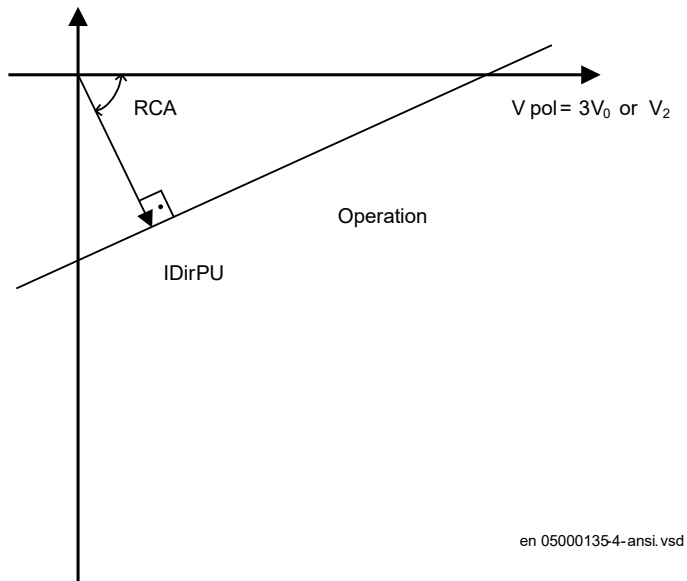
Figure 34: Relay characteristic angle given in degree
