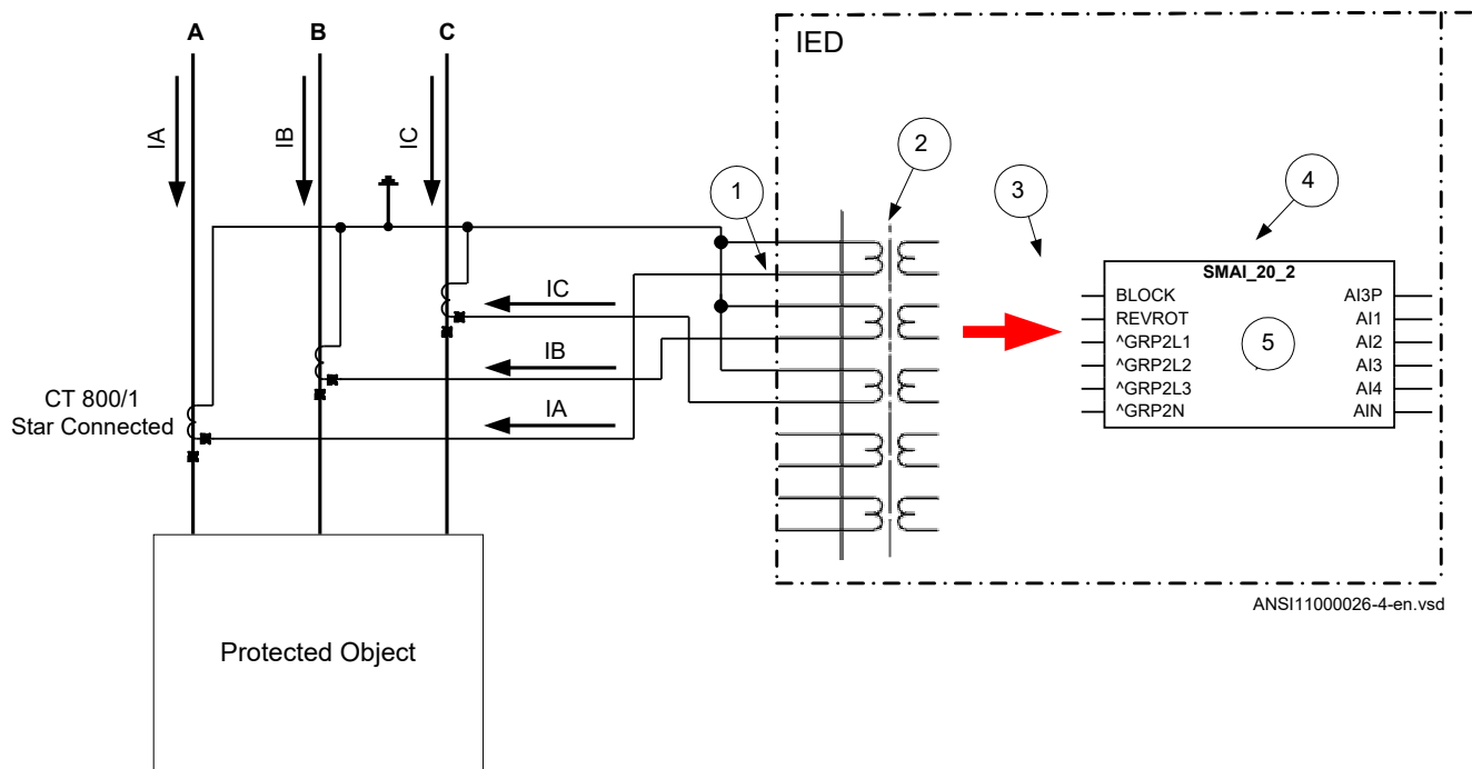
Figure 13: Wye connected three-phase CT set with its star point away from the protected object
