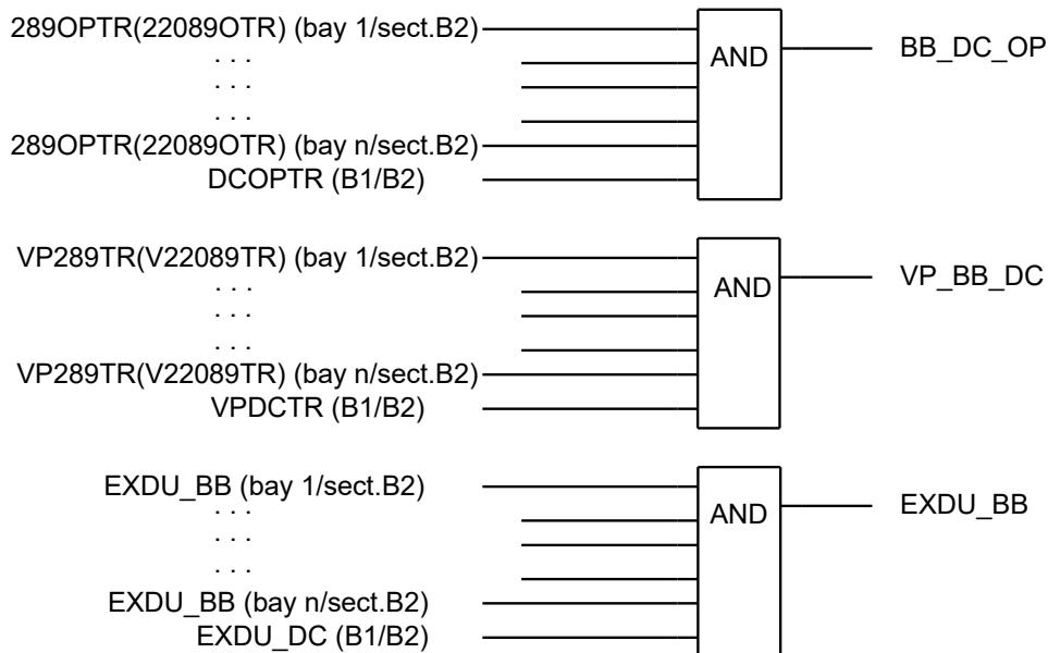
Figure 60: Signals from any bays in section B2 to a busbar grounding switch in the same section
