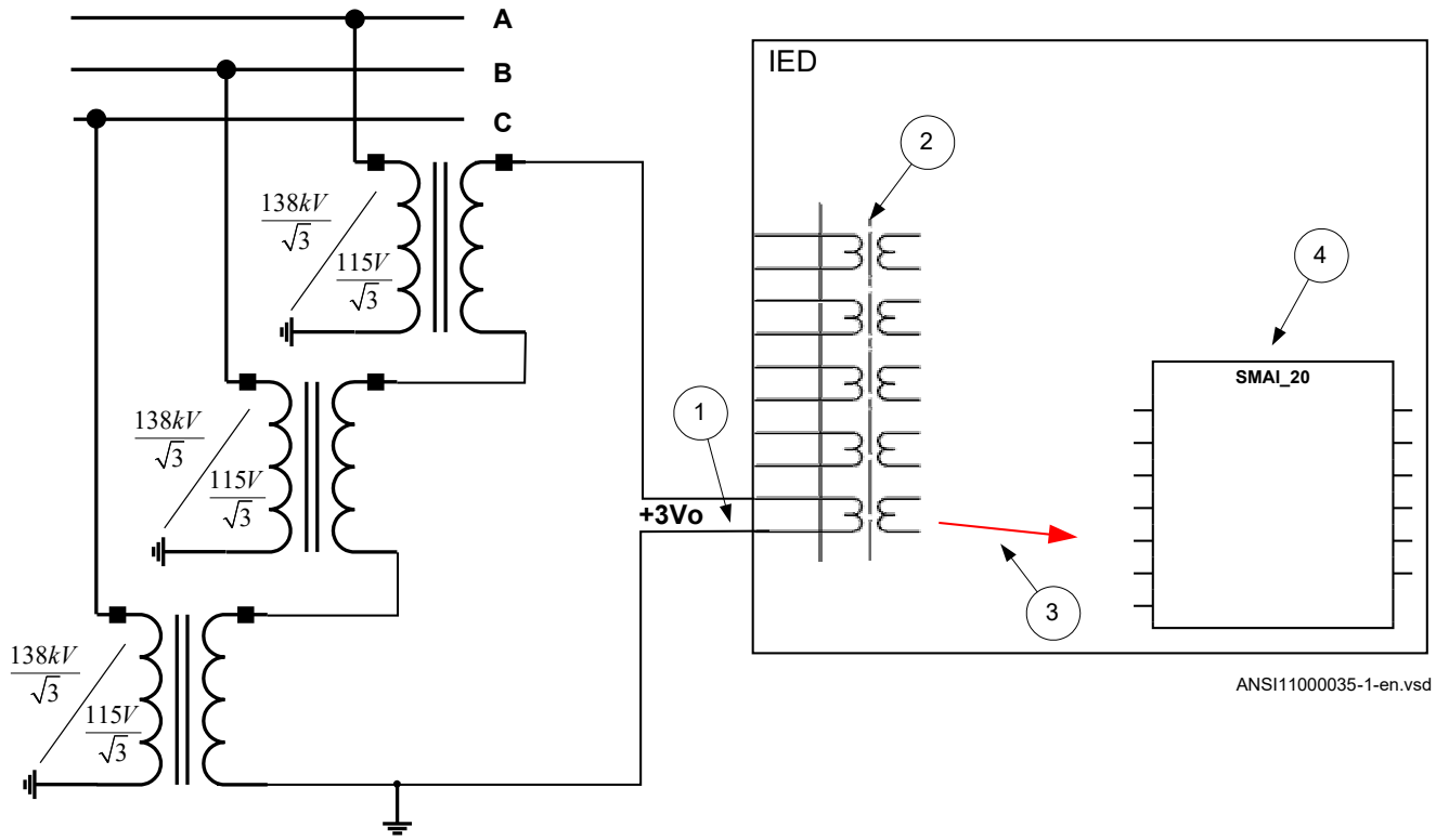
Figure 16: Open delta connected VT in low impedance or solidly grounded power system
