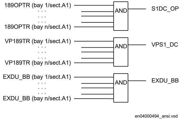
Figure 70: Signals from any bays in section A1 to a bus-section disconnecter
