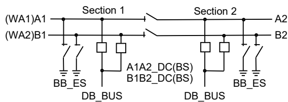
Figure 62: Busbars divided by bus-section disconnectors (circuit breakers)
