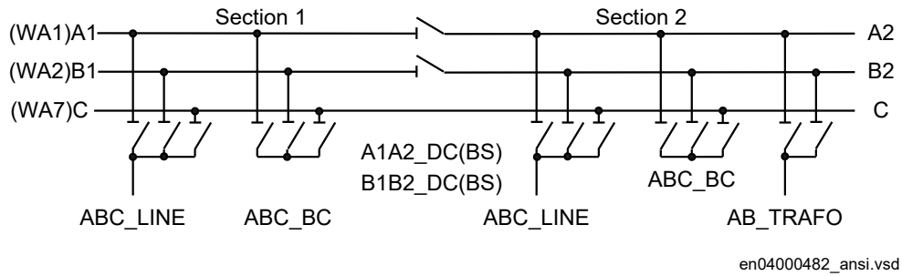
Figure 82: Busbars divided by bus-section disconnectors (circuit breakers)
