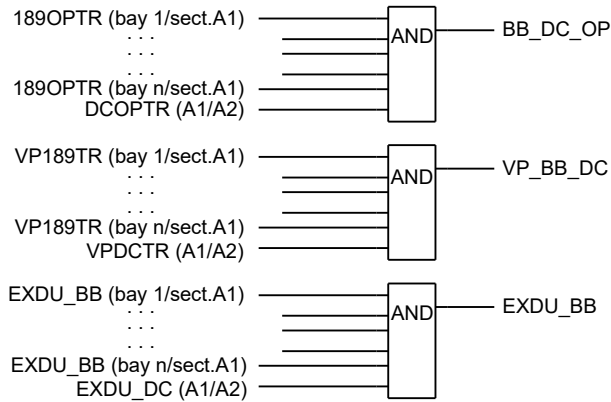
Figure 57: Signals from any bays in section A1 to a busbar grounding switch in the same section
