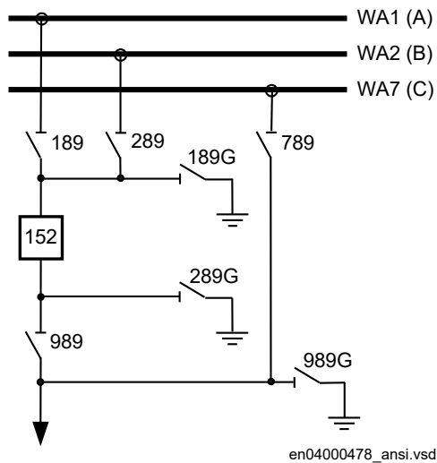
Figure 88: Switchyard layout ABC_LINE (3)
