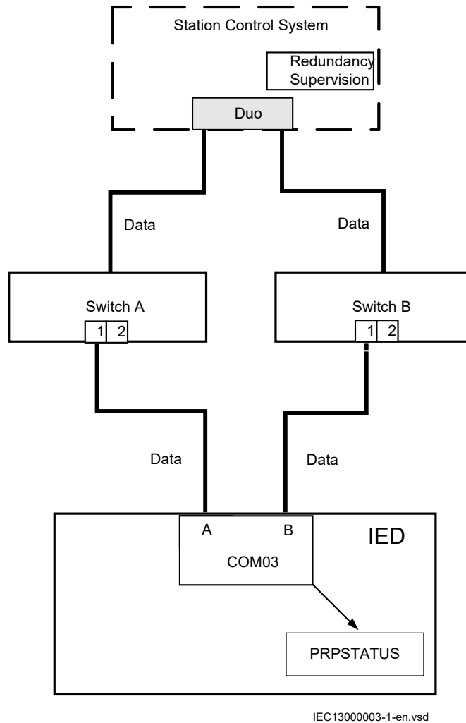
Figure 109: Redundant station bus
