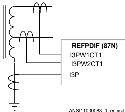
Figure 97: REFPDIF (87N) function inputs for autotransformer application
