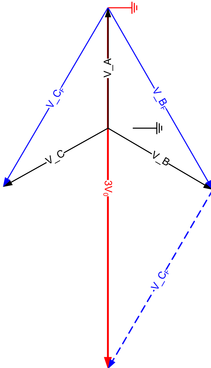
Figure 36: Ground fault in Non-effectively grounded systems
