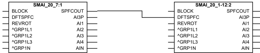
Figure 115: Configuration for using an instance in task time group 1 as DFT reference
