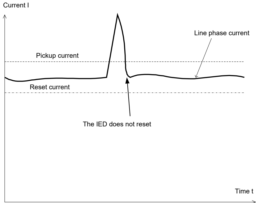
Figure 30: Pickup and reset current for an overcurrent protection
