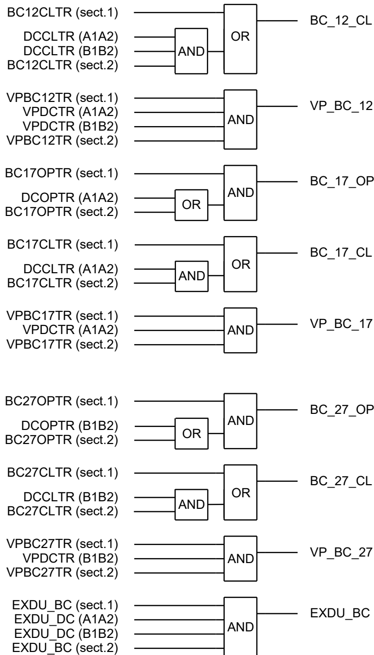
Figure 91: Signals to a line bay in section 1 from the bus-coupler bays in each section
