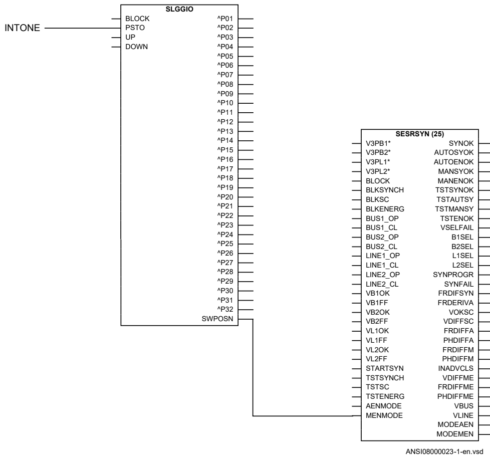
Figure 44: Selection of the energizing direction from a local HMI symbol through a selector switch function block.
