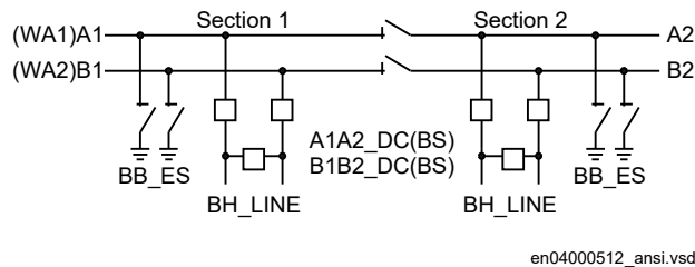
Figure 63: Busbars divided by bus-section disconnectors (circuit breakers)
