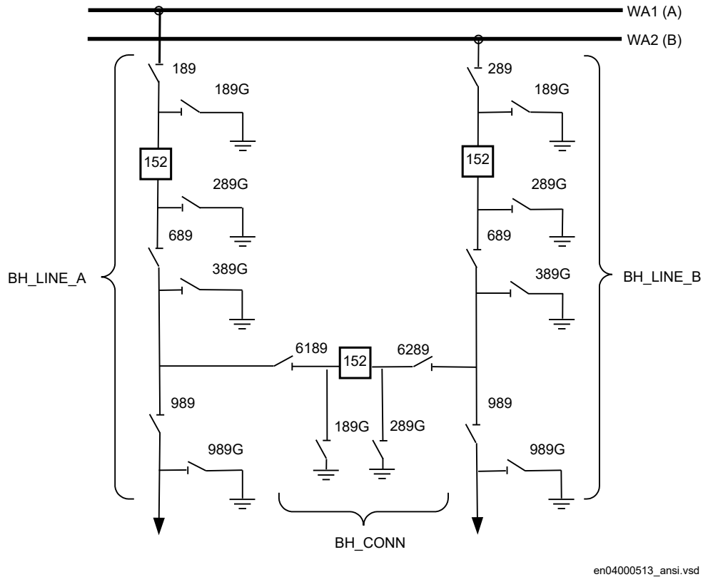
Figure 86: Switchyard layout breaker-and-a-half
