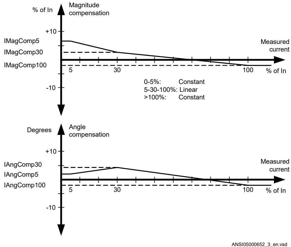
Figure 99: Calibration curves
