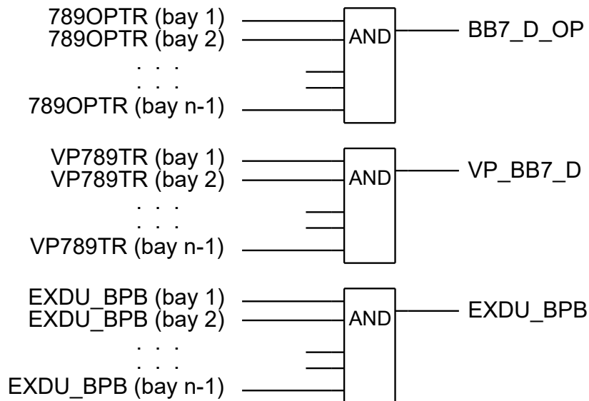
Figure 89: Signals from bypass busbar in line bay n
