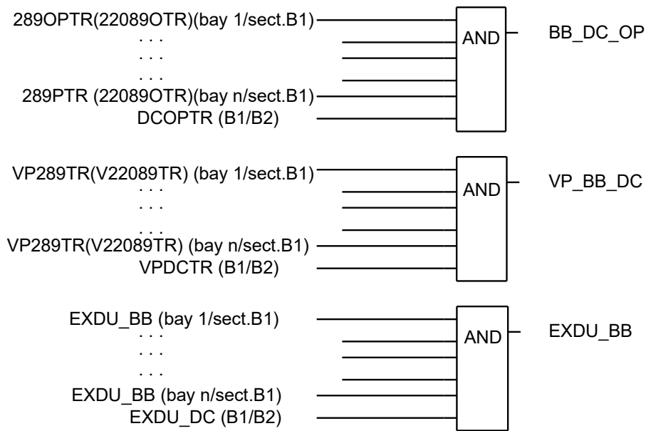
Figure 59: Signals from any bays in section B1 to a busbar grounding switch in the same section
