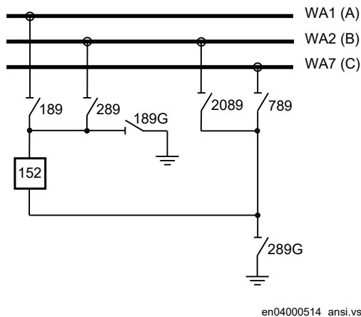
Figure 80: Switchyard layout ABC_BC (3)
