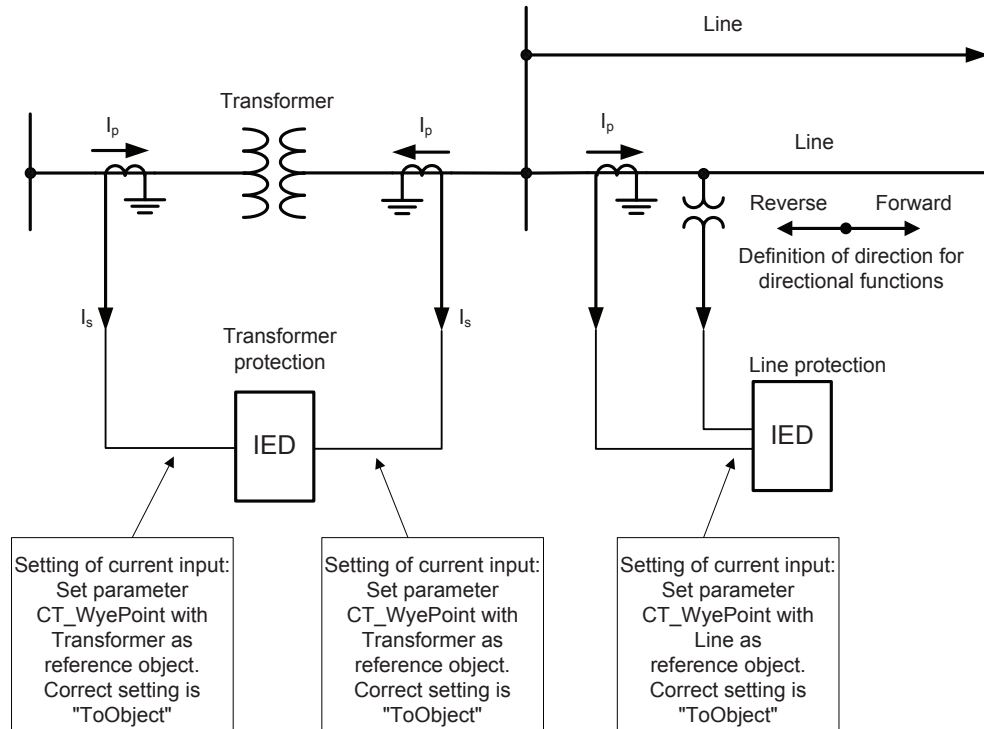
Figure 9: Example how to set CT_WyePoint parameters in the IED
