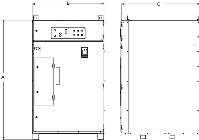
ZBTS T-series dimensions
