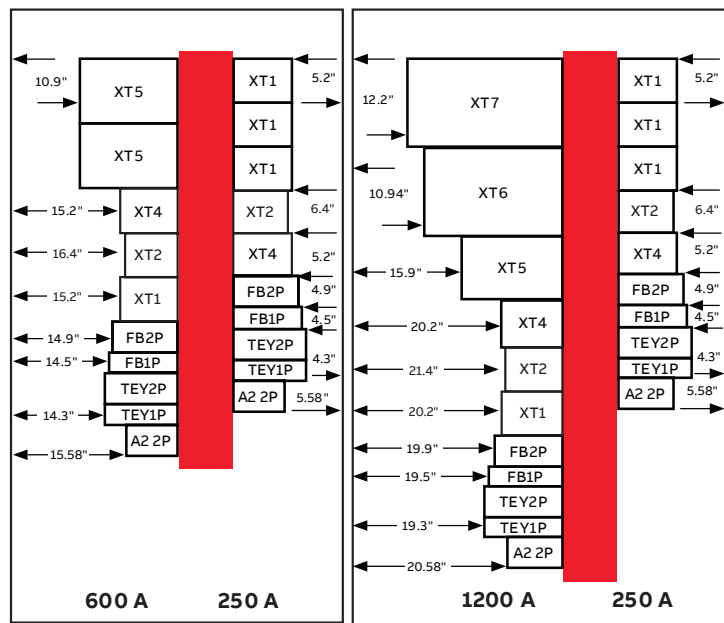
40" offset box
