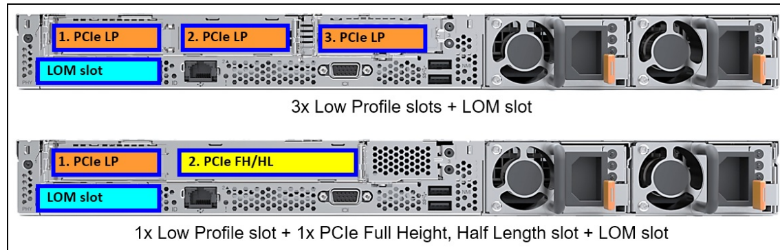
Figure 4. Slot locations
