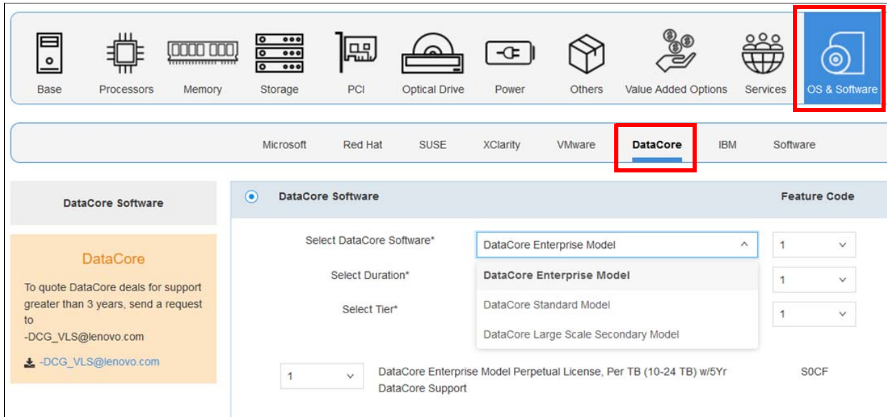
Figure 17 DataCore software
