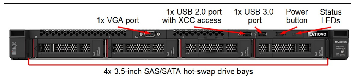
Figure 2. HX1320 front view
