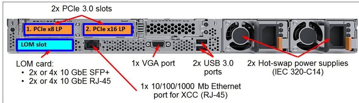
Figure 3. HX1320 rear view
