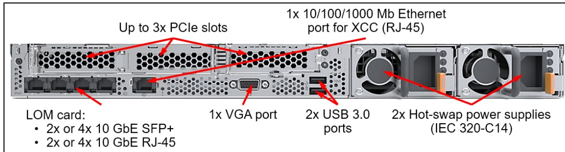
Figure 3. VX3320 rear view
