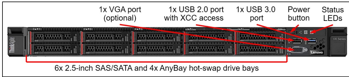
Figure 2. VX3320 front view
