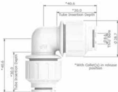
800-02202 JG WATERMARK EQUAL ELBOW 12MM PEMO312W
