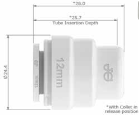
800-02216 JG WATERMARK END CAP 12MM PSE4612W
