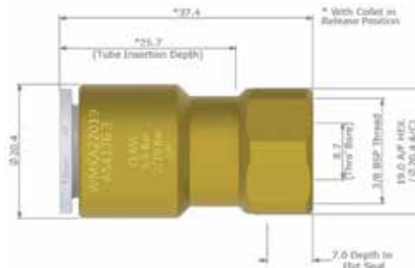
800-02220 JG WATERMARK FEMALE ADAPTOR 12MM MW451213 3/8 BSP
