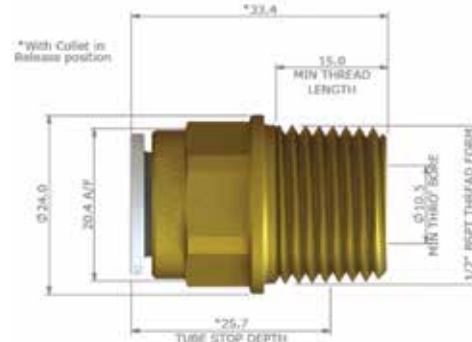
800-02218 JG WATERMARK MALE ADAPTOR 12MM NC2771 1/2 BSPT Ideal for use with Suburban HWS
