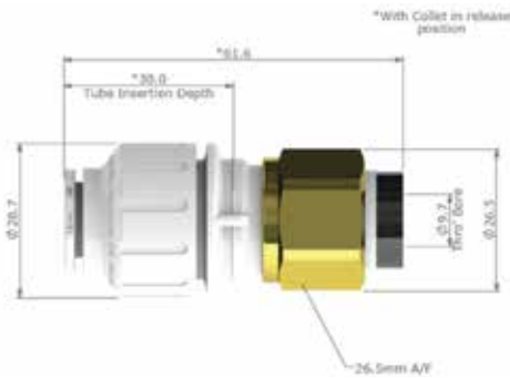
800-02212 JG WATERMARK STRAIGHT TAP CONNECTOR 12MM PEMSTC1214 1/2 BSP
