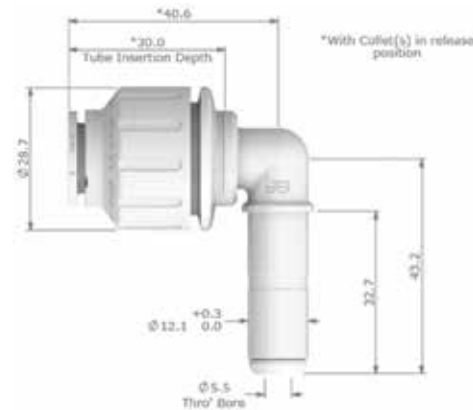
800-02206 JG WATERMARK STEM ELBOW 12MM PEM221212W
