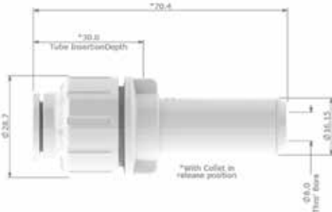
800-02212 JG WATERMARK STRAIGHT TAP CONNECTOR 12MM PEMSTC1214 1/2 BSP
