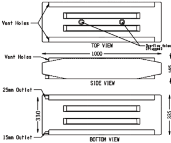
800-01520 ROUND ENDED TANK 61L round ended tank
