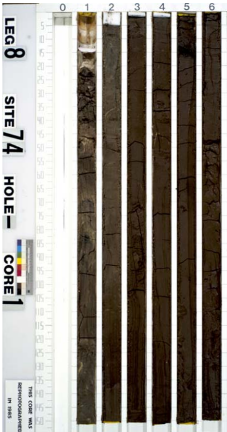
Core 8-74-1R
