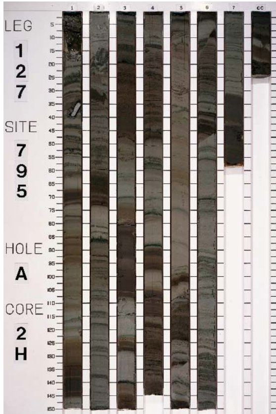
Core 127-795A-2H
