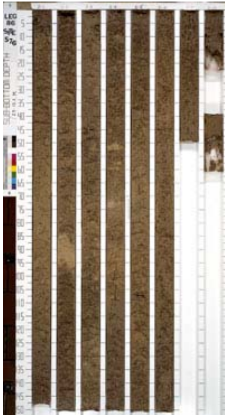
Core 86-576-2
