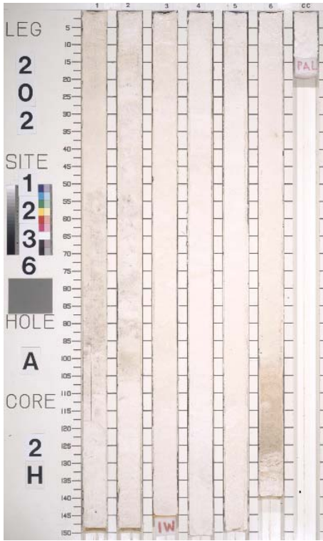
Core 202-1236A-2H
