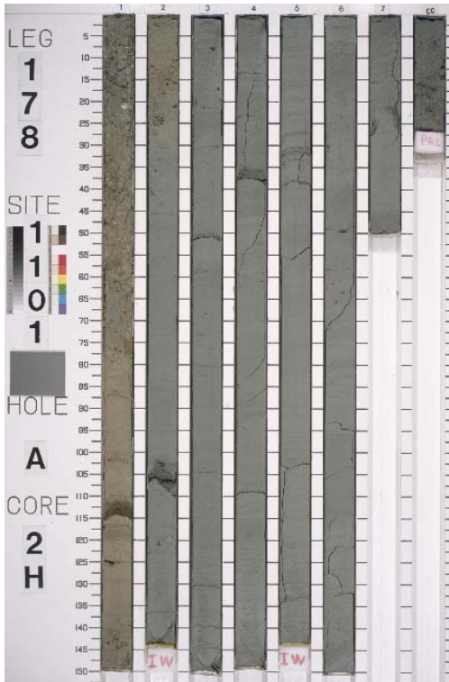
Core 178-1101A-2H
