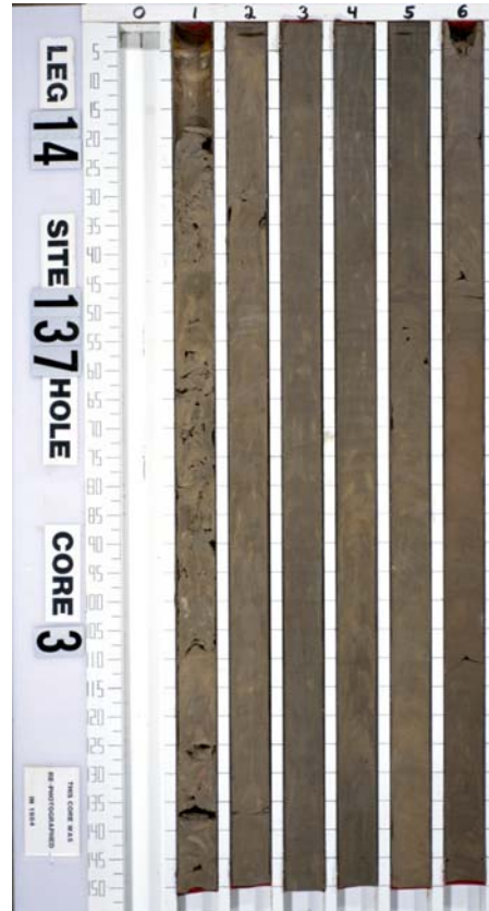
Core 14-137-3R
