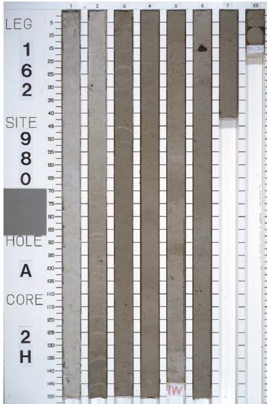
Core 162-980A-2H
