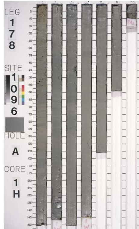
Core 178-1096A-1H
