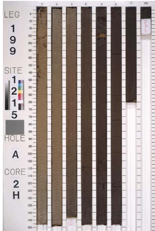
Core 199-1215A-2H
