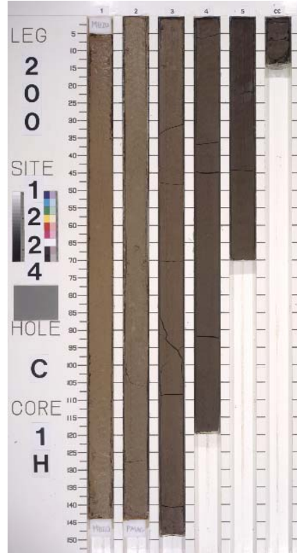
Core 200-1224C-1H
