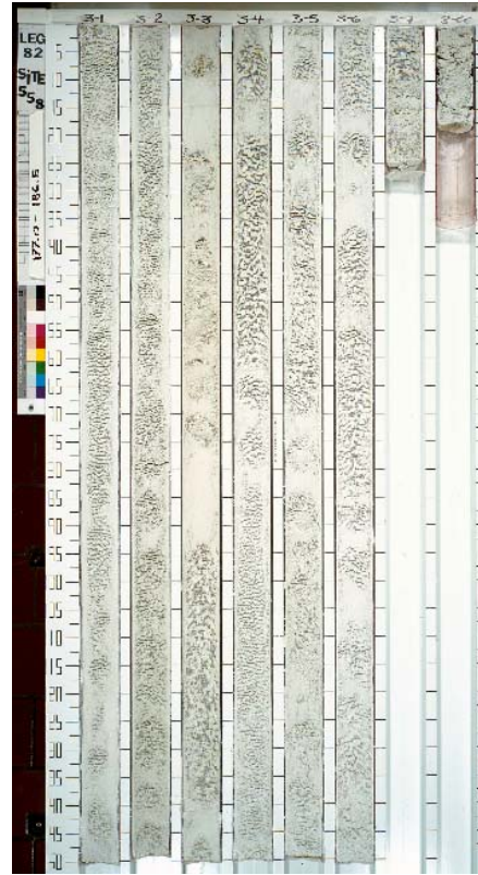
Core 82-558-3
