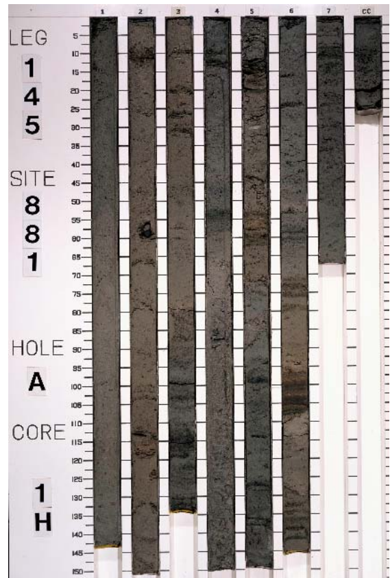
Core 145-881A-1H
