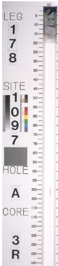
Core 178-1097A-3R
