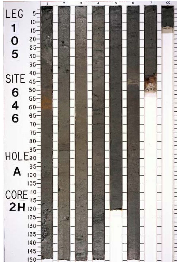
Core 105-646A-2H
