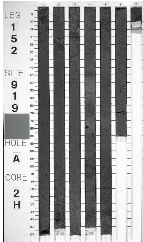
Core 152-919A-2H
