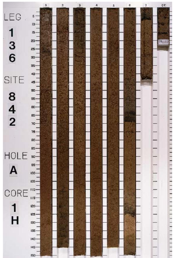
Core 136-842A-1H
