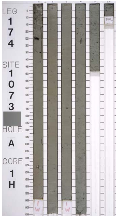
Core 174-1073A-1H
