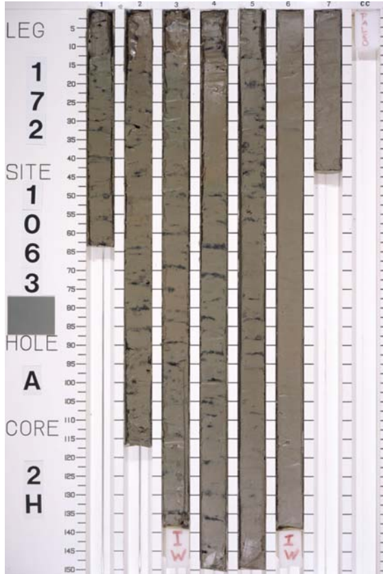
Core 172-1063A-2H
