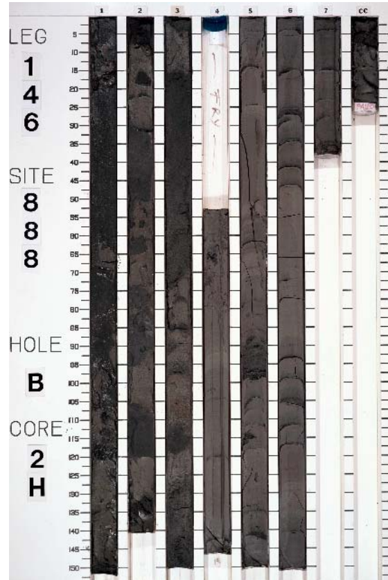
Core 146-888B-2H
