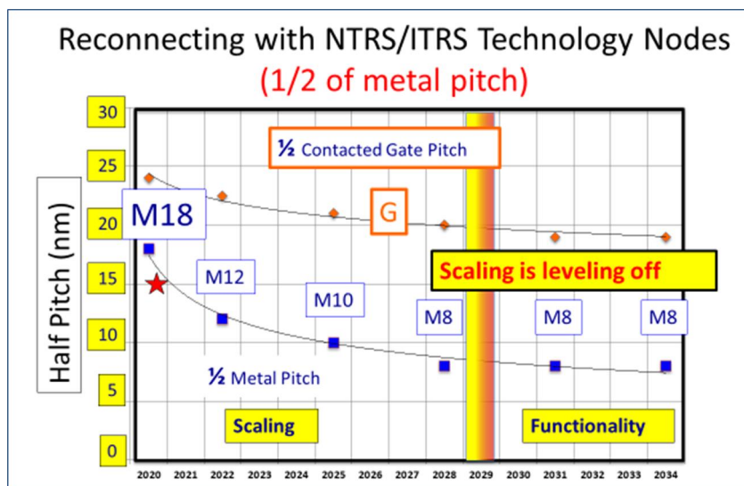
Figure ES8 Metal pitch scaling exceeding expectation in 2020!
