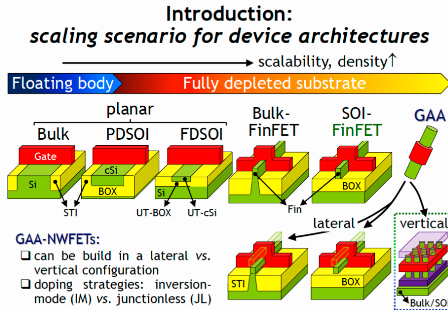
Figure ES47 Practical migration of transistor structure from FinFET to GAA to fully vertical
