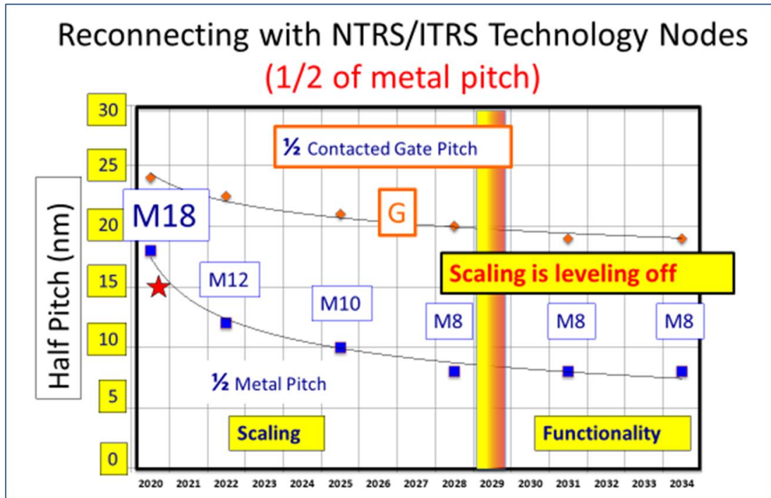
Figure ES31 Metal pitch scaling exceeding expectation in 2020!
