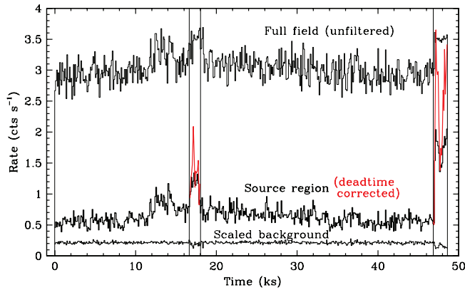
FIG. 8.— Light curves of the HRC observation, with 100 s binning. Zero time corresponds to the beginning of the observation on 2007 May 28 at 4:19:18 UT. Thin vertical lines mark flare intervals, and the red traces within those intervals denote event rates after approximate corrections for dead time due to telemetry saturation. The lowest curve is from the background region in Fig. 3 and is scaled for the area of the source region. The microflaring analysis excludes the large flare at the end (after time = 46,842 s). Exclusion of the small flare between times 16,642 and 18,042 s has little effect on the analysis.
