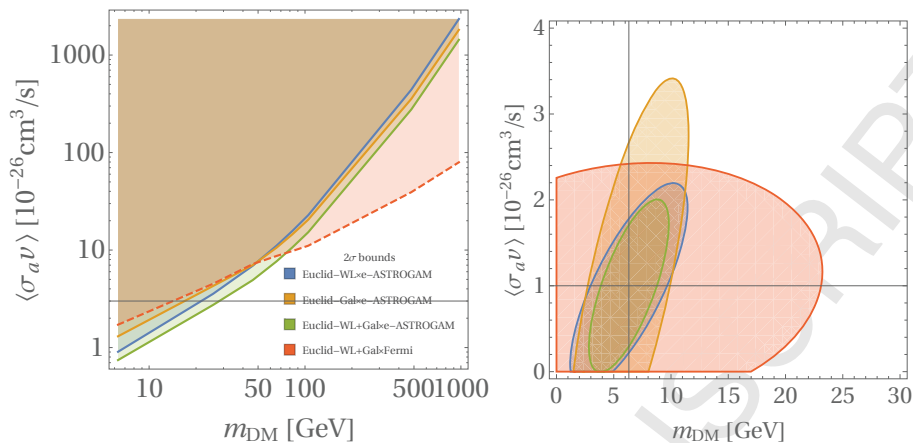
Figure 4.10.1: Left panel: Expected 2\sigma bounds on the DM annihilation cross section, \langle \sigma_a v \rangle , versus its mass for a DM candidate annihilating into bottom quarks. The blue line is derived for the cross-correlation of e-ASTROGAM with Euclid weak-lensing cosmic shear, the yellow instead considers the Euclid galaxy clustering, and green line is their combination. The dashed red line shows the bound expected with Euclid data (weak lensing together with galaxy clustering) combined with Fermi-LAT 10 year data dating Right panel : Expected 1\sigma joint marginal error contours on WIMP parameters for e-ASTROGAM gamma-ray data cross-correlated with Euclid (same colour code as in left panel). We chose a WIMP candidate with fiducial DM mass of \sim 6 GeV and \langle \sigma_a v \rangle = 10^{-26} \text{cm}^3/\text{s} .
