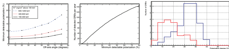
Figure 2.3.2: Left: Minimum polarization fraction detectable by e-ASTROGAM in three energy bands as a function of the off-axis angle. Centre: Cumulative number of GRBs to be detected by e-ASTROGAM as a function of the MDP. Right: Expected measured distribution of polarization degrees achieved using 1 year of data for the photospheric emission model (red) and the synchrotron with highly ordered magnetic field model (blue).
