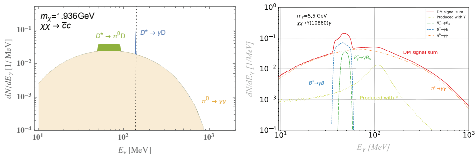
Figure 4.4.1: Left: Example of the expected gamma-ray spectrum for DM annihilation into charm quarks, with a DM mass m_\chi just above the kinematic threshold to produce D -mesons. The sharp spectral features result from the indicated meson transitions, while the background is mostly due to \pi^0 \rightarrow \gamma\gamma . For more details, see Ref. [416]. Right: Gamma-ray spectrum from DM annihilation through the quarkonium channel \chi\chi \rightarrow \Upsilon(10860)\gamma . The three visible spectral features are due to two different meson transitions and the photon produced in conjunction with the quarkonium. For more details, see Ref. [425].
