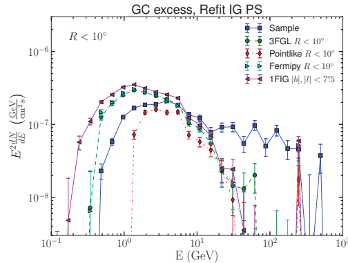
Figure 8.3.1: Effect on the spectrum of the GC excess from refitting of PS near the GC [833].
