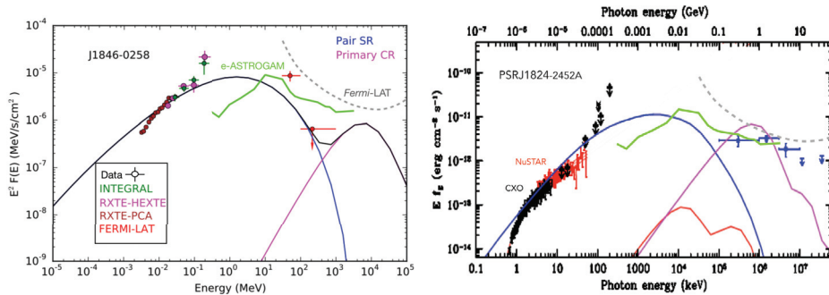
Figure 6.4.2: SEDs of the young pulsar J1846-0258 (left) and of the millisecond pulsar J1824-2452A (right). The model curves show the expected curvature radiation (magenta) and synchrotron radiation (red) from the primary particles accelerated in the current sheet, and the synchrotron radiation (blue) from the secondary pairs produced in cascades and radiating in the open magnetosphere. Adapted from [664], [667] and [668], with J1846-0258 data from [615] and [666]. The sensitivities of e-ASTROGAM (solid green) and of Fermi -LAT (dashed gray) are given for one year of effective exposure in the Galactic disk.
