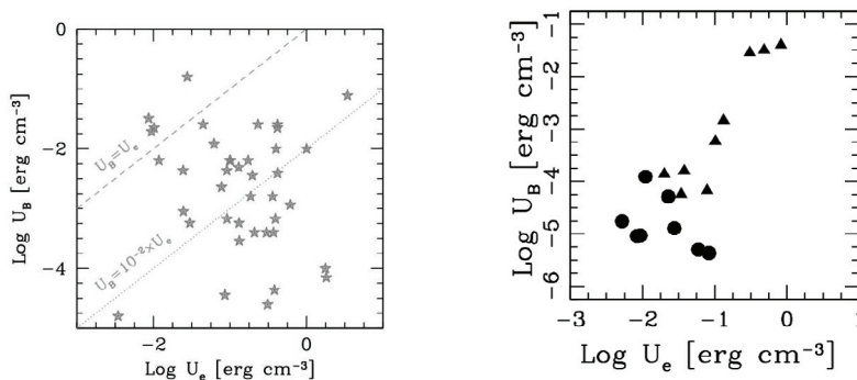
Figure 2.13.1: Left: Magnetic energy density and relativistic electron density estimated from SEDs of 45 BL Lac objects [240]. Right: Same, for Mrk 421 (triangles) and Mrk 501 (circles) in different activity states [241].
