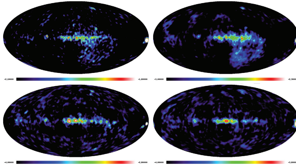
Figure 8.1.1: COMPTTEL all-sky images using the current Maximum Entropy implementation. Galactic coordinates, centred on l = 0 , b = 0 . Left to right, top to bottom: 1-3 MeV, 3-10 MeV, 10-30 MeV, 1.8 MeV ^{26}\text{Al} line.
