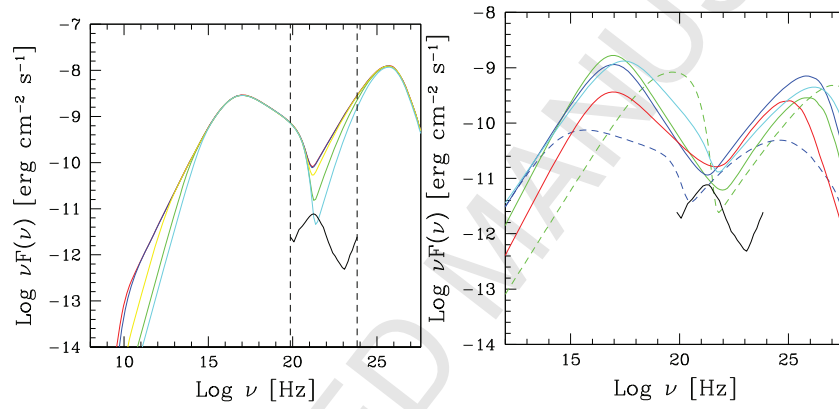
Figure 2.13.3: Left: SSC emission models produced by varying \gamma_{\min} , while keeping other emission parameters as constant. Red ( \gamma_{\min}=1 ), blue ( \gamma_{\min}=100 ), yellow ( \gamma_{\min}=1000 ), green ( \gamma_{\min}=5000 ), and cyan ( \gamma_{\min}=10000 ) model curves show a significant difference at the e-ASTROGAM range (dashed vertical lines), and the radio region (where the emission from the extended region dominate). The black line corresponds to the sensitivity of e-ASTROGAM. Right: SSC model curves considering the SEDs of Mrk 501 (continuous line [241]) and Mrk 421 (dotted line [244]), which can be detected by e-ASTROGAM. The different colors indicate different activity levels.
