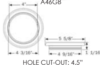
HOLE CUT-OUT: 4.5"
