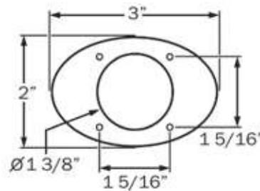
HOLE CUT-OUT: 1.375"
