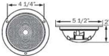
HOLE CUT-OUT: 4.5"
