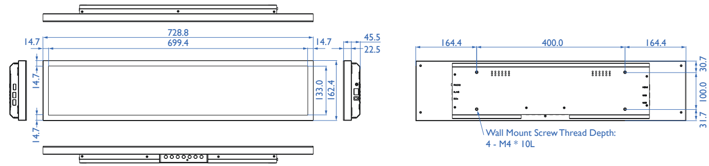
BH350I
