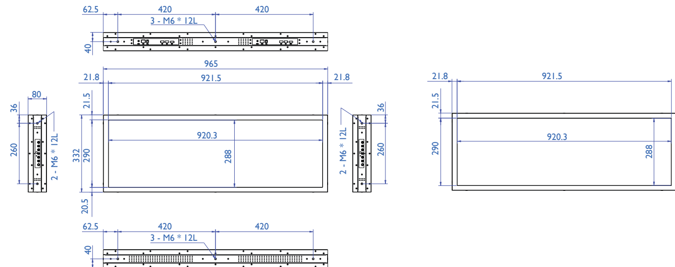
BH380ID
