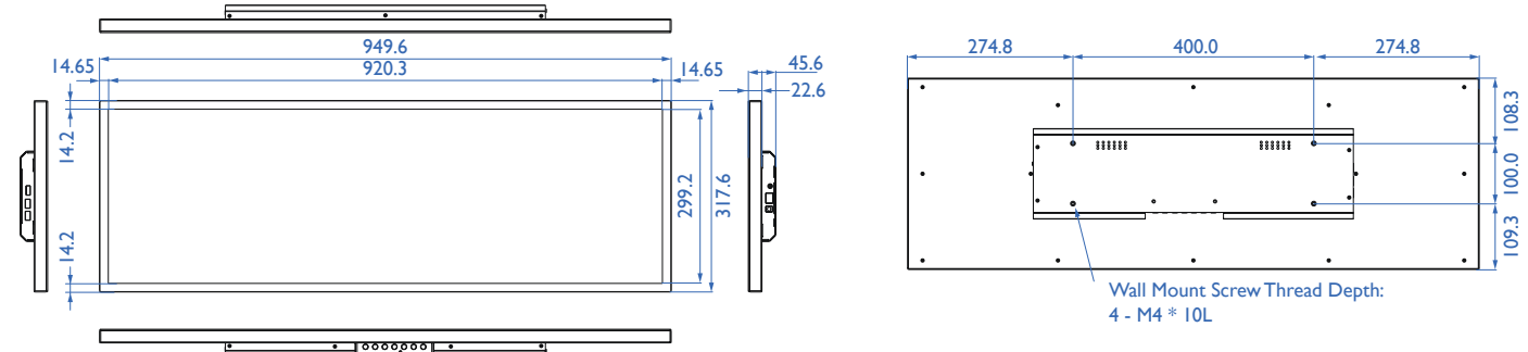
BH380ID
