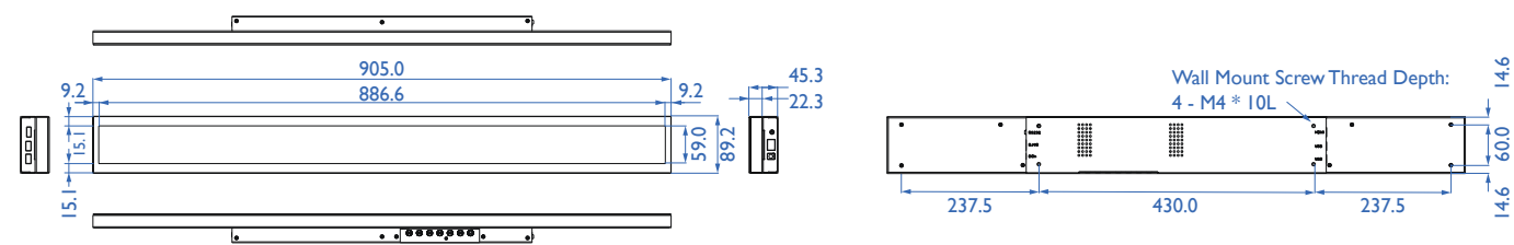
BH380I
