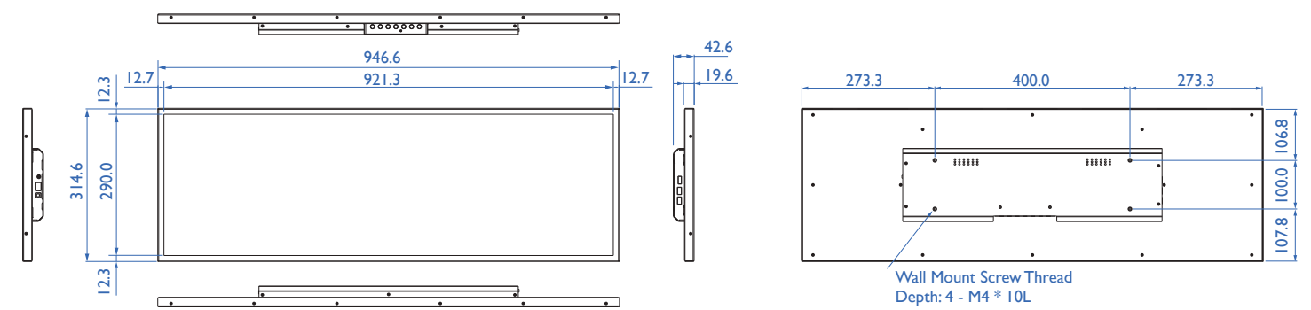
BH380IN
