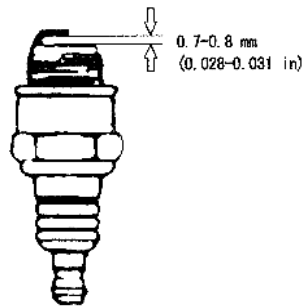
Figure 2 6- Measuring the spark plug gap
