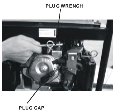
Figure 25- Removing the spark plug
