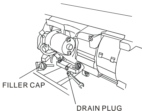
Figure 21- Draining oil
