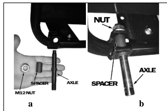
Figure 5 - axle assembly
