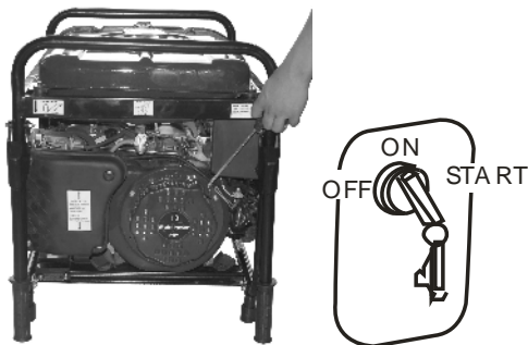
Figure 12- Start the generator
