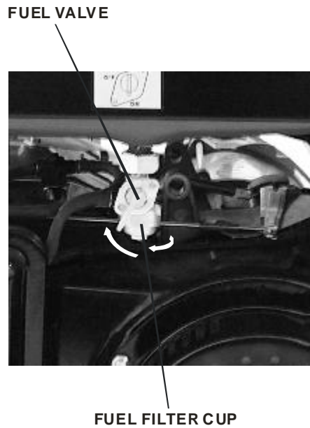
Figure 24- Removing the Fuel Filter Cup
