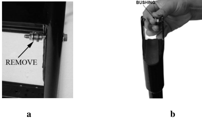
Figure 3- handle assembly
