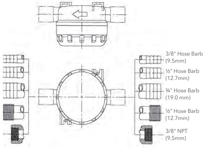
Inlet Strainer (Plugs into Quad pump port)
