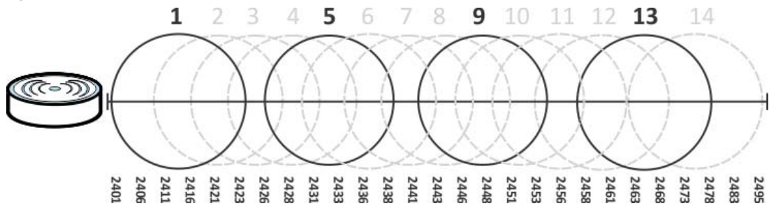
Figure 117 An Alternative Four-Channel Deployment
