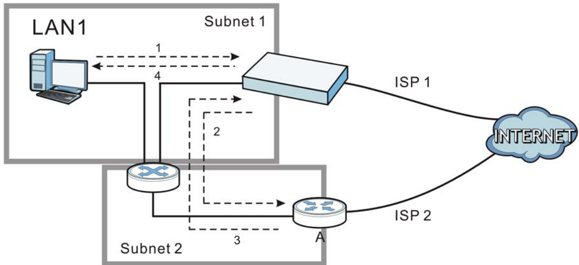
Figure 214 Using Virtual Interfaces to Avoid Asymmetrical Routes
