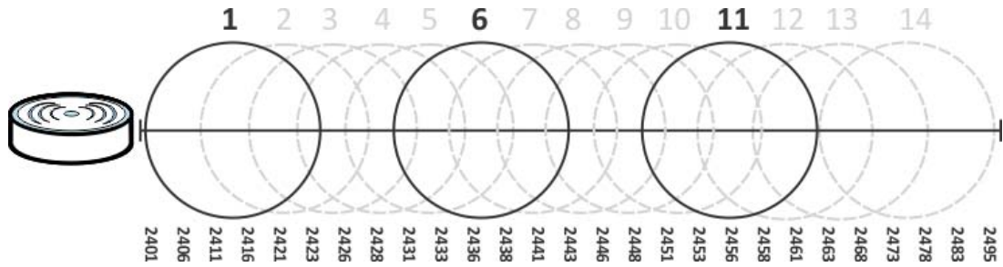
Figure 115 An Example Three-Channel Deployment
