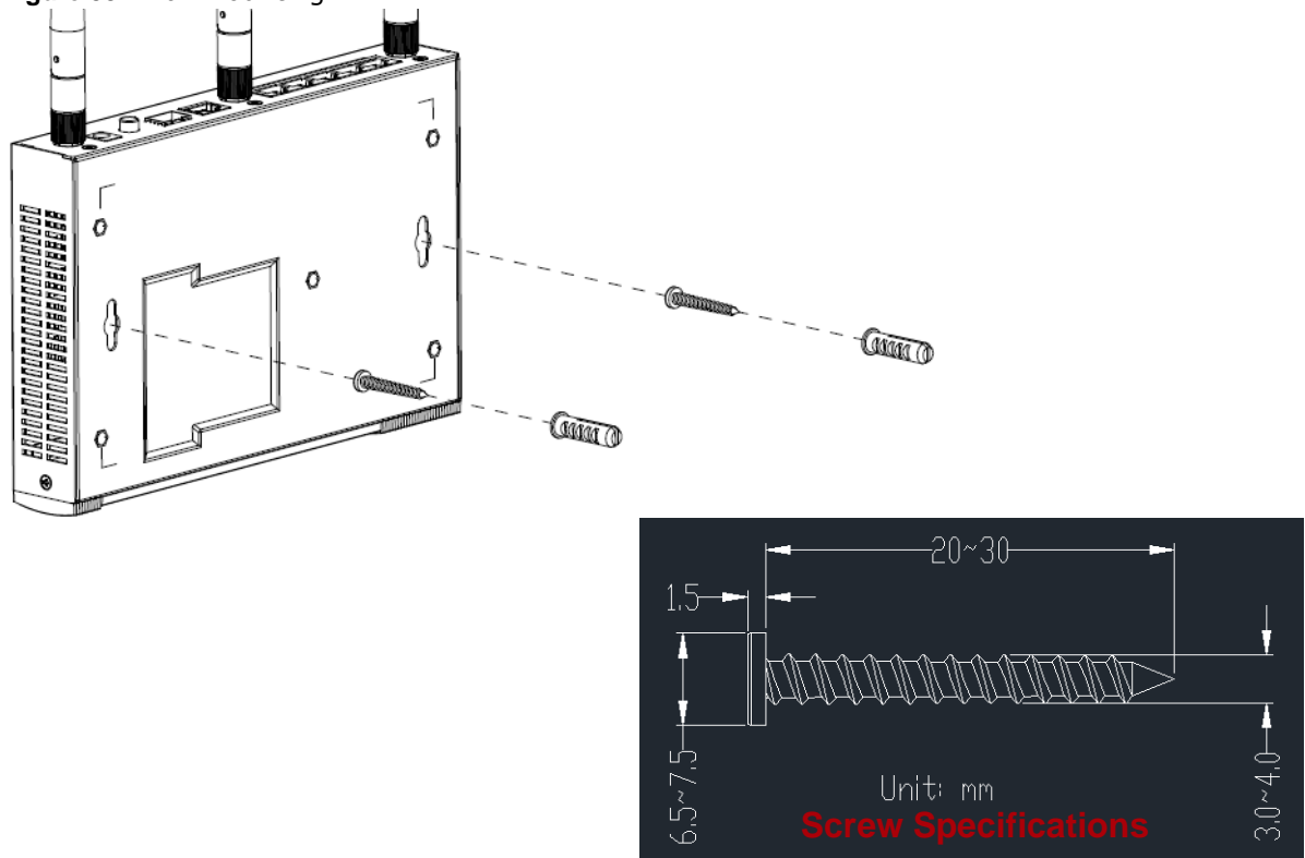
Figure 35 Wall Mounting
