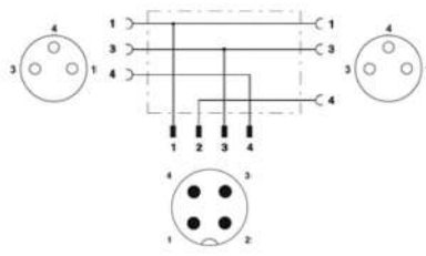
M12 to M8 Cable Splitter - Pin Out TA04XXMIEKC03000 (Male to Female View)
