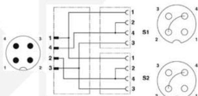
M12 to M12 Cable Splitter - Pin Out TA04XXMIEJC04000 (Male to Female View)
