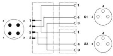
M12 to M8 Cable Splitter - Pin Out TA04XXMIEKC03000 (Male to Female View)
