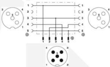
M12 to M12 Cable Splitter - Pin Out TA04XXMIEJC04000 (Male to Female View)
