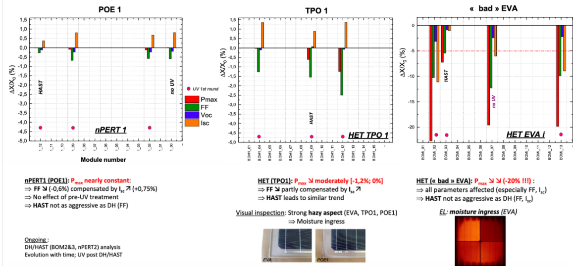
Figure 38: Assessment of heterojunction and nPERT modules with different encapsulants, following the modified indoor testing procedure (Source [109]).
