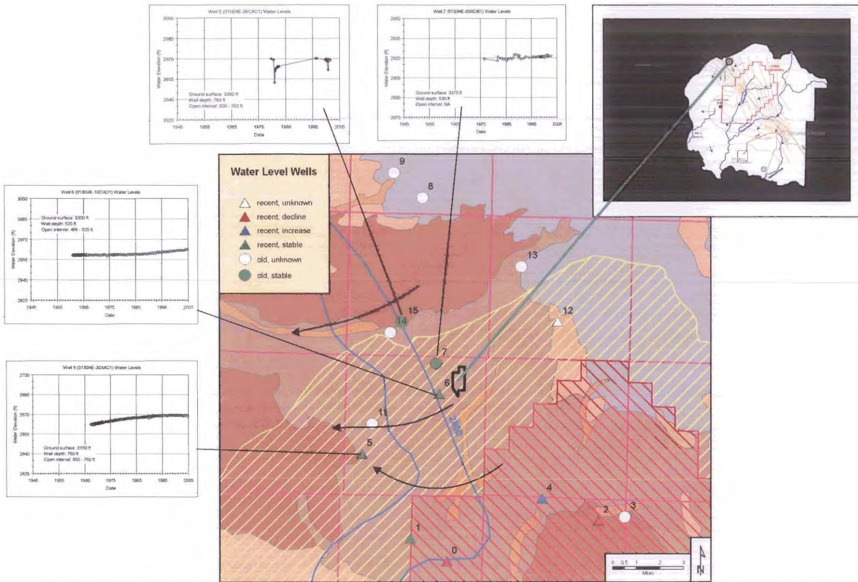
Figure 5. Mountain Home GWMA and Cinder Cone Butte CGWA boundaries with IDWR water level monitoring sites and hydrographs (Bendixsen, 1994). Arrows show general groundwater flow directions. Groundwater elevation contours in inset from Harrington, 2004.
