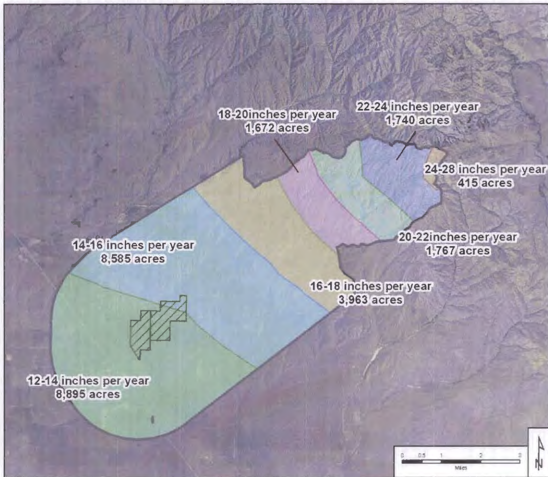
Figure 3. Annual precipitation rates in the project area.
