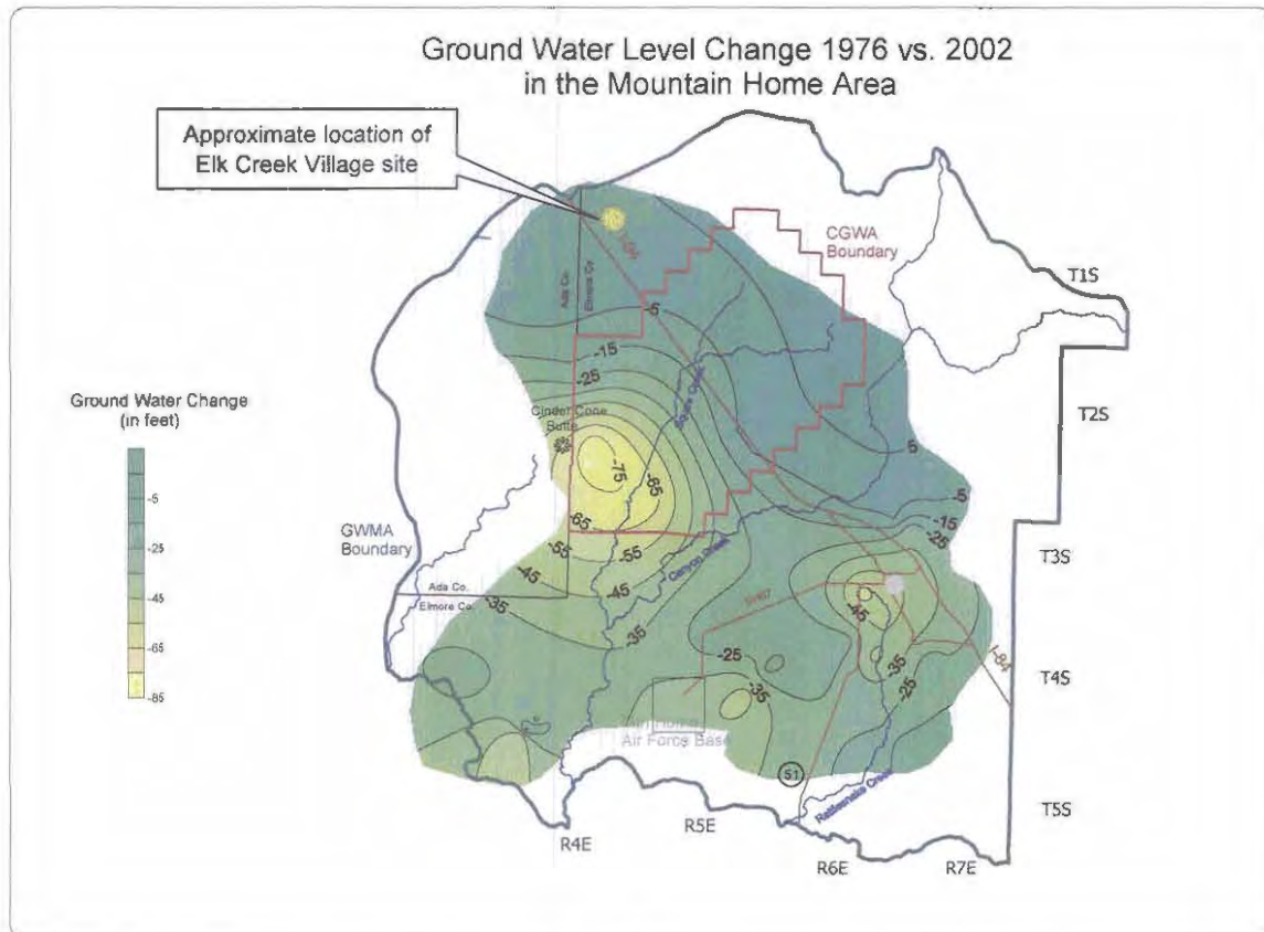
Figure 6. Water level changes measured by IDWR, 1976 to 2002 (from Harrington, 2004).
