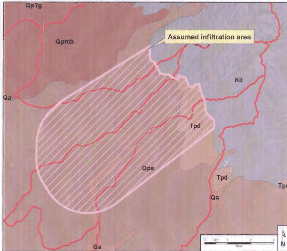
Figure 4. Precipitation infiltration area in the vicinity of the property.
