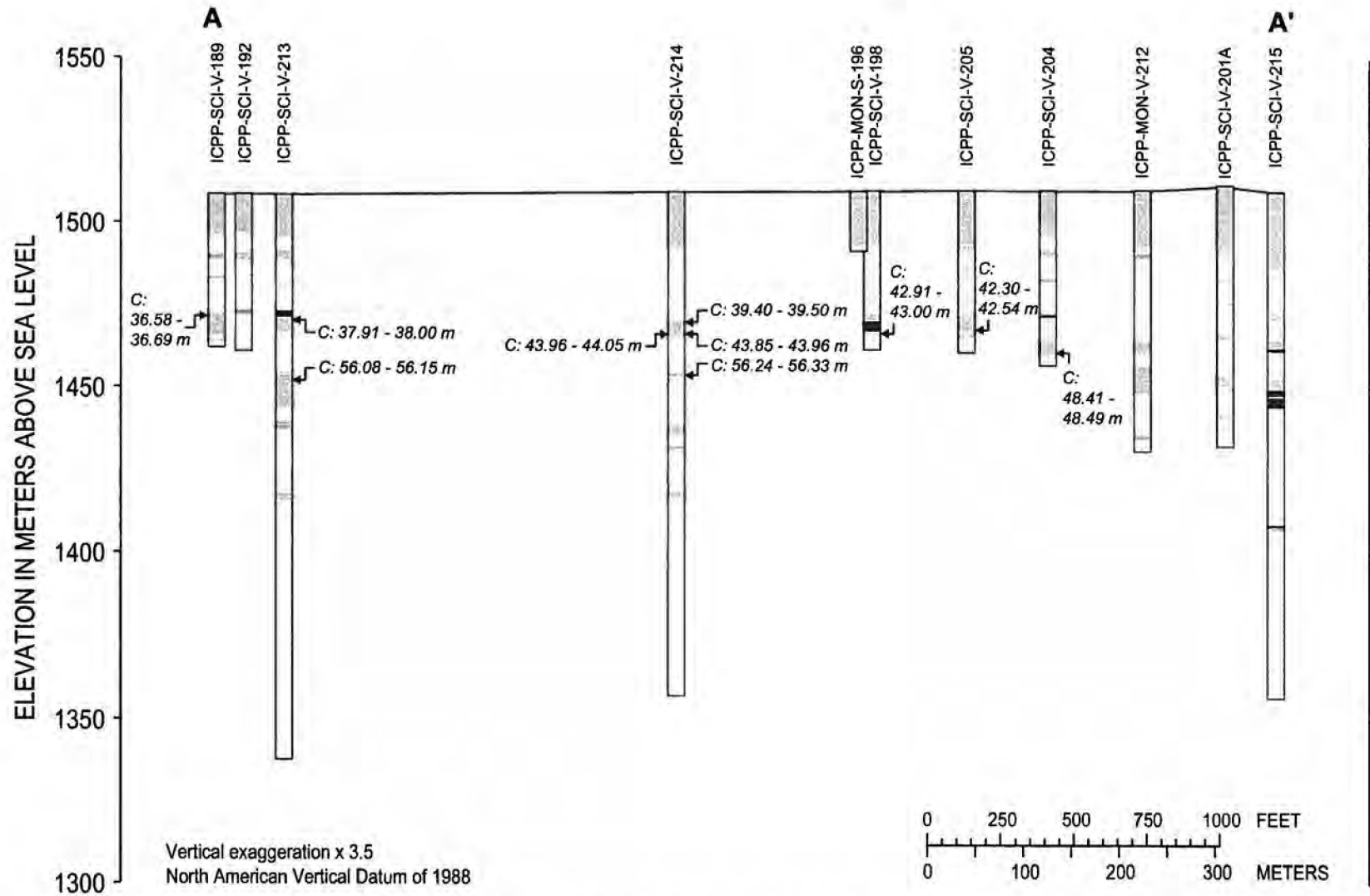
Figure 3. Borehole locations within the Vadose Zone Research Park at the Idaho National Engineering and Environmental Laboratory, Idaho (adapted from Bechtel BWXT Idaho, LLC, 2002). Cross section A-A' shows location and thickness of basalt and sedimentary intervals within selected boreholes. Locations of core samples analyzed for unsaturated hydraulic properties are also indicated—Continued.
