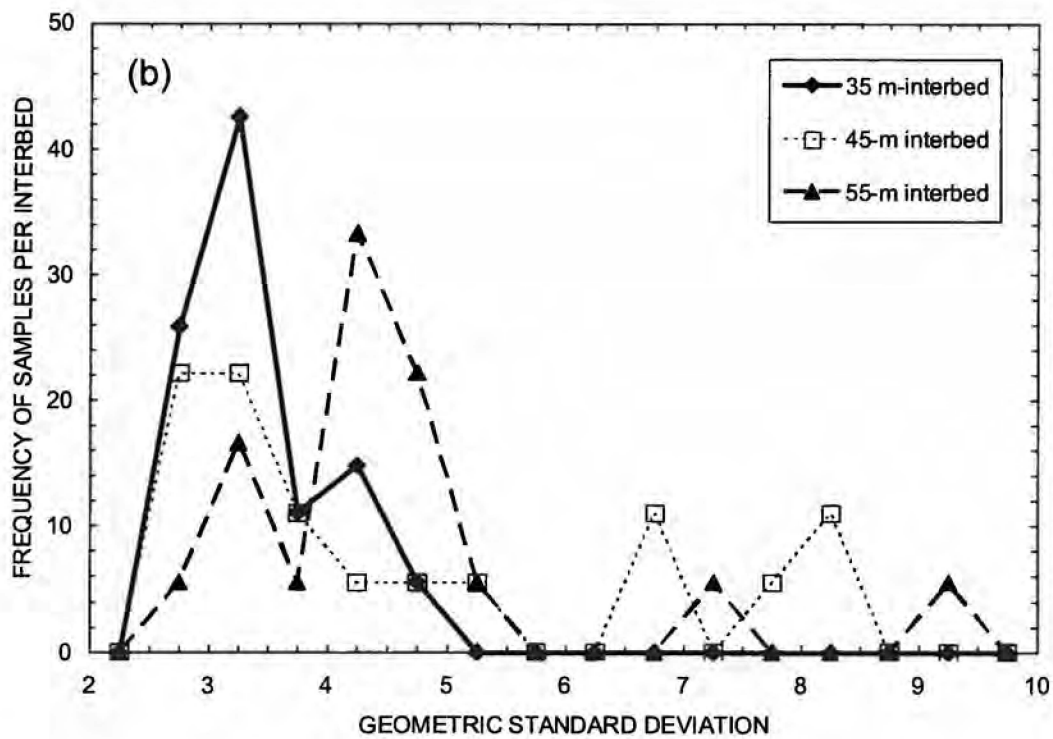
Figure 9. Frequency distribution of 90 samples (from this study and that of Perkins (2003)) within the 35-m, 45-m, and 55-m interbeds, based on (a) geometric mean particle diameter, and (b) geometric standard deviation.
