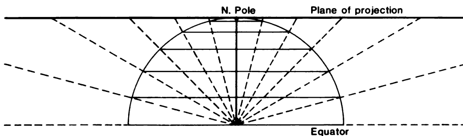
FIGURE 33.—Geometric projection of the parallels of the polar Gnomonic projection.
