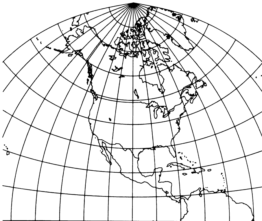
FIGURE 25.—North America on a Polyconic projection grid, central meridian long. 100^{\circ} W., using a 10^{\circ} interval. The parallels are arcs of circles which are not concentric, but have radii equal to the radius of curvature of the parallel at the Earth's surface. The meridians are complex curves formed by connecting points marked off along the parallels at their true distances. Used by the USGS for topographic quadrangle maps.
