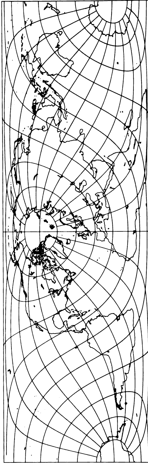
FIGURE 17.—Oblique Cylindrical Equal-Area projection, with central oblique great circle inclined 60° to the Earth's Equator. No distortion along this central line.
