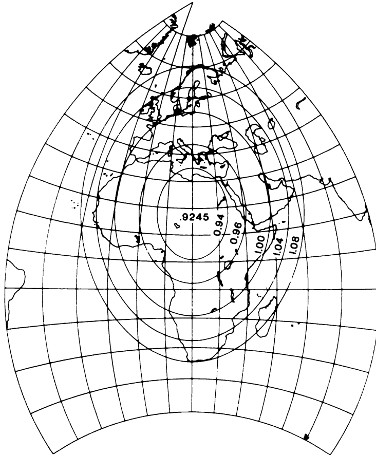
FIGURE 42.—Miller Oblated Stereographic projection of Europe and Africa, showing oval lines of constant scale. Center of projection lat. 18° N., long. 20° E.
