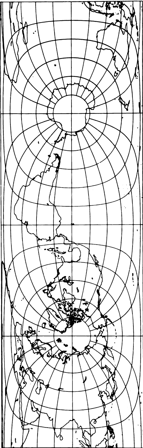
FIGURE 16.—Transverse Cylindrical Equal-Area projection. The central meridian, long. 90° W., as well as long. 90° E., coincides with the equator of the base projection.
