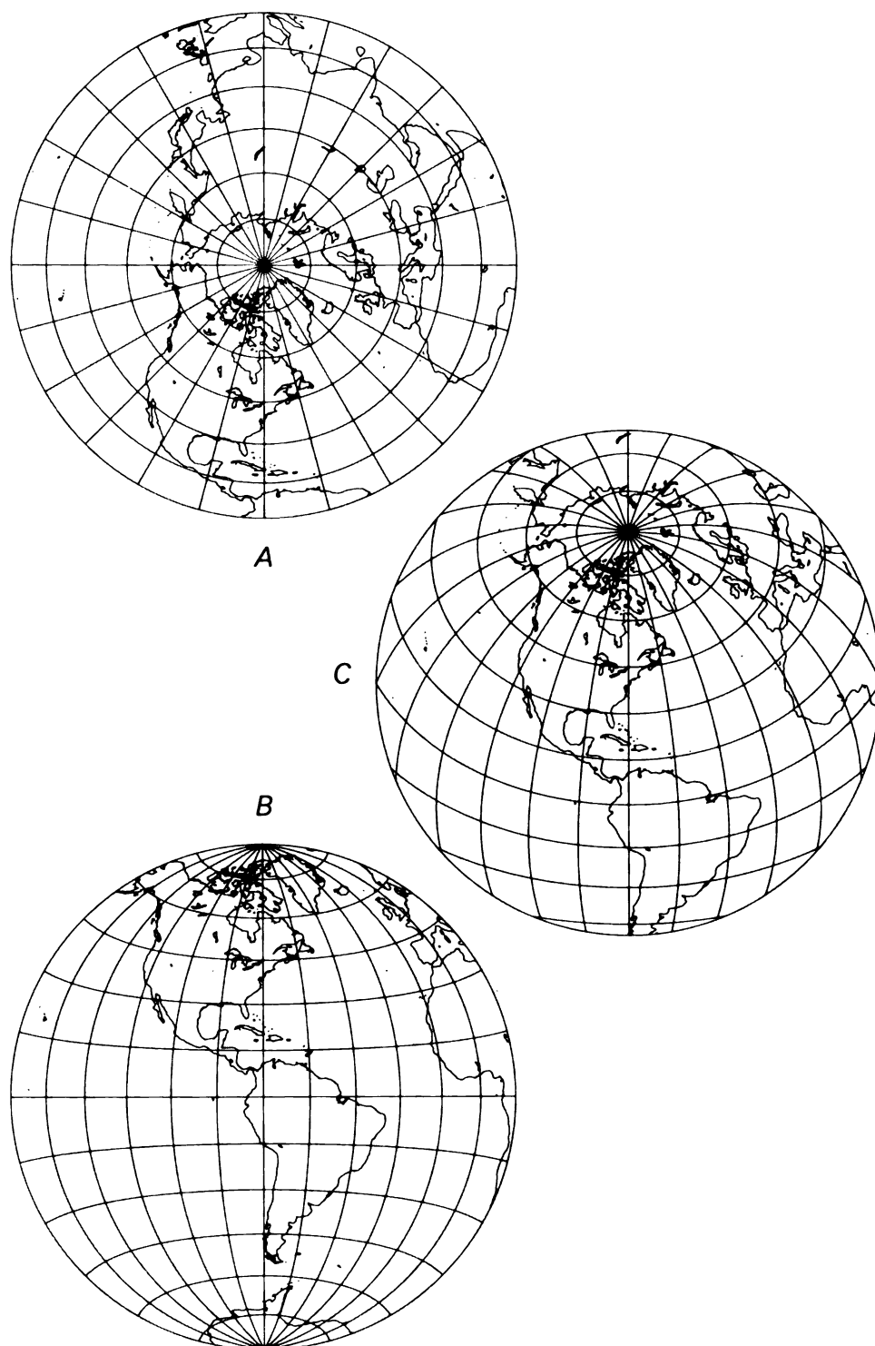
FIGURE 39.—Lambert Azimuthal Equal-Area projection. (A) Polar aspect showing one hemisphere; the entire globe may be included in a circle of 1.41 times the diameter of the Equator. (B) Equatorial aspect; frequently used in atlases for maps of the Eastern and Western hemispheres. (C) Oblique aspect; centered on lat. 40° N.
