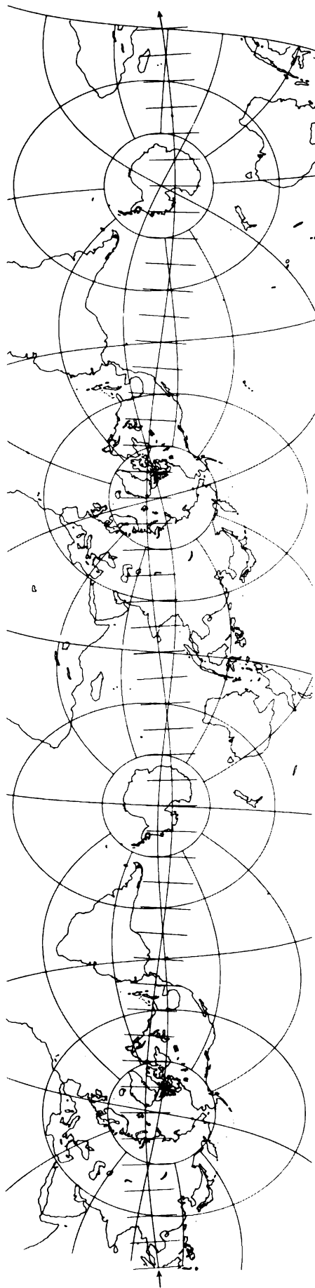
FIGURE 46.—Two orbits of the Space Oblique Mercator projection, shown for Landsat 5, paths 15 (left) and 31. Designed for a narrow band along ground-track, which remains true to scale. Note the rotation of the Earth with successive orbits. Scan lines, extended 15^\circ from groundtrack, are short lines nearly perpendicular to it.
