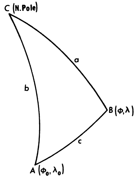
FIGURE 5.—Spherical triangle.
