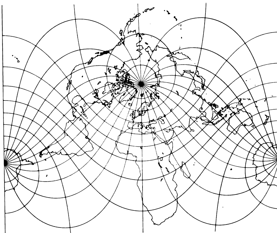
FIGURE 12.—Oblique Mercator projection with the center of projection at lat. 45° N. on the central meridian. A straight line through the point and, in this example, perpendicular to the central meridian is true to scale. The projection is conformal and has been used for regions lying along a line oblique to meridians.
