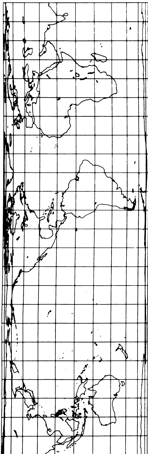
FIGURE 14.—Lambert Cylindrical Equal-Area projection. Standard parallel is the Equator. Seldom used in this form, but is suitable for equal-area strips near the Equator.
