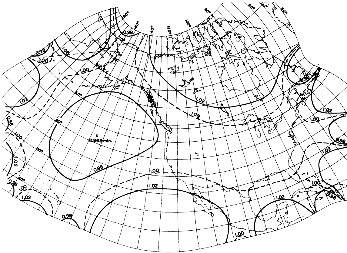
FIGURE 43.—GS-50 projection, with lines of constant scale factor superimposed. All 50 States, including islands and passages between Alaska, Hawaii, and the conterminous 48 States are shown with scale factors ranging only from 1.02 to 0.98.
