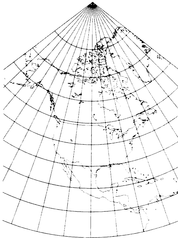
FIGURE 21.—Lambert Conformal Conic projection, with standard parallels 20° and 60° N. North America is illustrated here to show the change in spacing of the parallels. When used for maps of the conterminous United States or individual States, standard parallels are 33° and 45° N.
