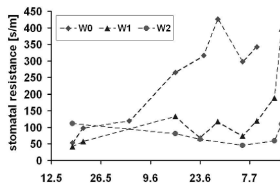
Fig2. Midday stomatal resistances ( r_s ) in 2010.
