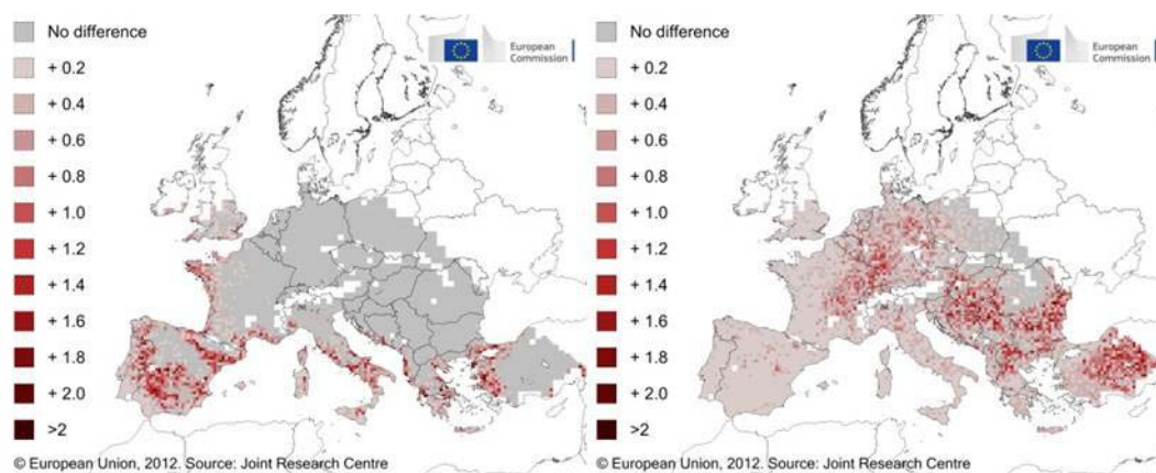
2a – Modelling approach using air temperature as the only input – 2030 vs Baseline
