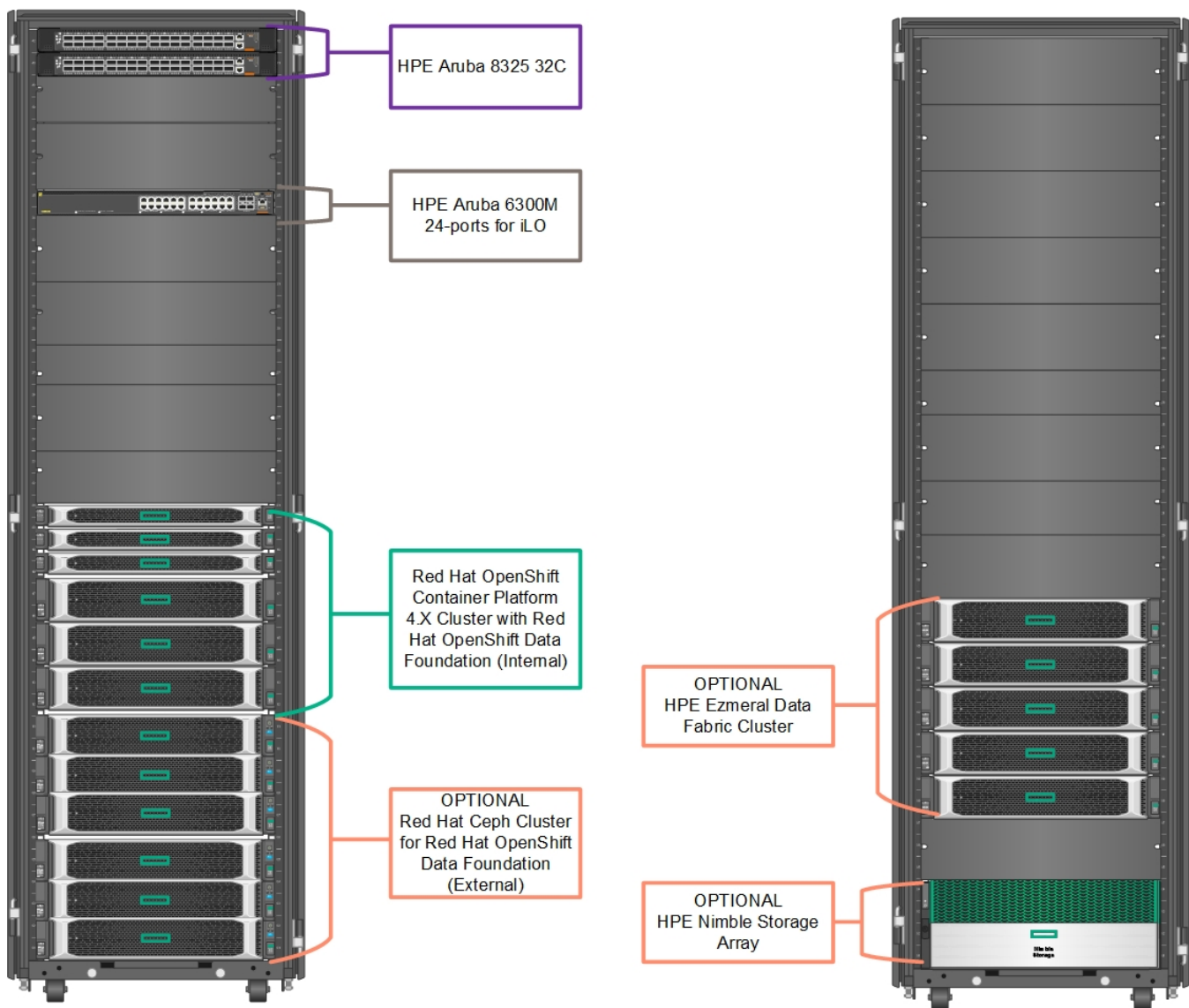
FIGURE 4. Front view of the HPE Rack and Solution Components featuring HPE ProLiant DL325 or HPE ProLiant DL385 servers, HPE Nimble Storage, and Network Switches
