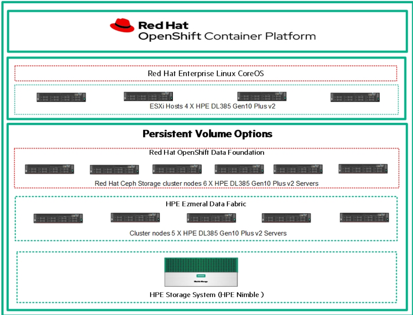
FIGURE 3. Solution Layout – Virtualized setup
