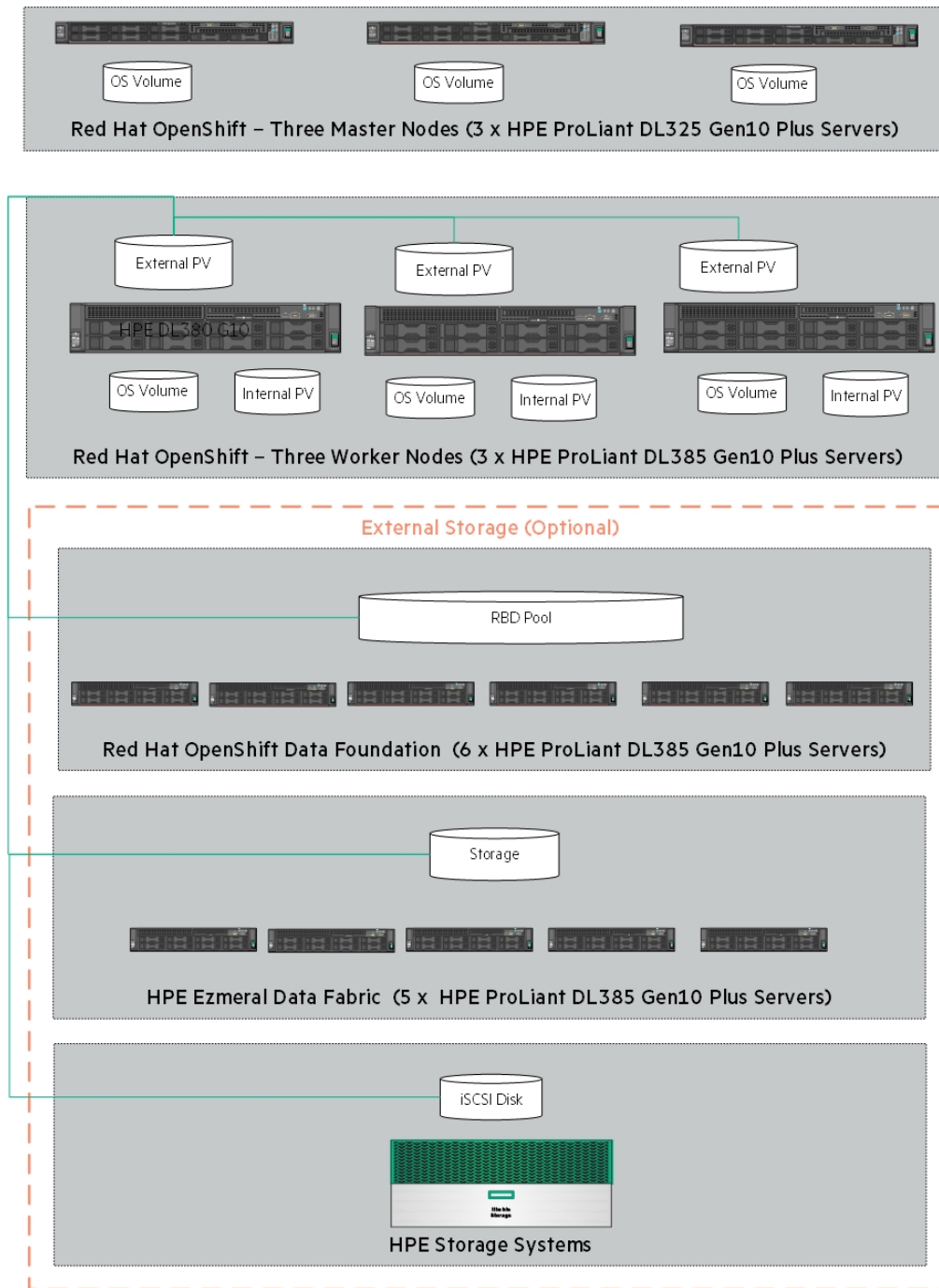
FIGURE 9. Logical storage layout in solution
