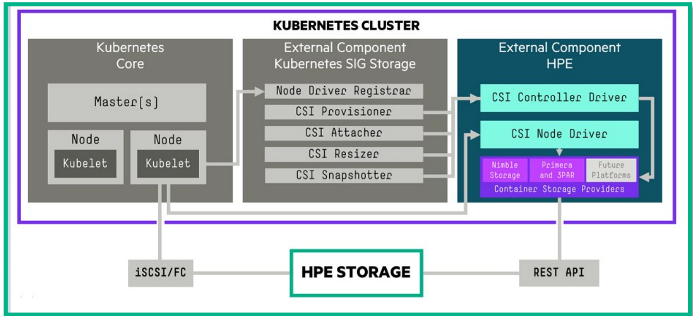
FIGURE 17. HPE CSI driver for Kubernetes architecture
