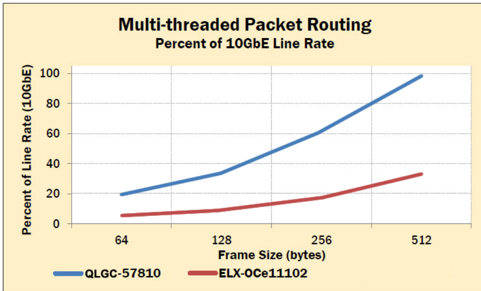
Figure 5. Multi-threaded Packet Routing ((Source: Demartek Labs, 2014))
