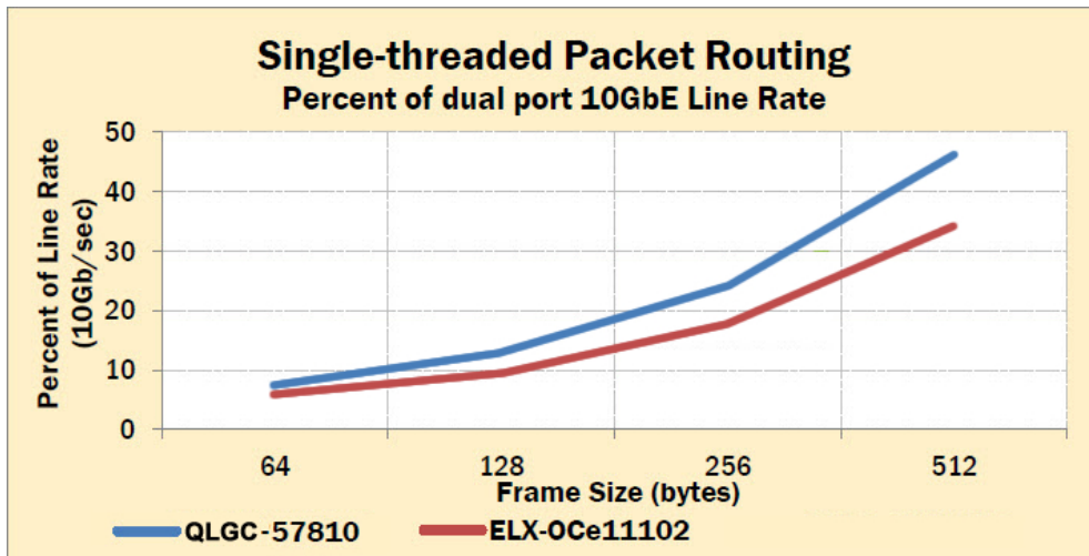
Figure 4. Single-Threaded Packet Routing ((Source: Demartek Labs, 2014))
