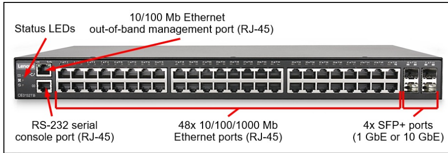
Figure 2. Front panel of the CE0152TB switch
