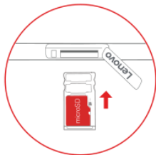
WiFi model
