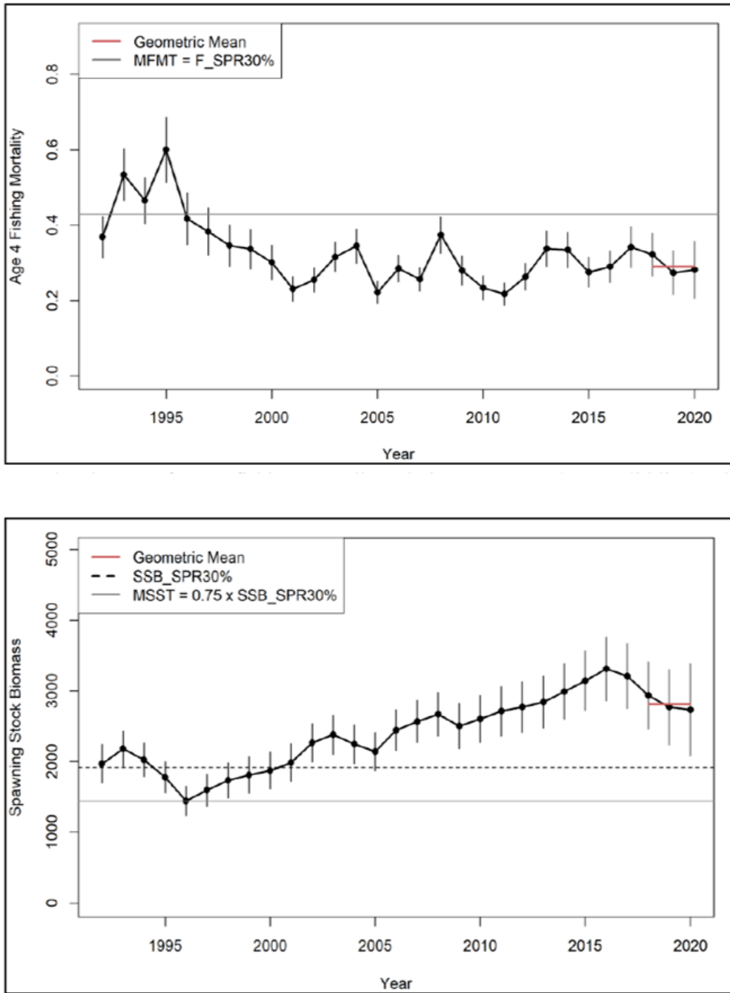
Figure 3.2.1.2.1. Top panel: annual estimates of age-4 fishing mortality relative to MFMT (grey solid line). The geometric mean of fishing mortality in the last three years ( F_{current} ) is shown in red. Bottom panel: Annual estimates of spawning stock biomass (SSB) relative to MSST (grey solid line) and SSB_{F30\%SPR} (black dashed line). The geometric mean of SSB in the last three years ( SSB_{current} ) is shown in red. For both panels: vertical lines represent approximate symmetric 95% confidence intervals.
