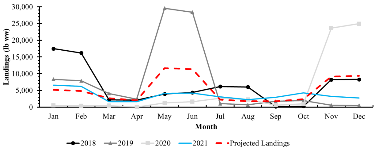
Figure A.3.3. Gulf of Mexico yellowtail snapper monthly recreational landings (lb ww) for 2018-2021, and projected future landings. Source: SEFSC Recreational ACL Dataset (October 25, 2022).
