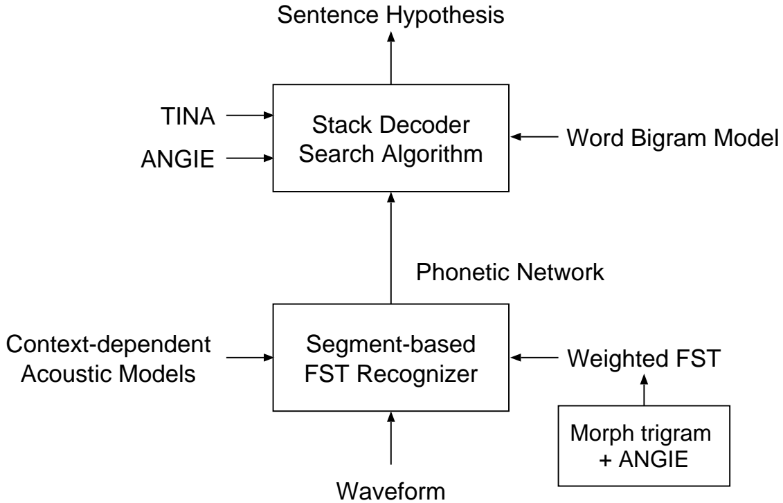
Figure 5-1: Block Diagram of FST-Based Two-Stage System.
