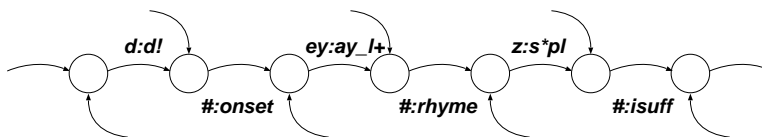
Figure 6-1: Schematic of an FST for the Word Days. The input and output labels, given at the arcs, are delineated by a “:”. The phonetic realization is given by /d ey z/, and the letter-phoneme baseform is given by /d! ay_l+ s*pl/. The “isuff” label is emitted indicating the inflectional suffix at the column associated with the plural and the /s*pl/ letter-phoneme.
