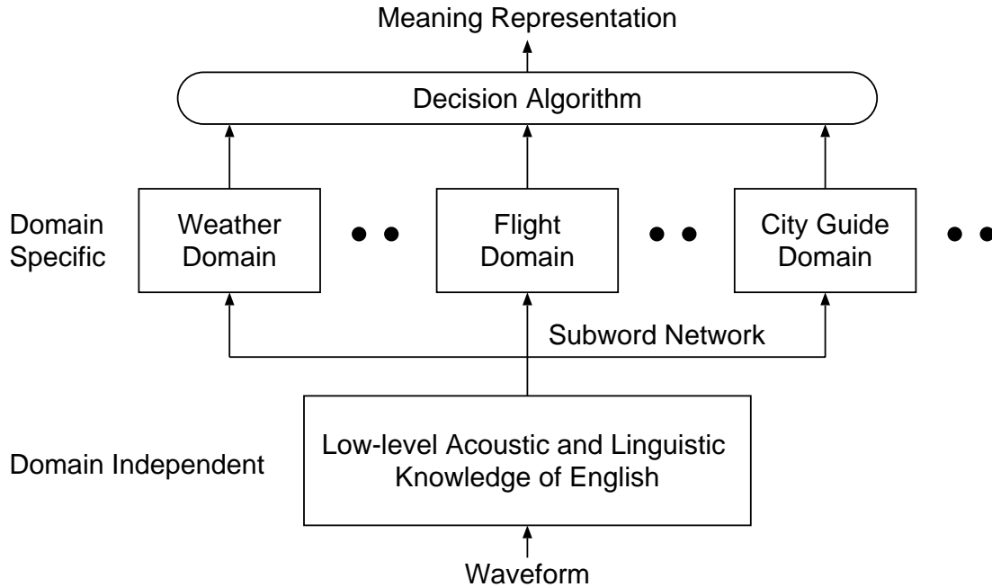
Figure 2-2: A Multi-Stage Multi-Domain Speech Understanding System.
