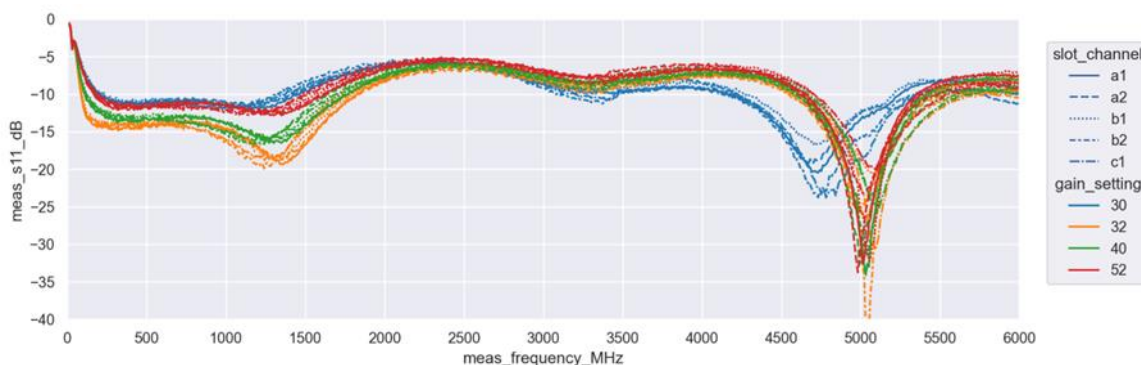
Figure 10.4.21. Typical S11 [dB]
