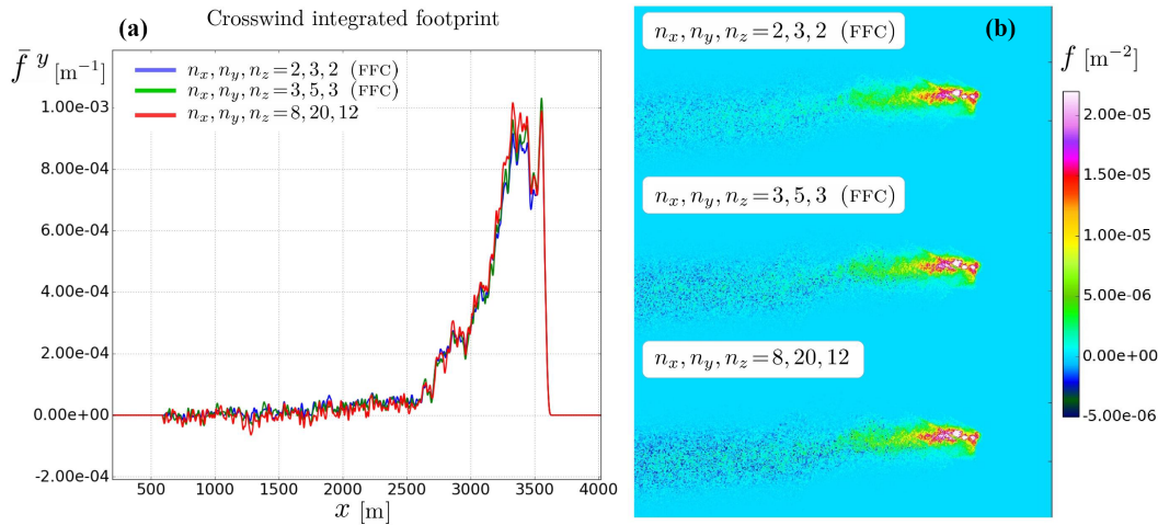
Figure 7. Comparison of identically normalized footprint distributions (b) and their crosswind integrations (a) obtained either by applying (1) the far-field correction (FFC) method and selective assembly or (2) the standard coordinate rotation while utilizing the uniform 1 m resolution of the LES grid in the target volume discretization. The subvolume contributions included in the n_x, n_y, n_z = 8, 20, 12 result were selected to correspond with the effective target volume \mathcal{V}_{T,\text{eff}} = \sum_{i,j,k \in \mathcal{K}} \mathcal{V}_{i,j,k} determined via the selective assembly for n_x, n_y, n_z = 3, 5, 3 .
