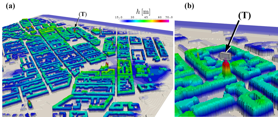
Figure 3. A three-dimensional rendering of the urban topography near Hotel Tornii (a) and a close-up featuring the target box (T) for particle capturing (b).
