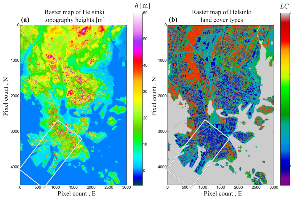
Figure 1. Raster maps of topography height h (a) and land cover types LC (b) from Helsinki area. The rectangle in the bottom left corner is aligned with southwesterly wind and represents the area of interest for the footprint analysis. In the surface type classification each pixel (2 m) is categorized according to the following numbering: 0 = building, 1 = impervious (rock, paved, gravel), 2 = grass, 3 = low vegetation, 4 = high vegetation, and 5 = water.
