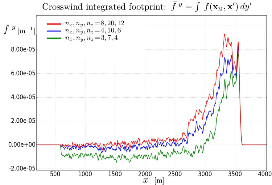
Figure 5. Crosswind integrated distributions of piecewise postprocessed footprints obtained with different levels of target volume discretizations using \langle \bar{w} \rangle_{i,j,k} from LES solution. Anomalous contributions from subvolumes immediately behind or in contact with the tower structure were omitted from the assembly (refer to Sect. 2.3.2).
