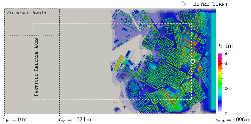
Figure 2. Visualization of the topography height distribution underlying the LES domain. The particle release area is enveloped by a white dashed line. The size of the precursor domain is outlined in the top left corner. The location of the turbulence recycling plane is marked by a black dotted line at x_{rc} .
