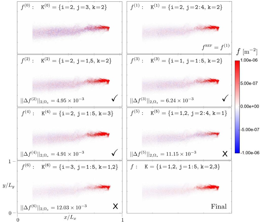
Figure 6. Illustration of the selective assembly of the final footprint for n_x \times n_y \times n_z = 3 \times 5 \times 3 = 45 . Values of \|\Delta f^{(l)}\|_{2,\Omega_\star} indicating discrepancy between f^{\text{REF}} and f^{(l)} are shown where applicable. Acceptable candidates are marked by \checkmark and the rejected by \times . Note the use of short-hand notation, e.g., 1:3 = 1, 2, 3 .
