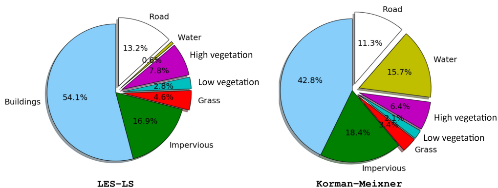
Figure 11. Comparison of source-area fractions a_e resulting from applying f_{LES} and f_{KM} to the raster map of land cover types in Fig. 10.
