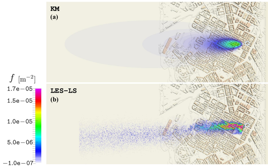
Figure 8. Comparison of identically normalized LES–LS (b) and KM (a) footprint distributions merged with the urban topography model of Helsinki. The location of the EC sensor (Hotel Tornio) building is indicated with a white circle.
