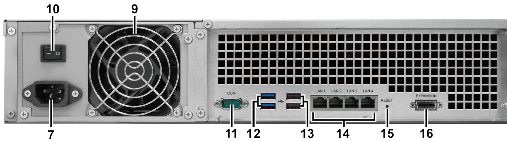
RS2416RP+
