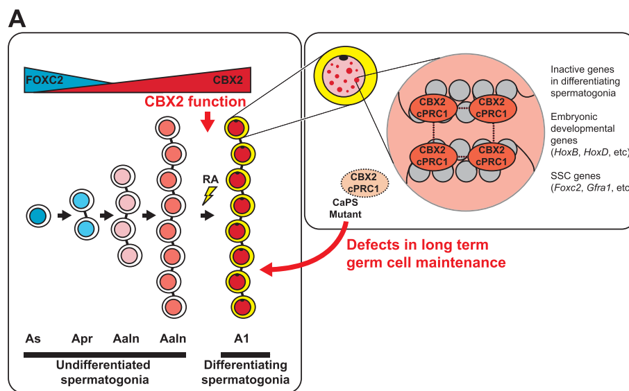
Figure 8. A model of CBX2 function at the exit from the SSC state. CBX2 expression is up-regulated as A-single or A-paired spermatogonia differentiate to A-aligned spermatogonia. CBX2 expression further increases at A1 spermatogonia when the cells irreversibly commit to differentiation. CBX2 function is required specifically for the production of A1 spermatogonia. In differentiating spermatogonia, CBX2 forms Polycomb bodies that encompass its target genes that need to remain repressed. Disruption of the CaPS region of CBX2 results in defects in the long-term maintenance of germ cells.
