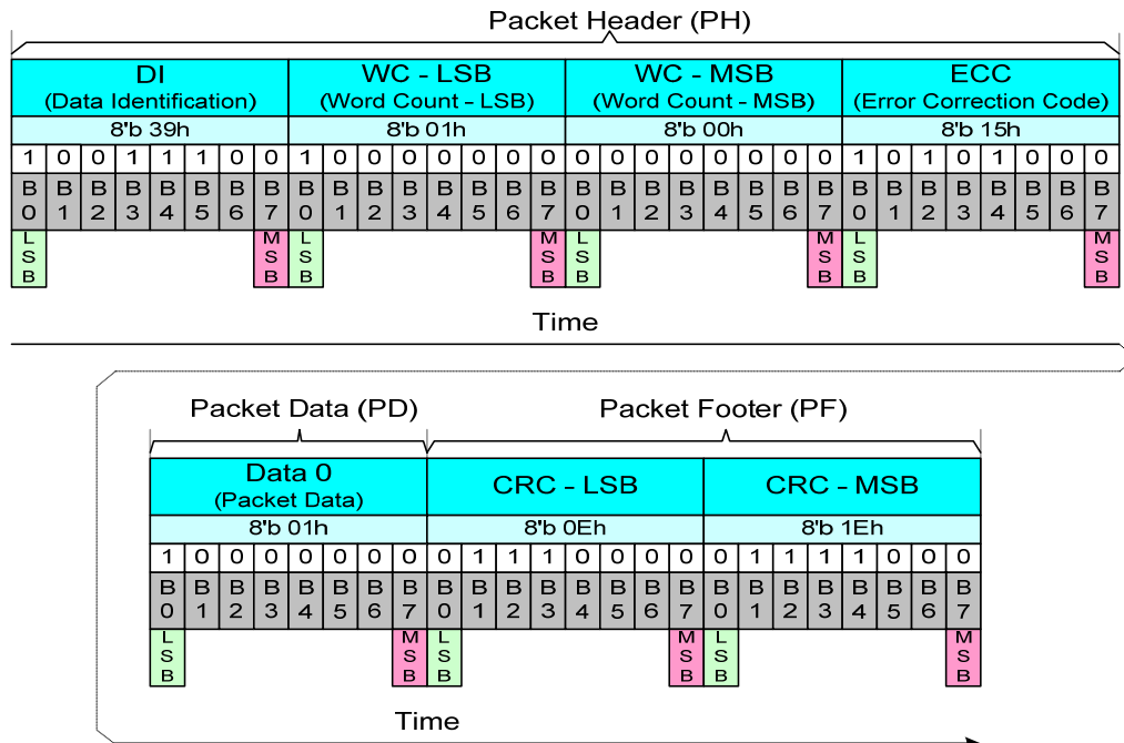
Figure 46 Packet Header (PH) on Long Packet (LPa)
