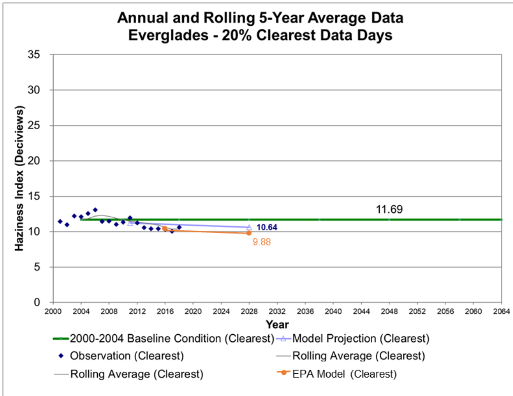
Figure 7-15: 20% Clearest Days Rate of Progress for Everglades
