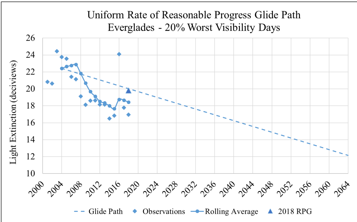
Figure 13-5: Everglades Visibility Impairment on the 20% Worst Visibility Days, Glide Path, and 2018 RPG
