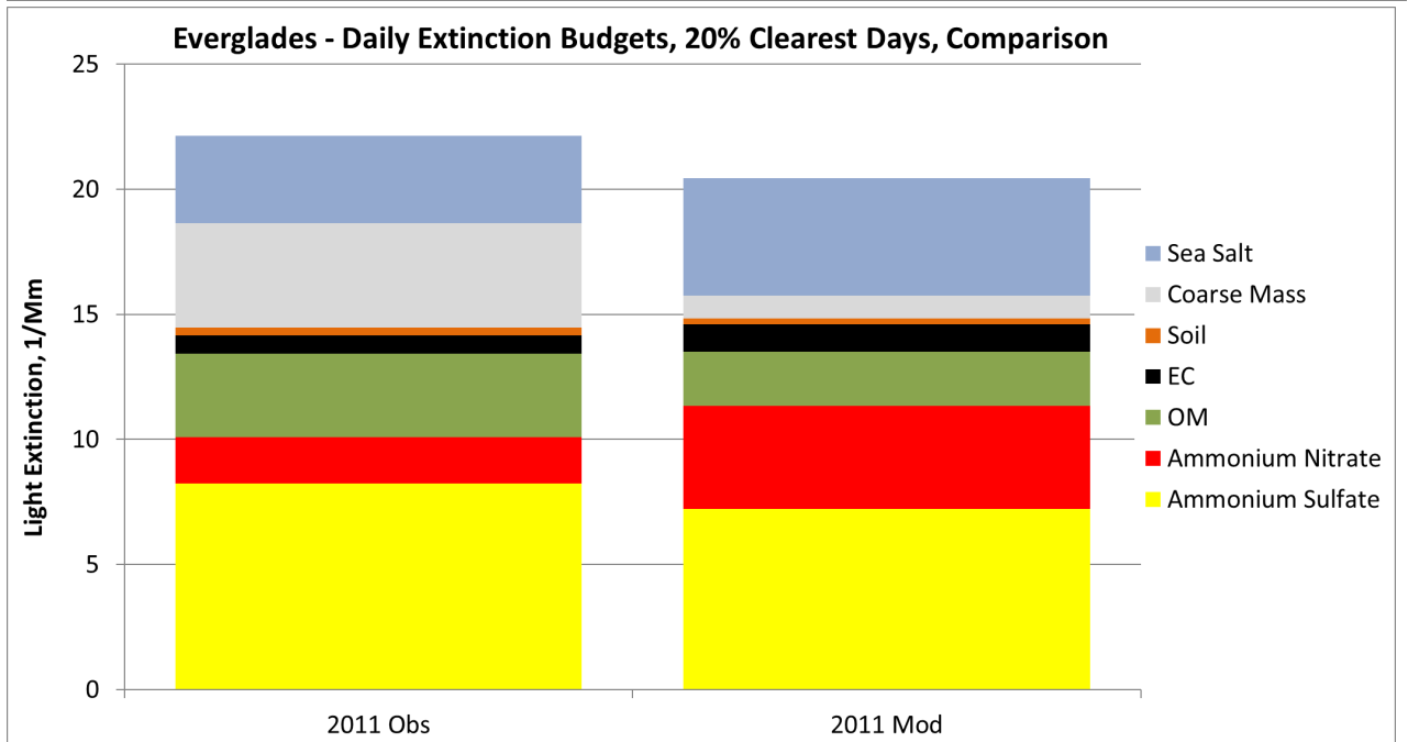
Figure 6-22: Stacked Bar Charts for Average Light Extinction on the 20% Most Impaired Days (top) and 20% Clearest Days (bottom) at Everglades
