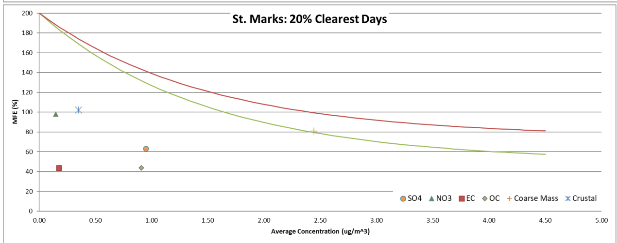
Figure 6-56: Bugle Plots of MFB (top) and MFE (bottom) for Sulfate, Nitrate, Elemental Carbon, Organic Carbon, Coarse Mass, and Crustal Concentrations on the 20% Clearest Days at St. Marks
