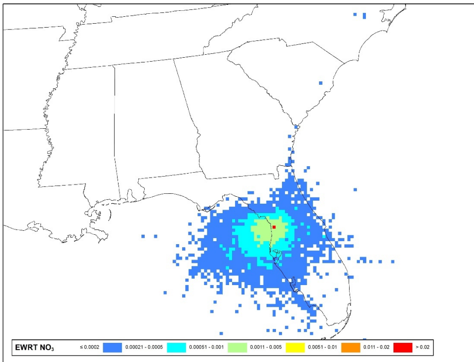
Figure 7-45: Nitrate Extinction Weighted Residence Time (Nitrate EWRT per 12-km Modeling Grid Cell) for Chassahowitzka - Full View (top) and Class I Zoom (bottom)
