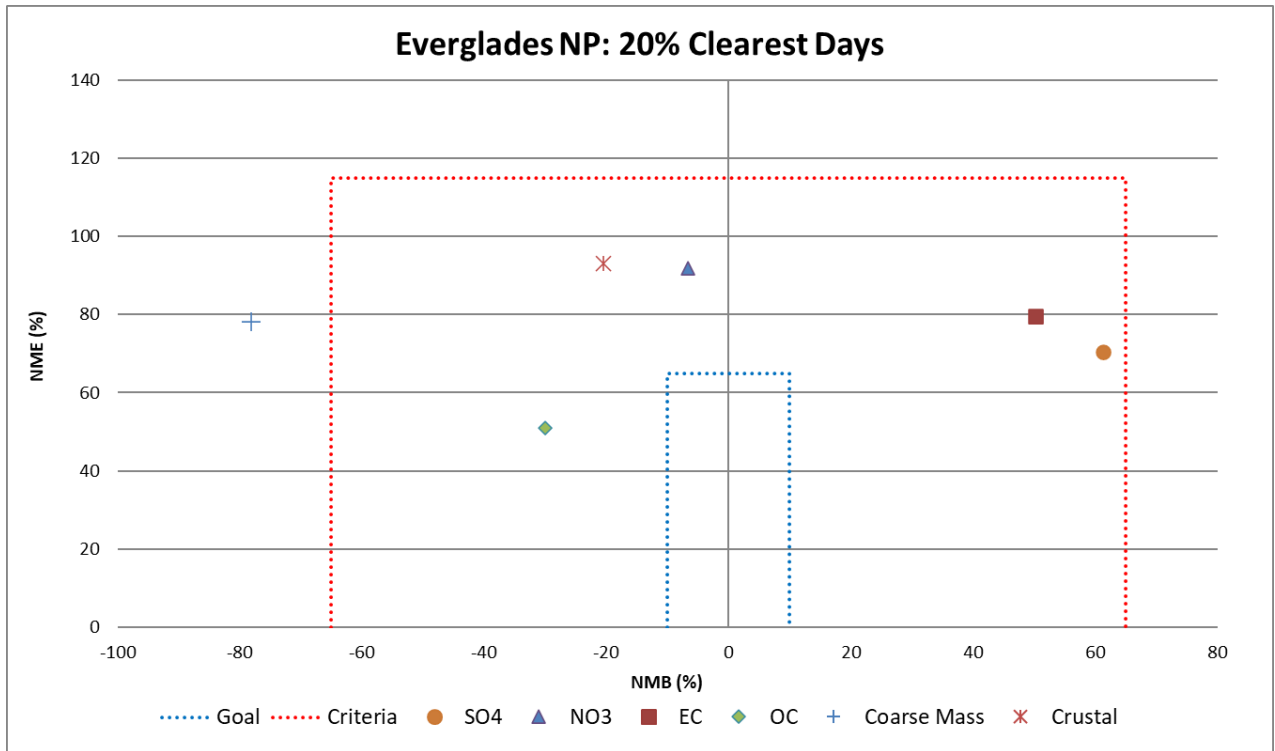
Figure 6-52: Soccer Plot for Sulfate, Nitrate, Elemental Carbon, Organic Carbon, Coarse Mass, and Crustal Concentrations on the 20% Clearest Days at Everglades
