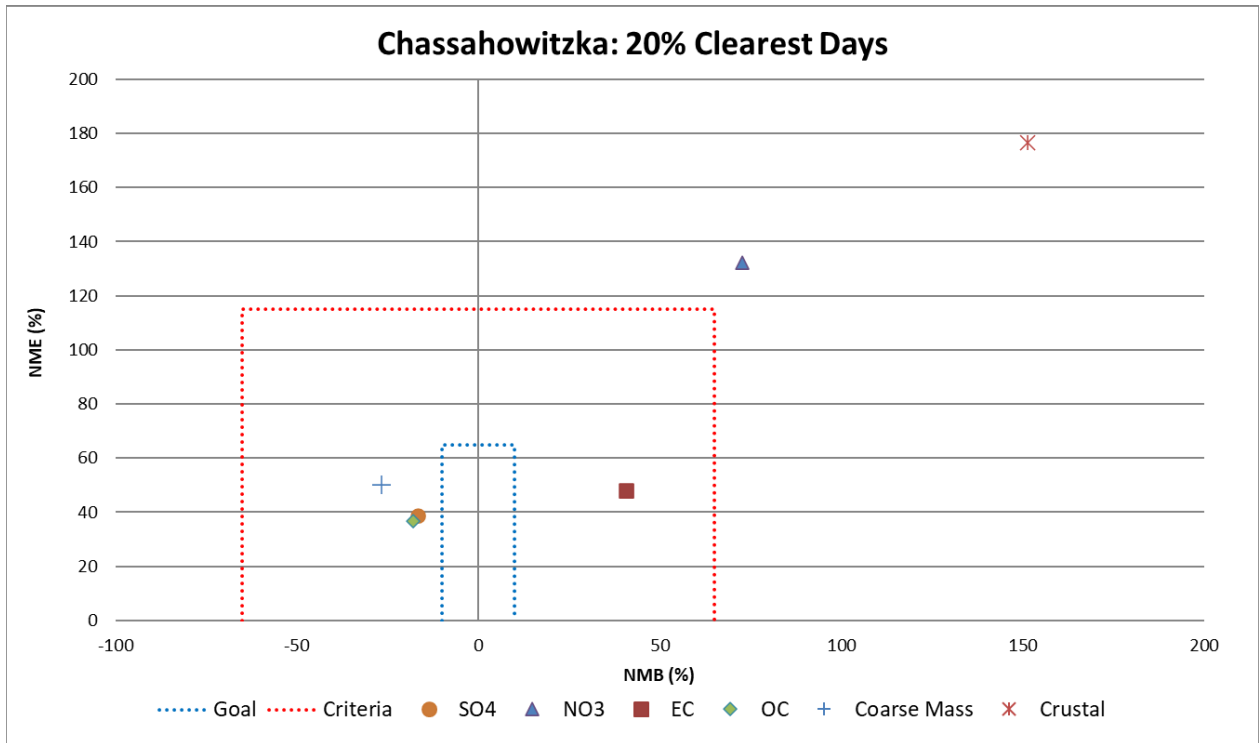
Figure 6-48: Soccer Plot for Sulfate, Nitrate, Elemental Carbon, Organic Carbon, Coarse Mass, and Crustal Concentrations on the 20% Clearest Days at Chassahowitzka
