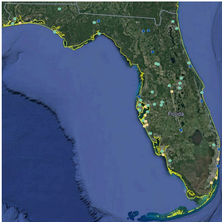
Figure 6-3: ME (ppb) of MDA8 Ozone \geq 60 ppb Over the Period May-September 2011 at AQS Monitoring Sites in VISTAS12 Domain (top) and in Florida (bottom)
