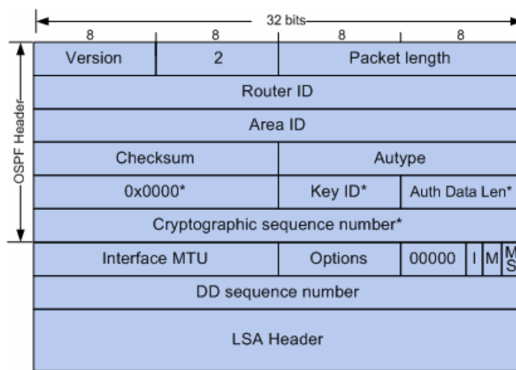
Figure 10-40 DD Packet
