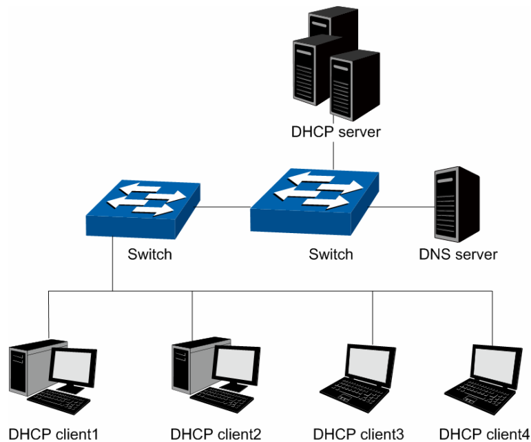
Figure 10-4 DHCP model
