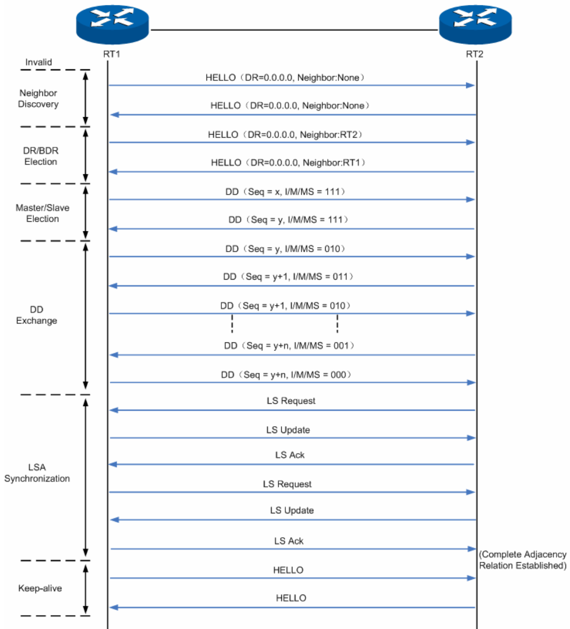
Figure 10-31 Steps to Establish a Complete Adjacency Relation
