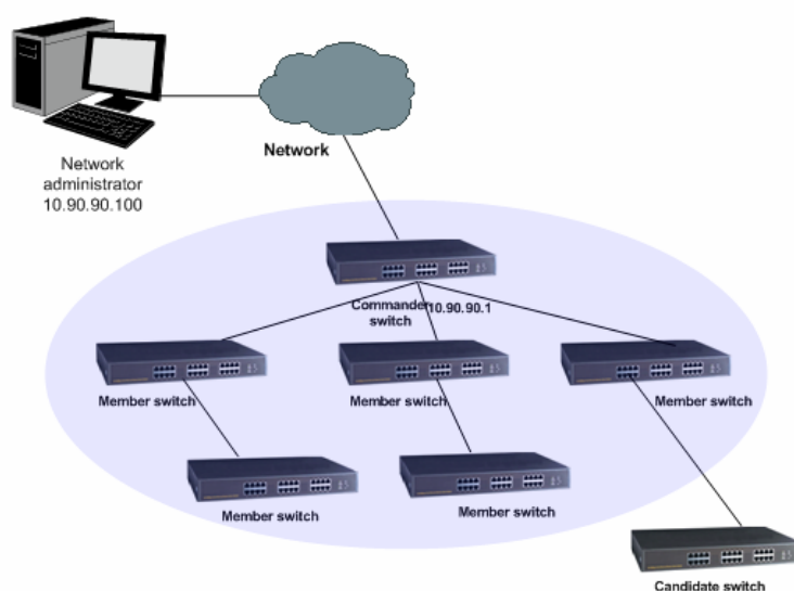
Figure17-1 Cluster topology
