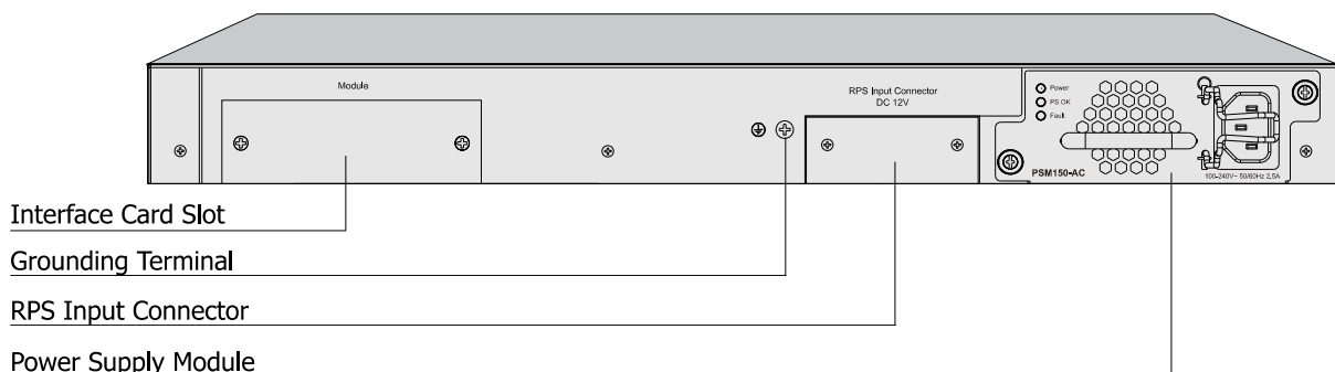
Figure 2-2 Rear Panel (1)
