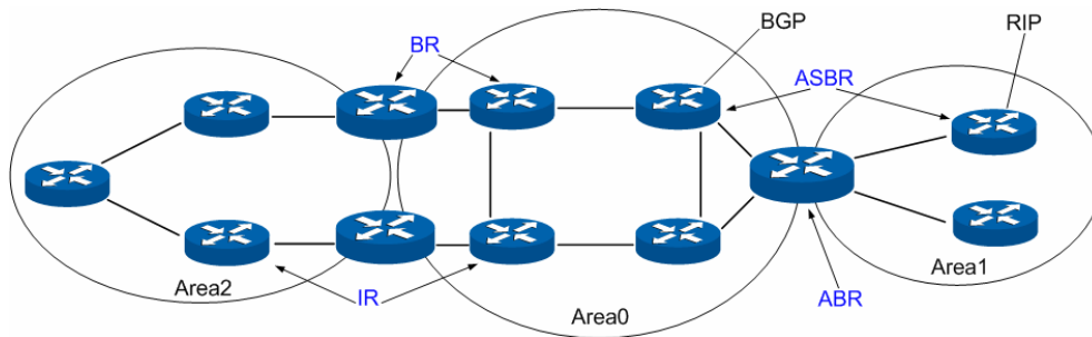
Figure 10-34 Classification of Routers
