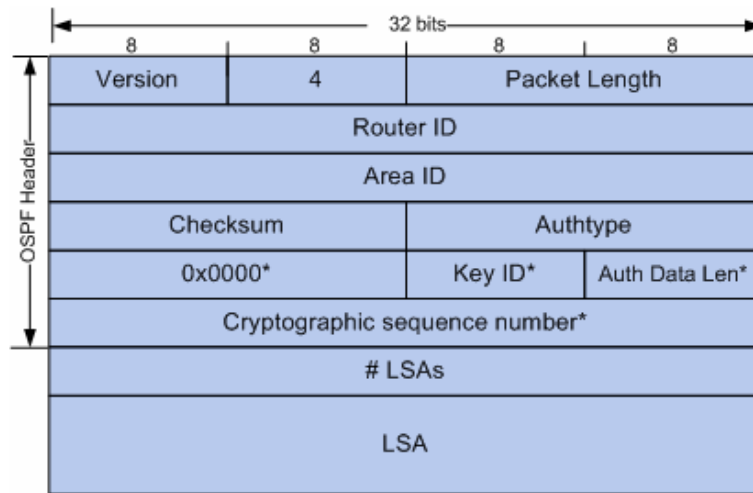
Figure 10-42 LSU Packet
