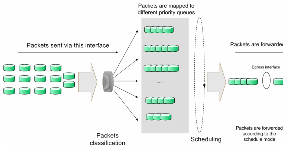
Figure 12-1 QoS function
