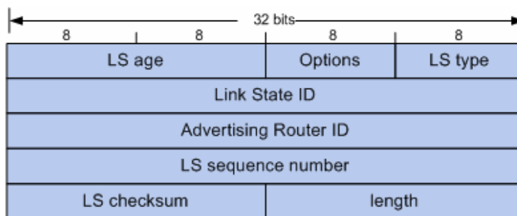
Figure 10-43 LSA Header
