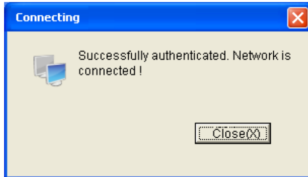
Figure C-15 Successfully Authenticated
