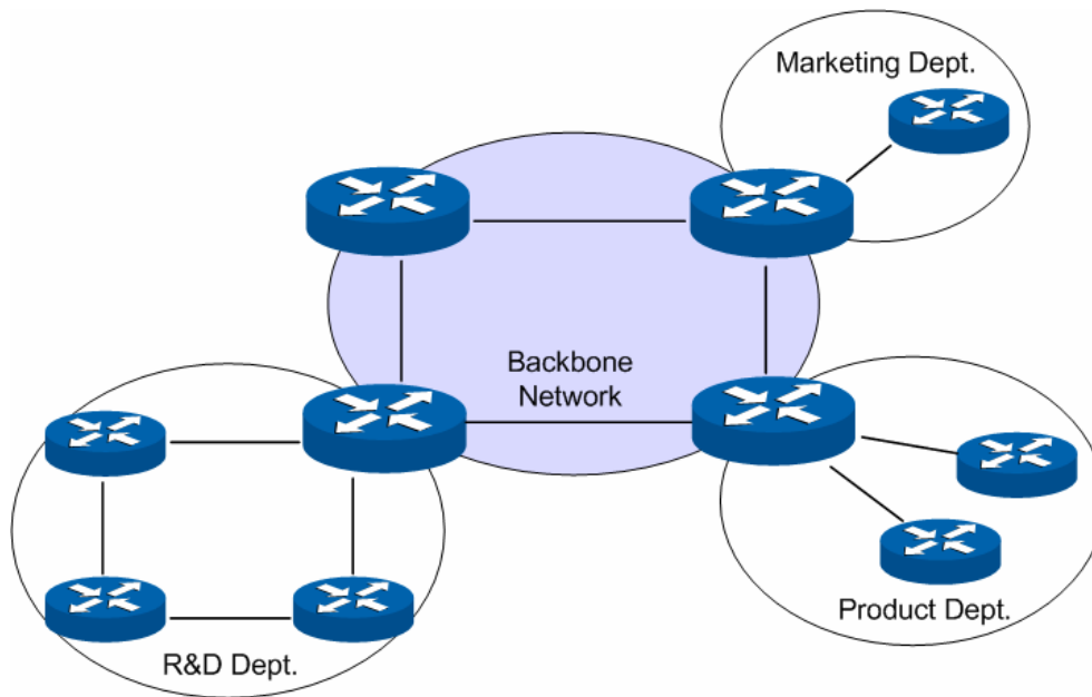
Figure 10-29 Common Scenario for OSPF routing protocol
