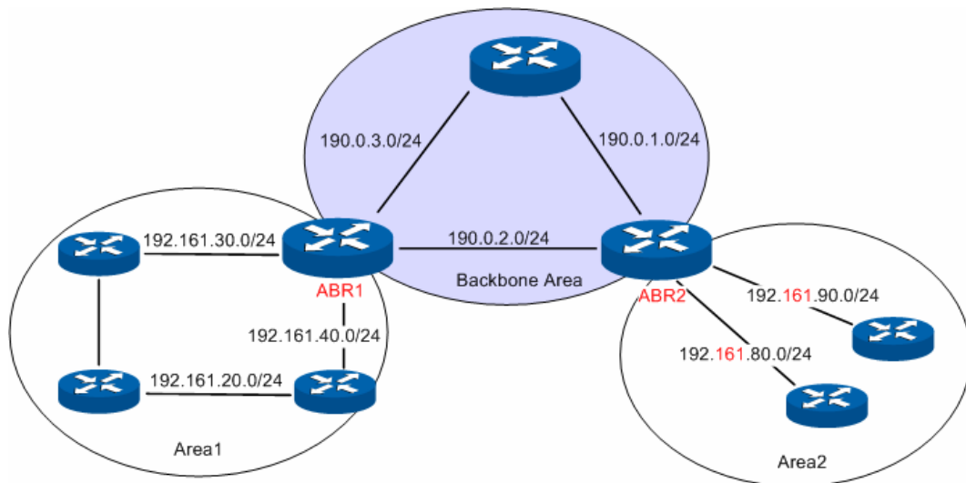
Figure 10-37 Discontinuous Network Segment
