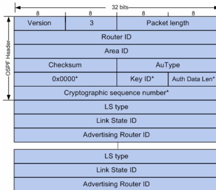
Figure 10-41 LSR Packet
