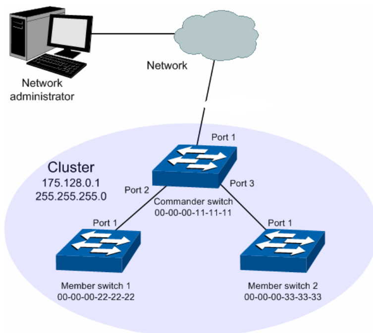
Figure17-19 Network diagram
