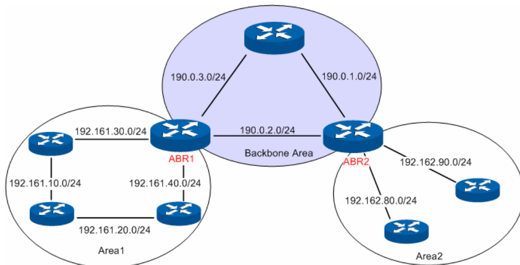
Figure 10-36 ABR Route Summarization
