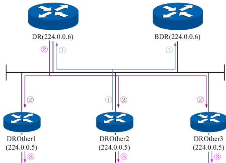
Figure 10-32 Flooding of the LSA
