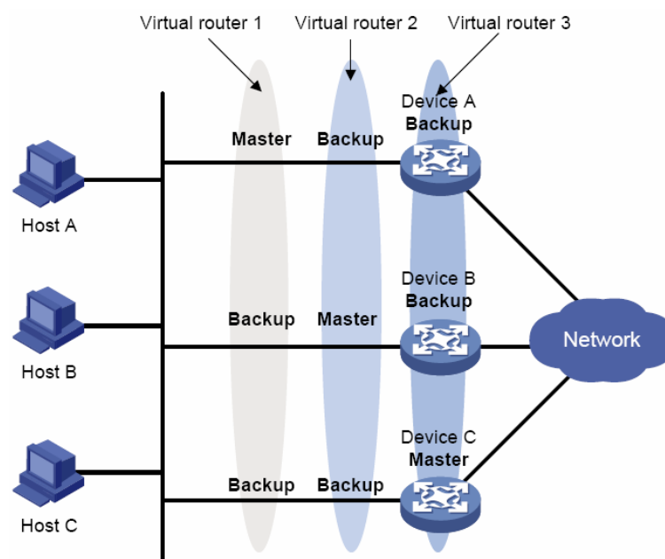
Figure 10-57 VRRP Load Balancing
