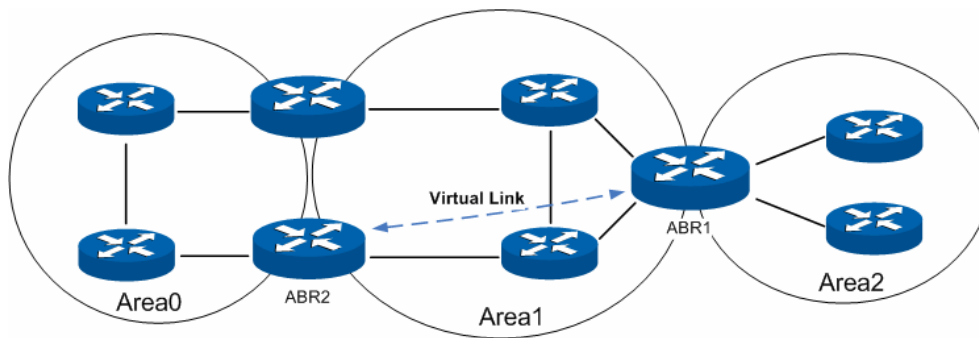
Figure 10-35 Virtual Link Sketch
