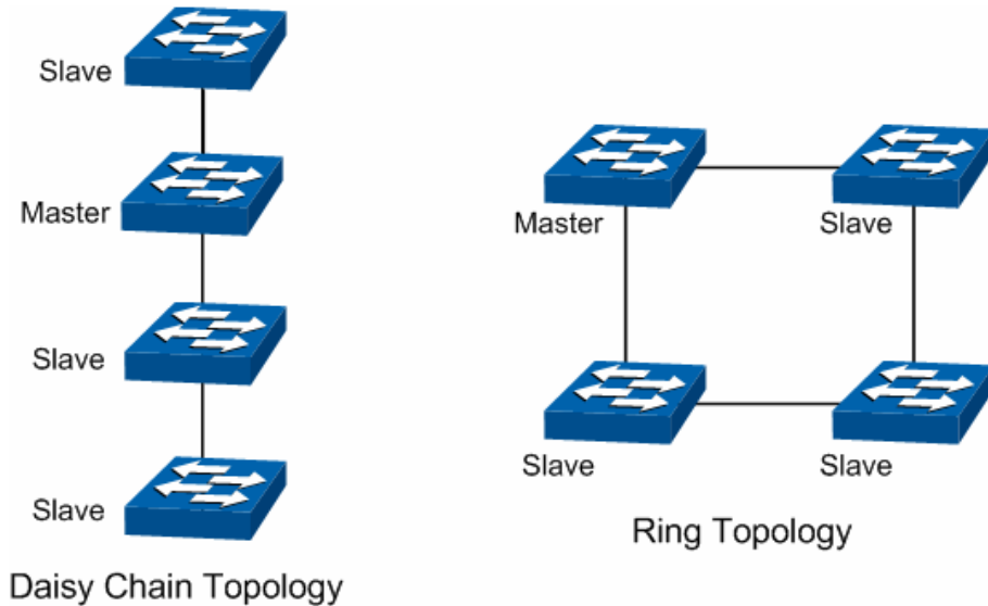
Figure 5-6 Stack Connect Topology
