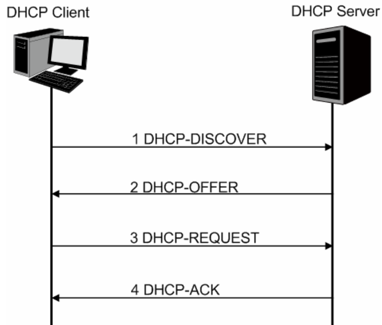
Figure 10-5 The Process of DHCP
