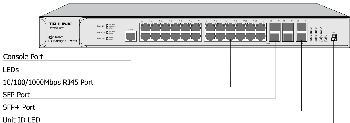
Figure 2-1 Front Panel
