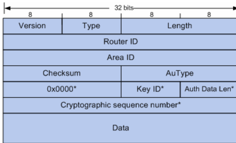
Figure 10-38 OSPF Header
