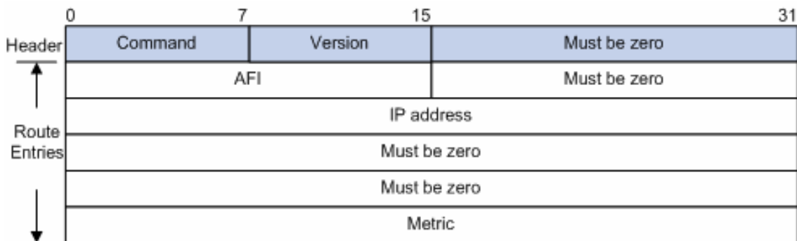
Figure 10-23 RIPv1 Message Format
