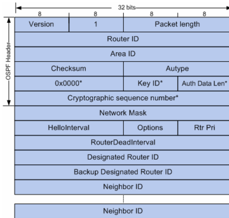
Figure 10-39 HELLO Packet
