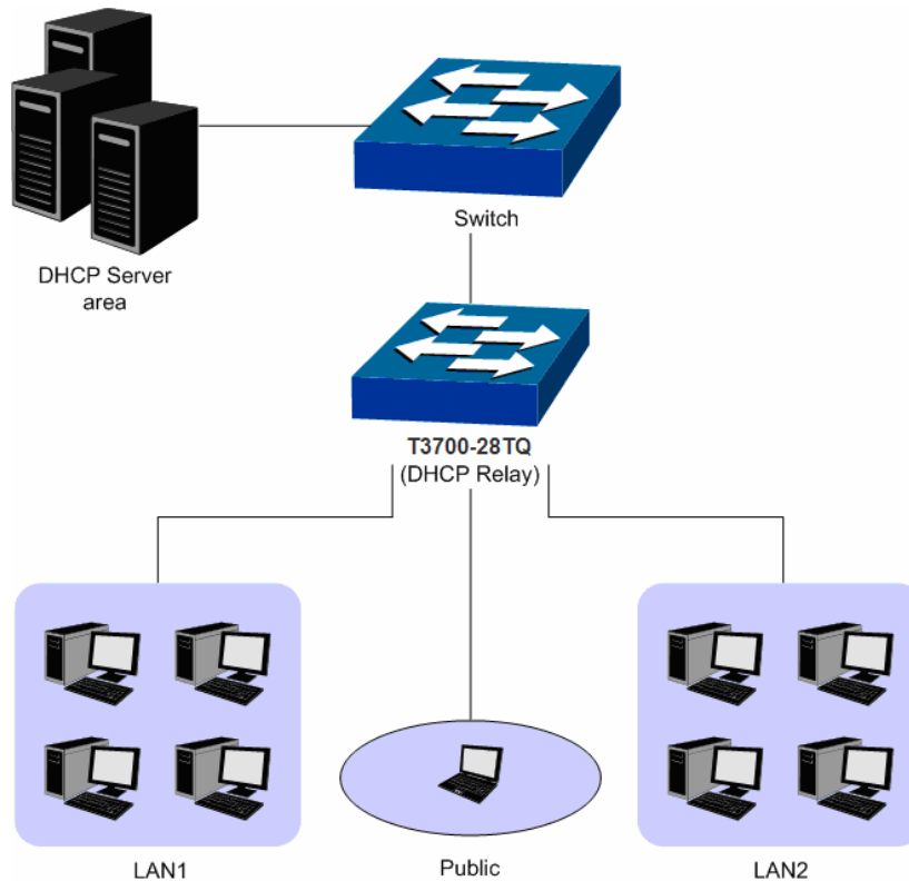
Figure 10-14 DHCP Relay Application
