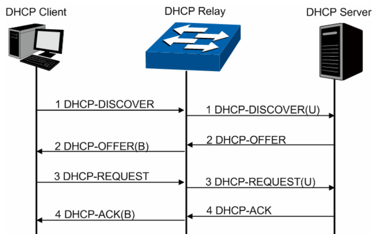
Figure 10-15 DHCP Relay Process
