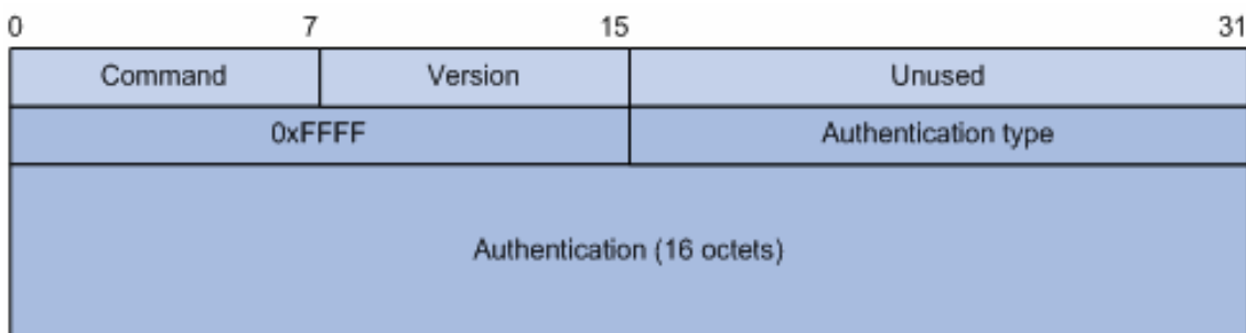
Figure 10-25 RIPv2 Authentication Message
