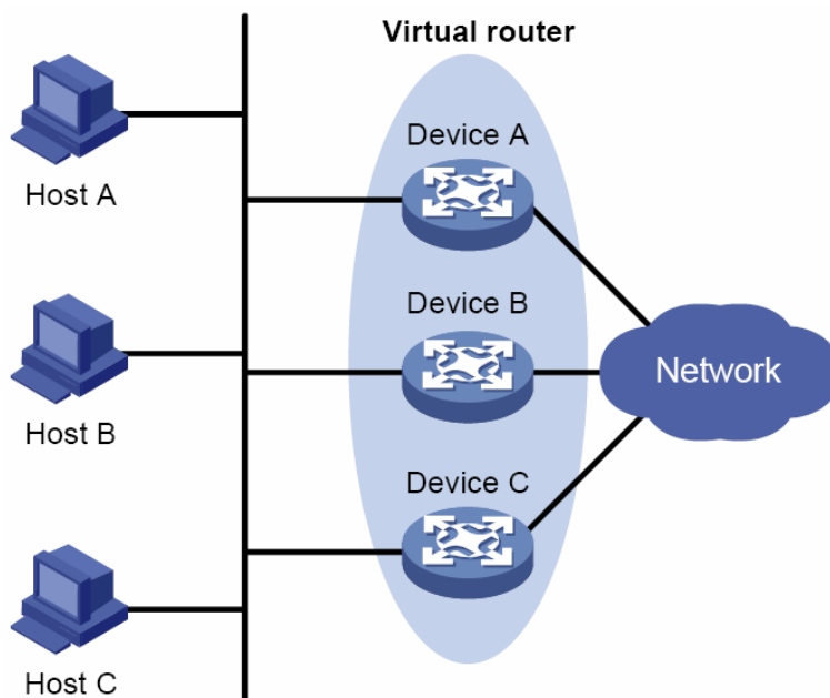
Figure 10-56 Typical Networking Application Diagram
