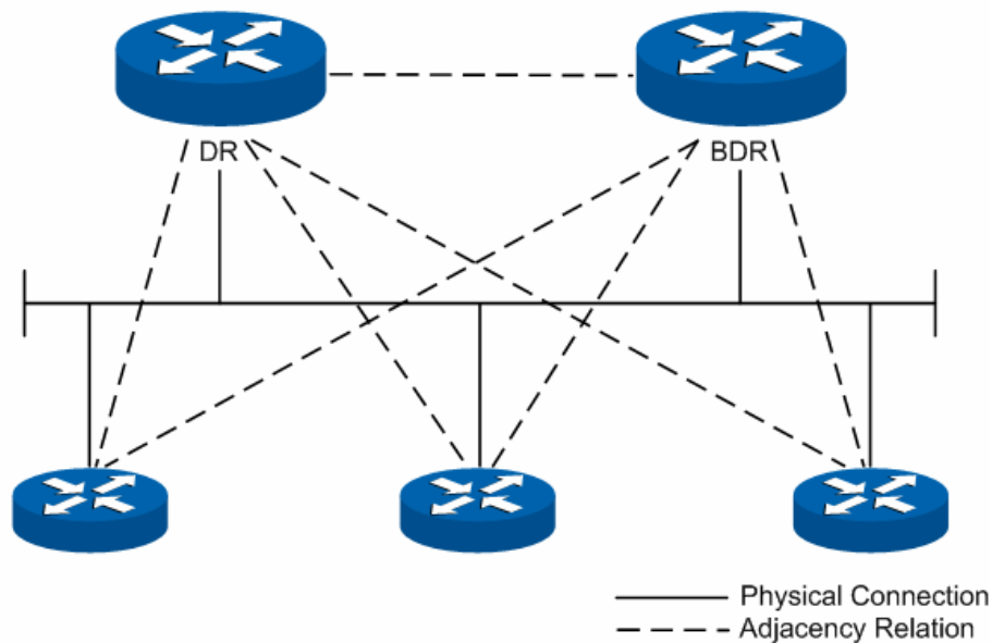
Figure 10-30 Diagram of DR/BDR Adjacency Relation
