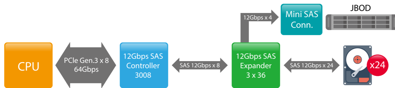
TVS-ECx80U-SAS R2 12Gbps SAS model block diagram
