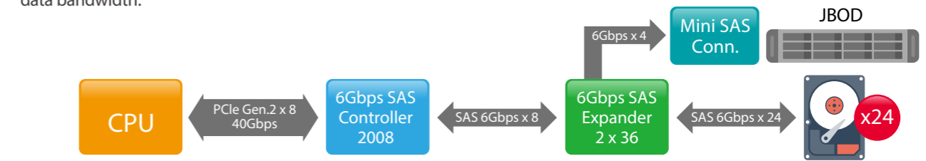
TS-x79U-SAS 6G SAS model block diagram
