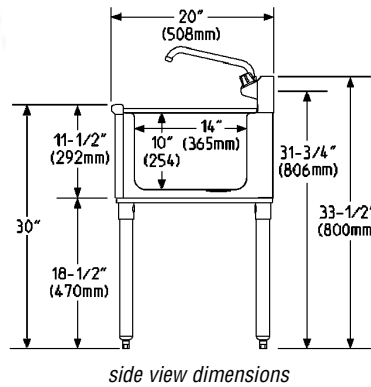
side view dimensions
