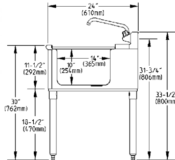
side view dimensions
