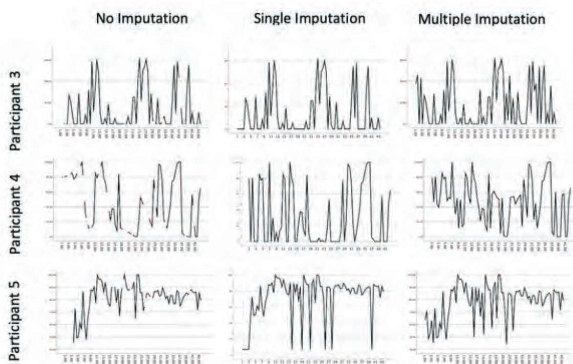
Figure 1. Fluctuations of psychological inflexibility: by participants and imputation techniques.
