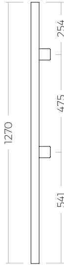
SSPSQ40X42E End Post 42"
