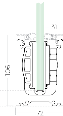
Recessed or No Cladding
