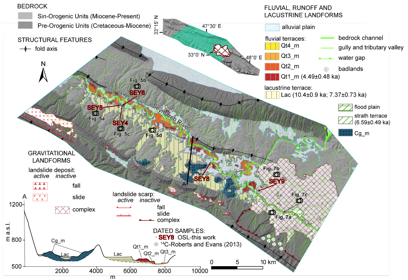
Figure 6: Map of the lacustrine and alluvial terrace suite and of the most significant landforms for the valley slope evolution upstream of the Seymarche landslide.
