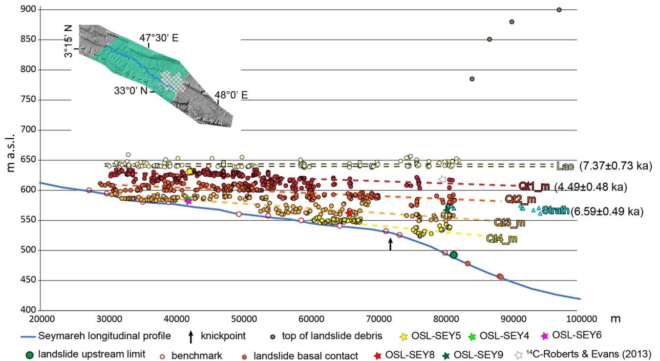
Figure 10: Projection along the longitudinal profile of Seymareh River of the post-failure geomorphic markers They are named according to the legend of Fig. 6 (see the text for explanation). The obtained OSL ages are indicated.
