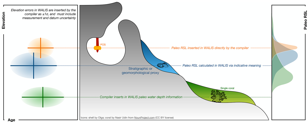
Figure 10. Three types of index points in WALIS 1.0 and associated elevation (left) and paleo RSL information (right). The figure represents the ideal case of three index points formed at the same time (overlapping ages within error bars), surveyed at different elevations but resulting in a coherent paleo RSL history (overlapping paleo RSL) once interpretation of proxies is included. POS is phreatic overgrowth on speleothems.
