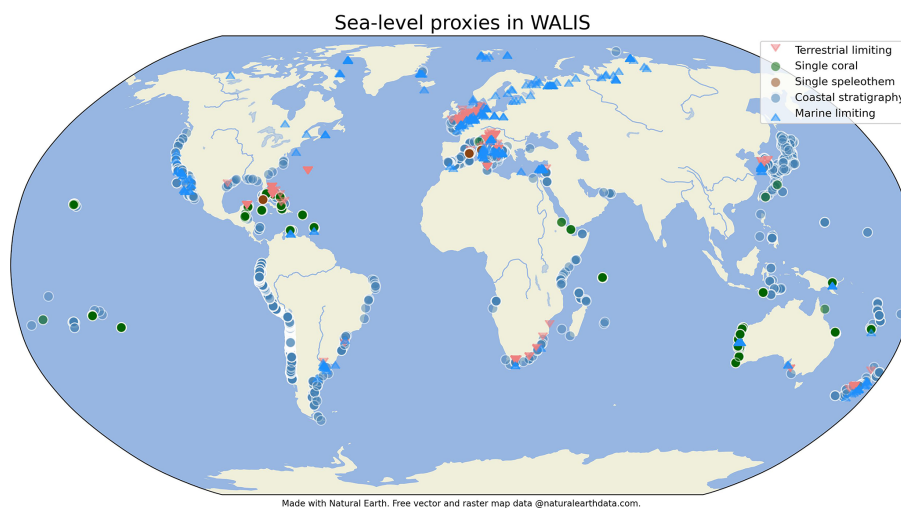
Figure 6. Location of sea-level proxies included in WALIS 1.0, divided by category. The code used to create this image is available from Rovere et al. (2022). Map made with Natural Earth, background from https://www.naturalearthdata.com (last access: 15 December 2022).
