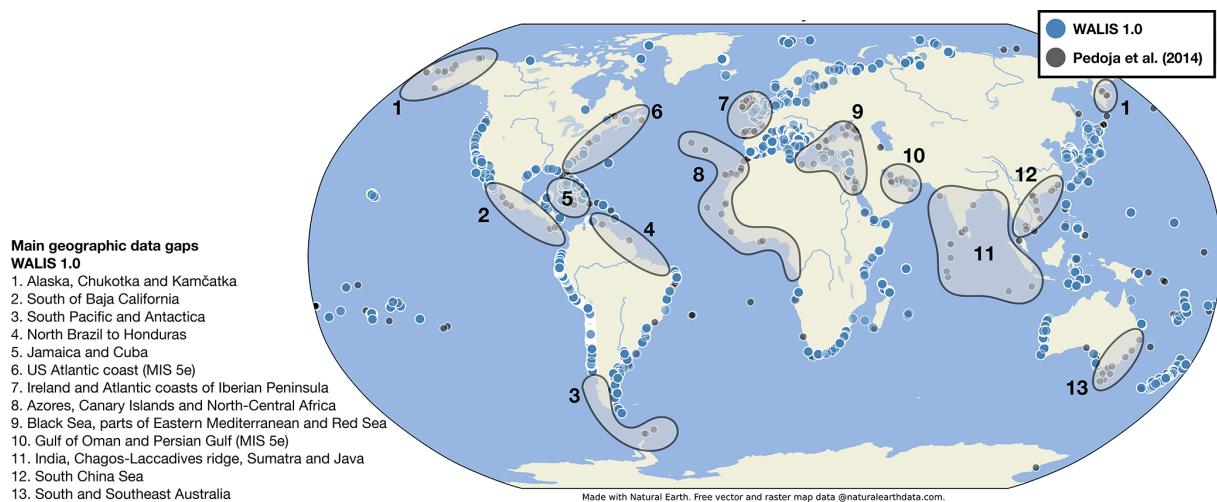
Figure 12. Comparison between sea-level proxies in WALIS 1.0 and those in the global review by Pedroja et al. (2014), indicating areas where geographic data gaps are present (see details in the main text). Map made with Natural Earth, background from https://www.naturalearthdata.com (last access: 15 December 2022).
