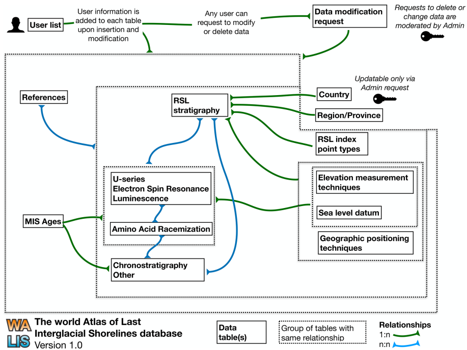
Figure 3. Database structure for WALIS. Note that the relationships among tables are managed via the PHP interface and are, therefore, not included in the database. Also not included in this scheme are the tables to report Holocene data, which are still in beta testing.
