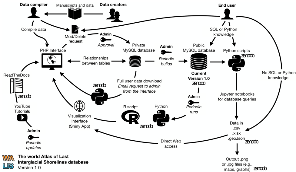
Figure 1. Overview of the WALIS platform, which includes the private and public instances of the database, the PHP data interface, and scripts in R and Python to query and visualize the data. The “Zenodo” logo indicates that the scripts/data are available in Zenodo (see Table 1 for links).
