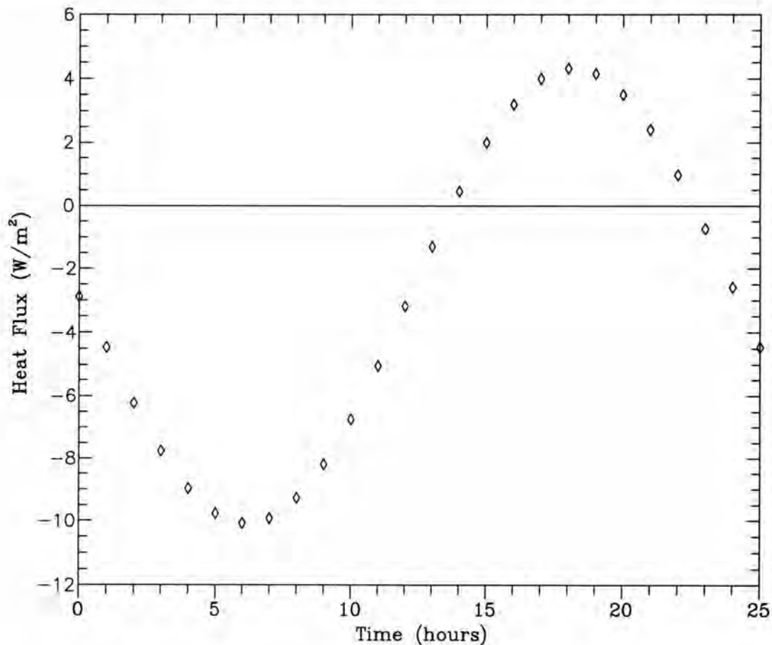
Figure 3. Test case for PROPOR. Calculated heat flux at mid-plane for H = 1 .
