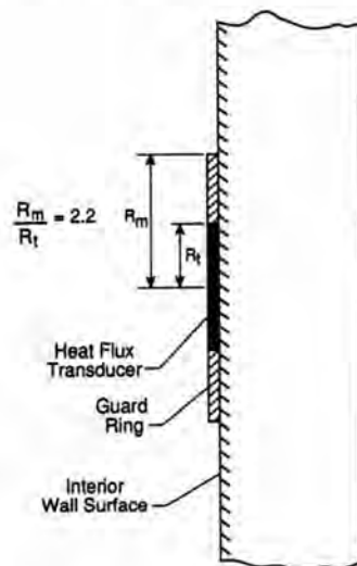
Figure 3. Method of installing a HFT at an interior wall surface.
