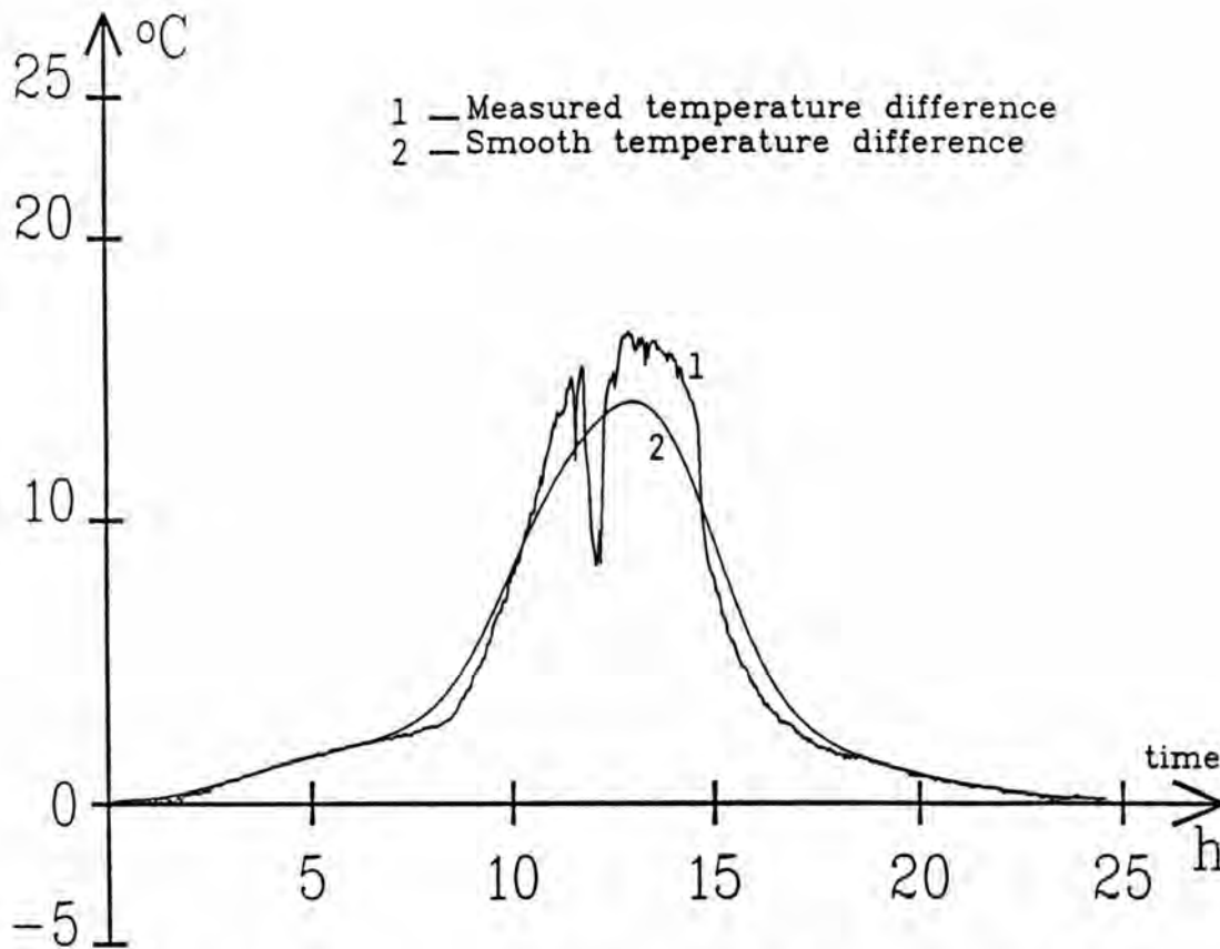
Figure 4a : Experimental temperature difference and heat smooth temperature difference.
