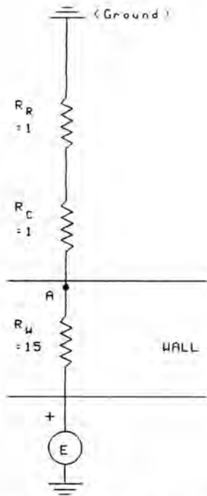
Resistances, Bare Wall Figure 2a
