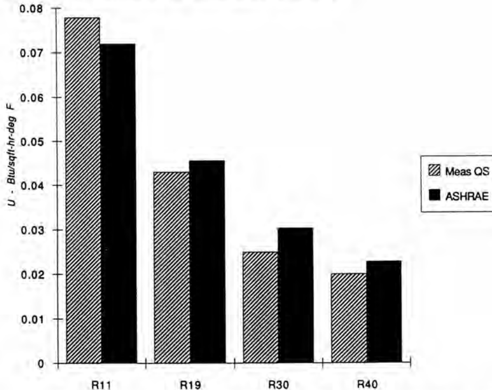
Figure 12. Measured and Handbook U-Values in Test Cell North Facing Wall
