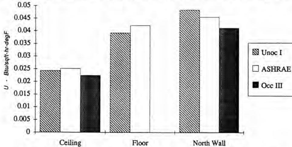
Figure 8. Measured and Handbook U-Values in MCS Test Houses Occupied and Unoccupied.
