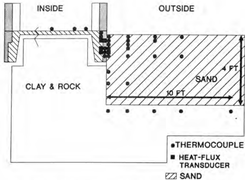
Figure 3. Instrument plane through insulated slab cross section.
