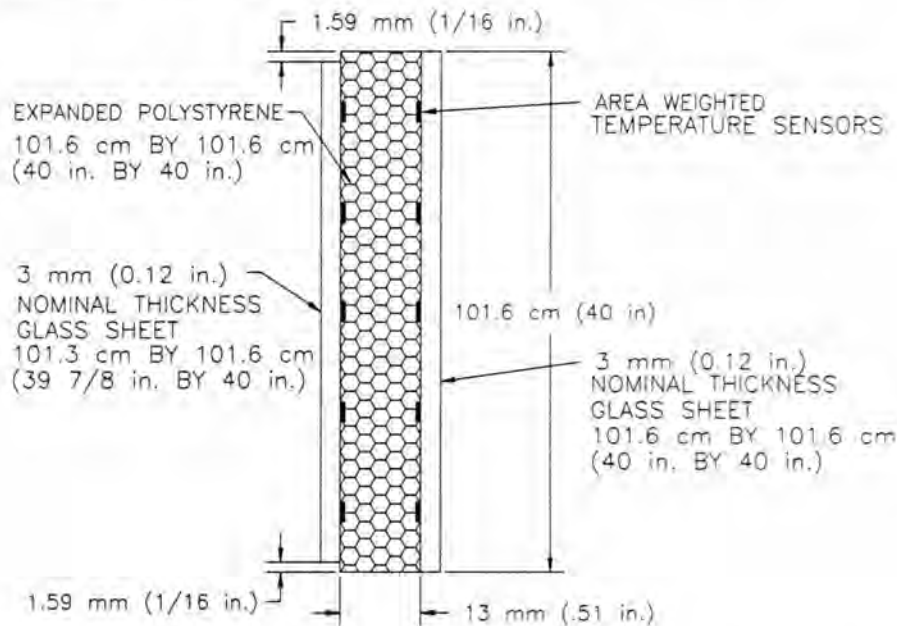
FIGURE 2. PROTOTYPE CALIBRATION TRANSFER STANDARD
