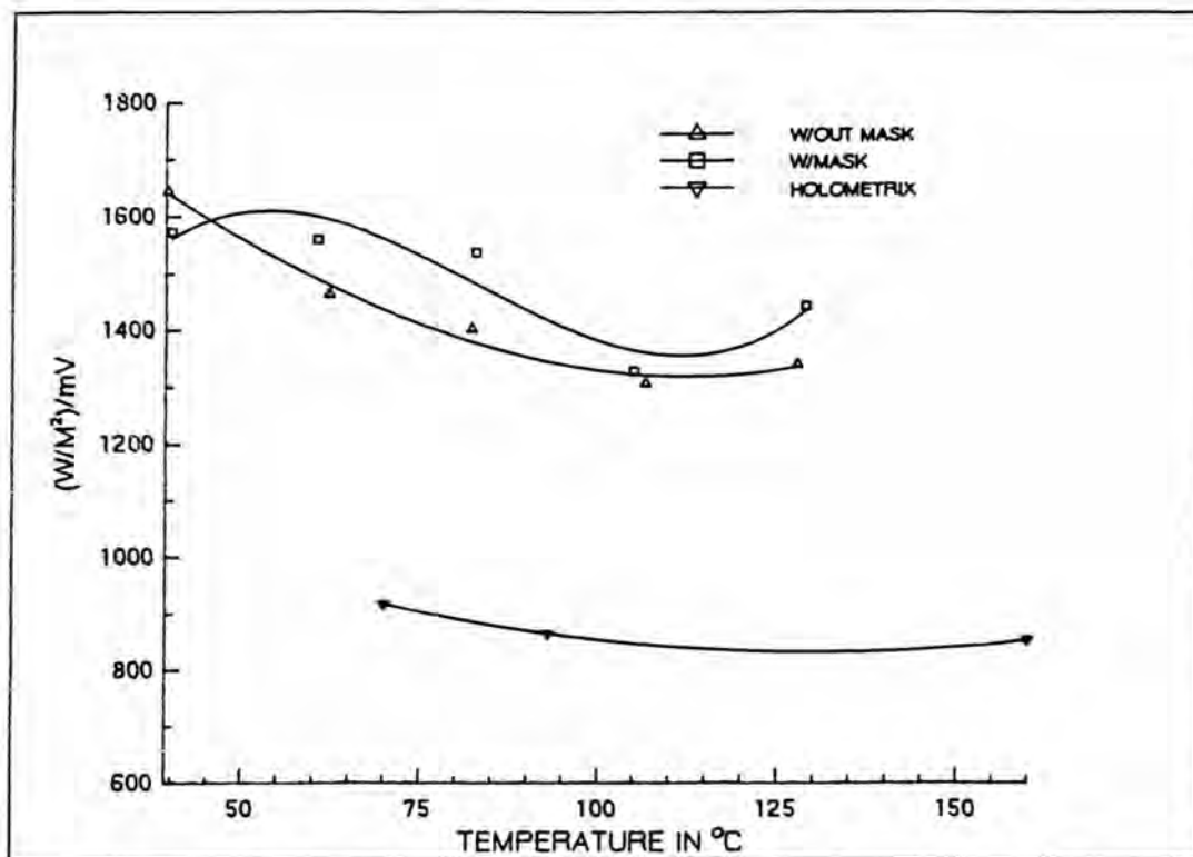
Figure 10. RdF #1286 calibration curves.
