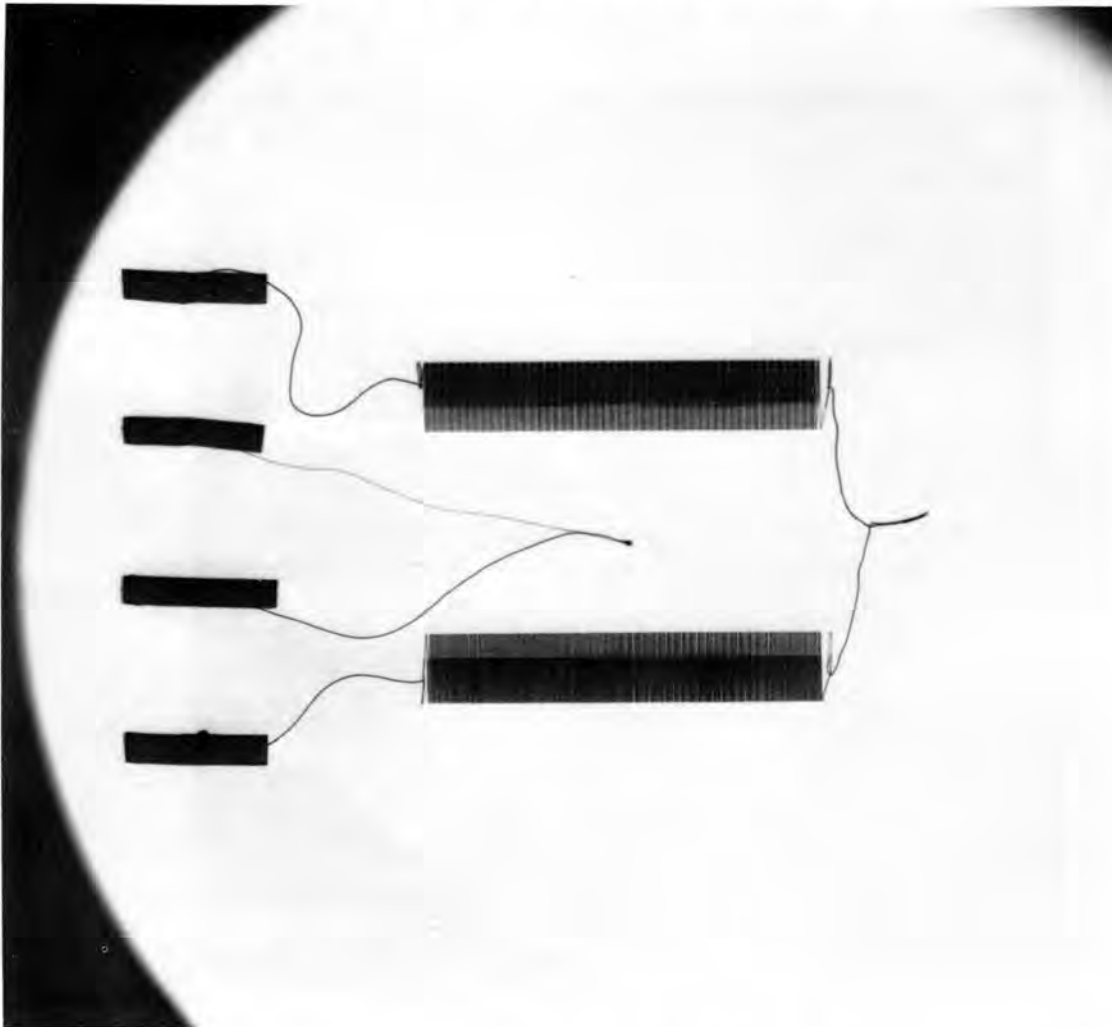
Figure 1 X-ray of a 1951 heat flux transducer showing small area sensor. Thermopile was formed by plating a material of low electrical resistivity on one-half of a winding of high electrical resistivity.
