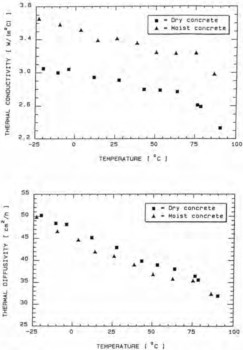
Figure 10. Thermal conductivity and diffusivity against the temperature of concrete
