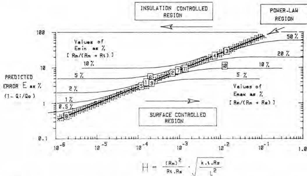
Figure 2. Locations of Example Cases from Table 1, on parametric correlation diagram.
