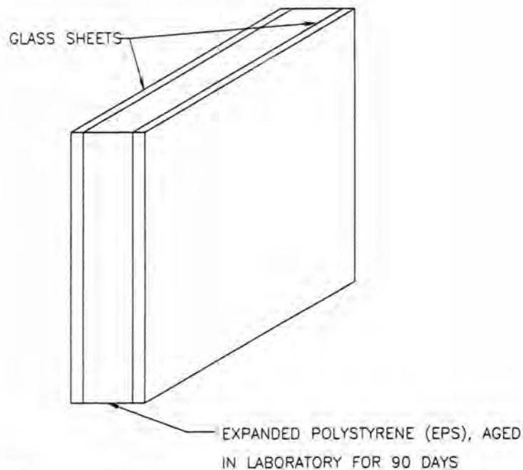
FIGURE 1. CALIBRATION TRANSFER STANDARD SCHEMATIC.
