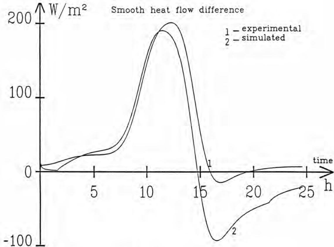
Figure 9 : Convolution of the smooth temperature difference with the same weighting function.
