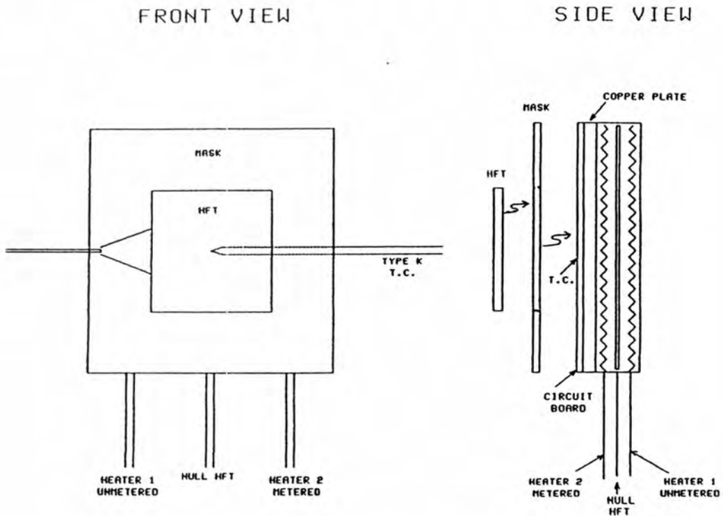
Figure 5. Thin Heating Device w/mask and HFT.
