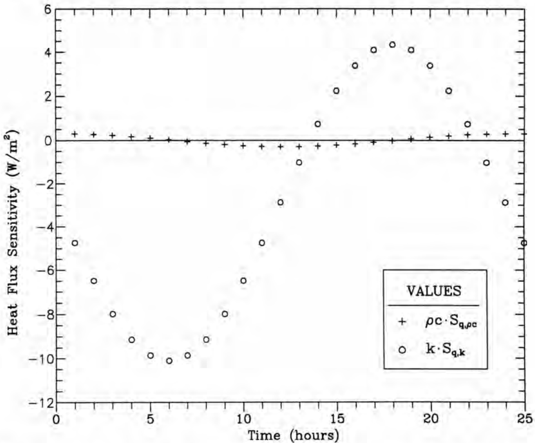
Figure 5. Test case for PROPOR. Heat flux sensitivities at mid-plane for H = 1 .
