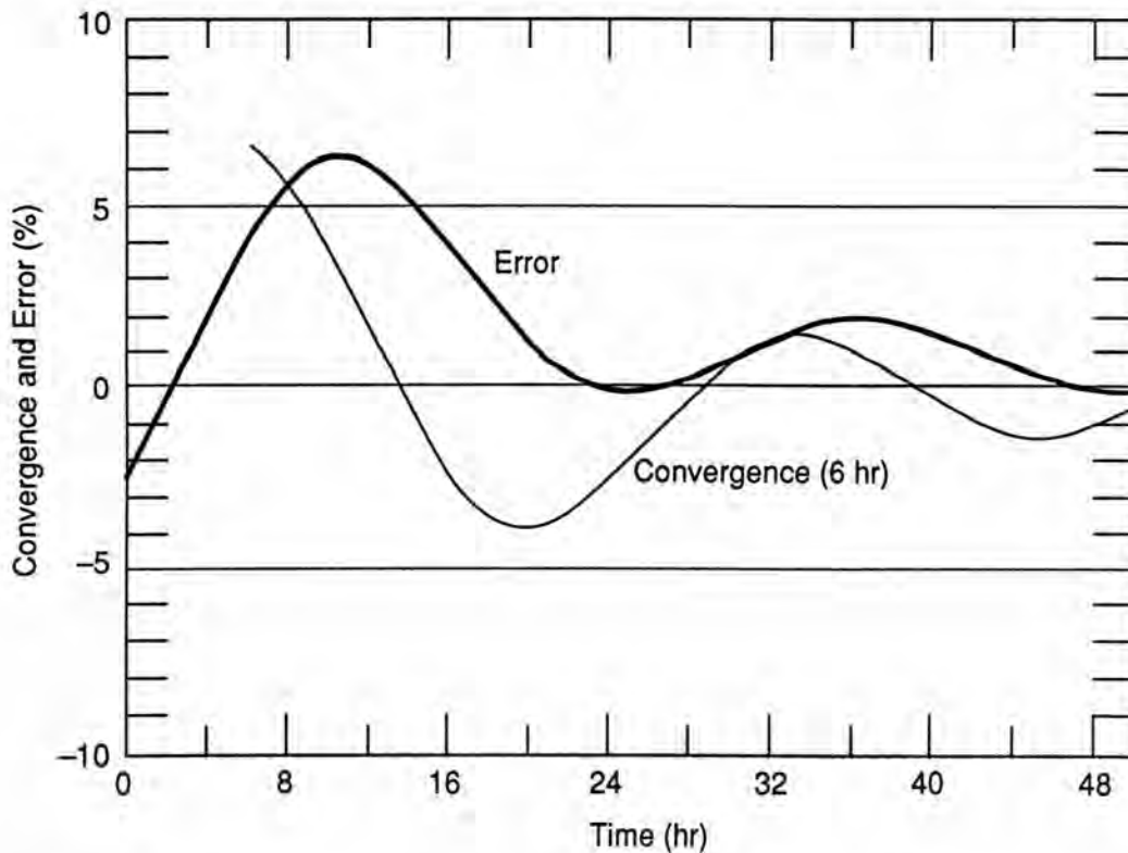
Figure 6. ERR(t) and CONV(t, 6h) for the insulated furnace case (Tables 3 and 4).
