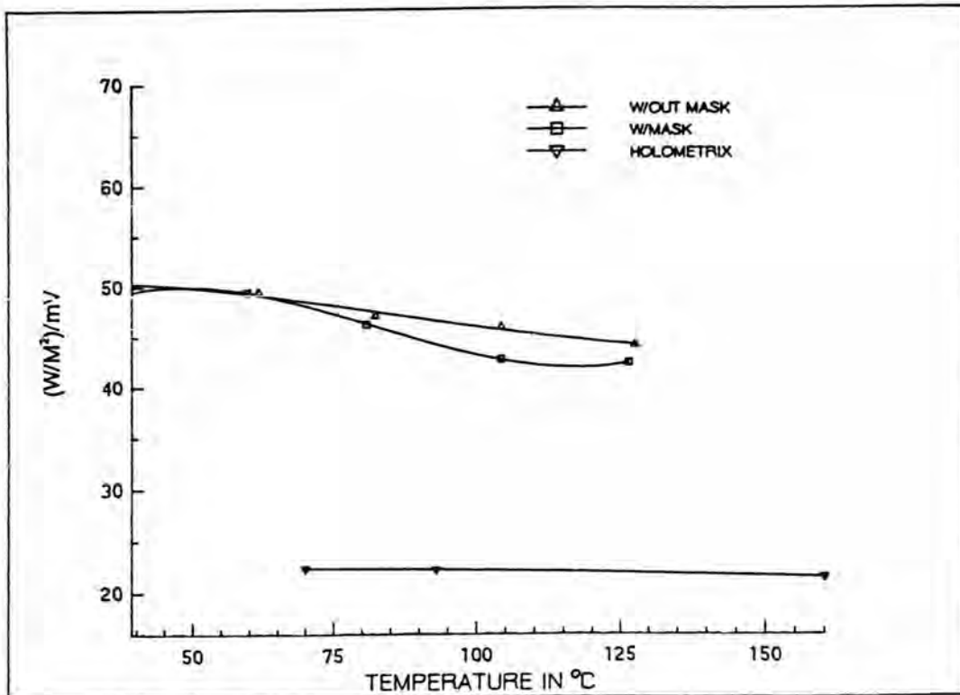
Figure 7. ITI #B-359 calibration curves.
