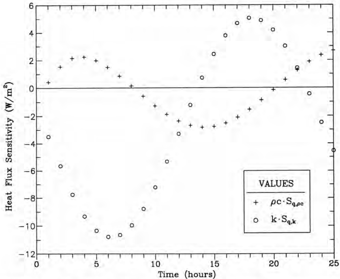
Figure 7. Test case for PROPOR. Heat flux sensitivities at mid-plane for H = 0.1 .
