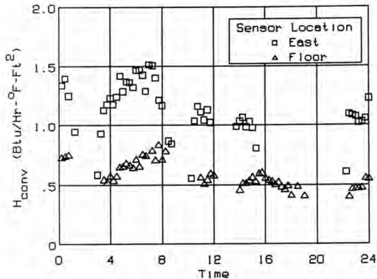
Figure 4. Variation of Convective Heat Transfer Coefficients over a 24 Hour Period
