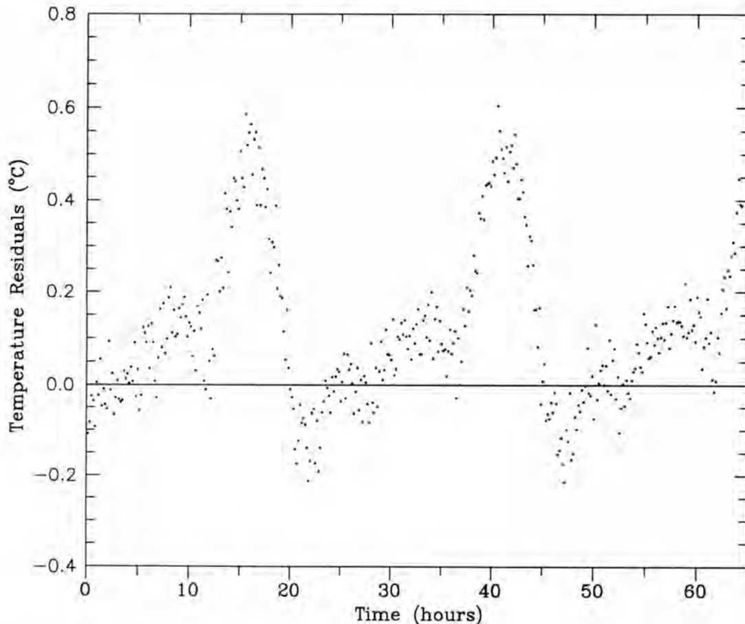
Figure 10. PROPOR analysis of SUMEPS to estimate constant properties. Temperature residuals at mid-plane for each measurement time.
