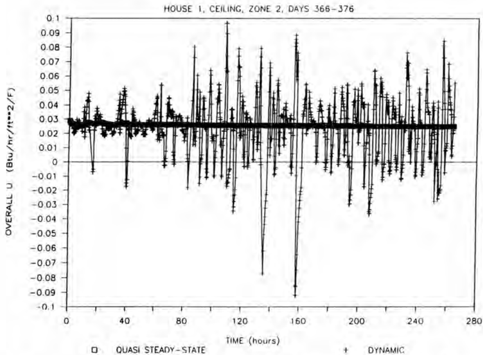
Figure 14. Developing Quasistatic U with Instantaneous Values Superimposed
