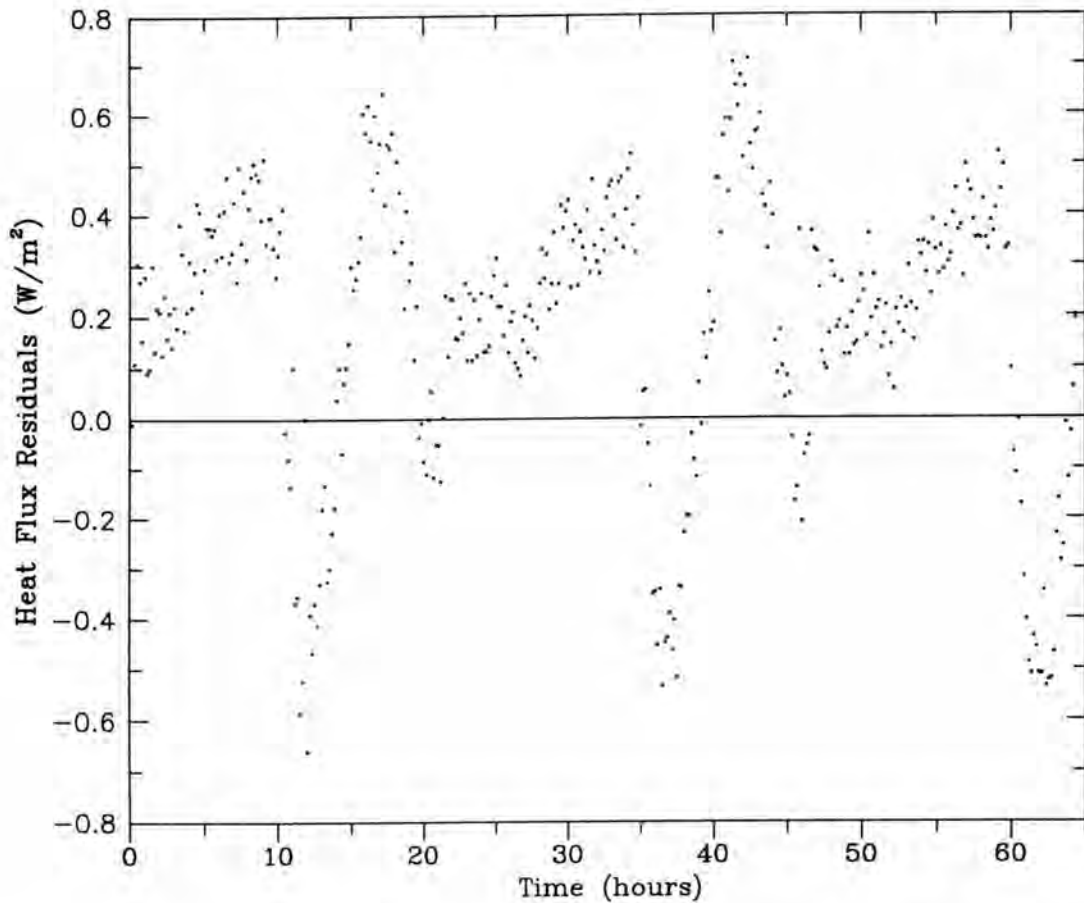
Figure 12. PROPOR analysis of SUMEPS to estimate constant properties. Heat flux residuals at mid-plane for each measurement time.
