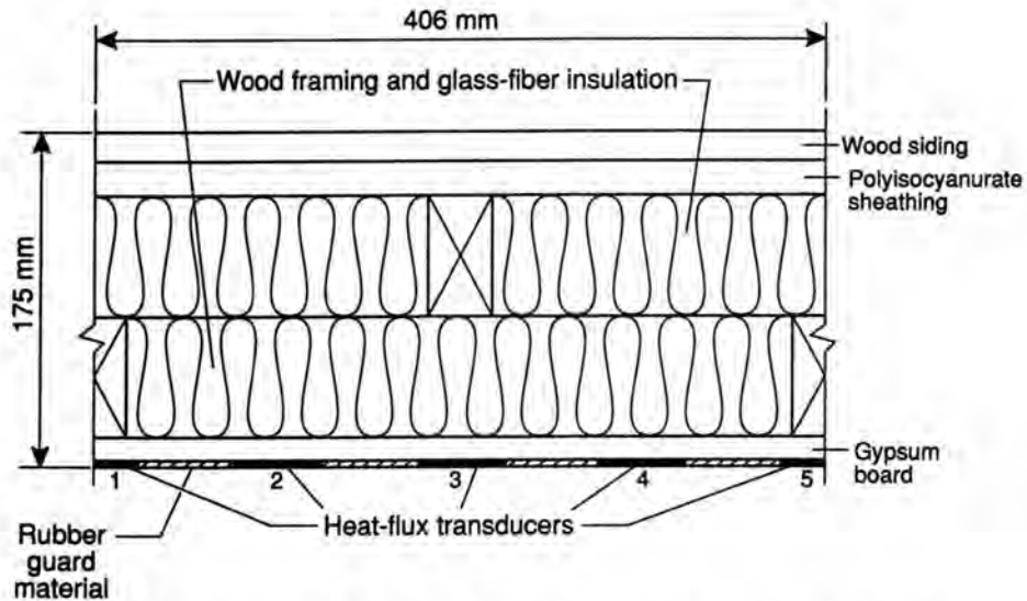
Figure 2. Cross section of the well-insulated wall specimen.
