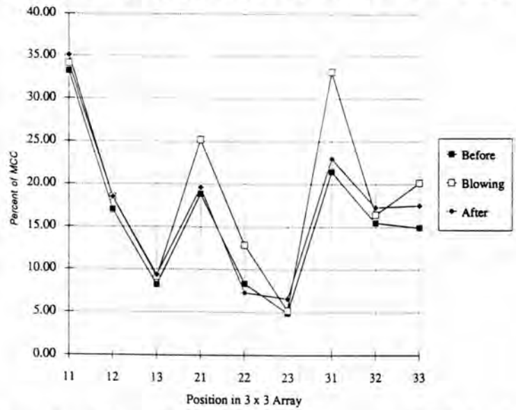
Figure 4. Effect of Forced Convection over HFT in Array Air Flow is in 13 to 31 Direction ECC Increase in Percent of MCC
