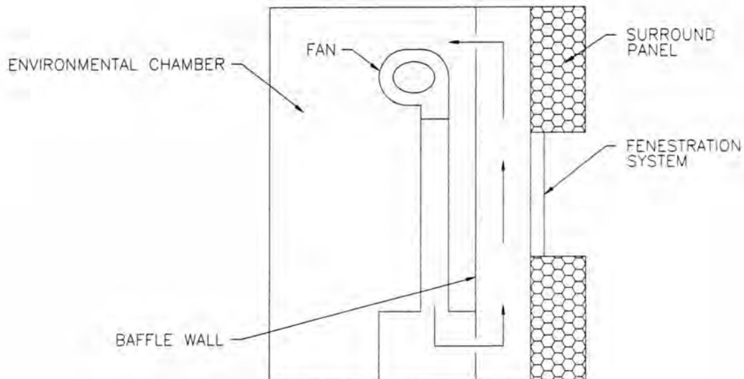
FIGURE 5. HOT BOX ENVIRONMENTAL CHAMBER, PARALLEL FLOW
