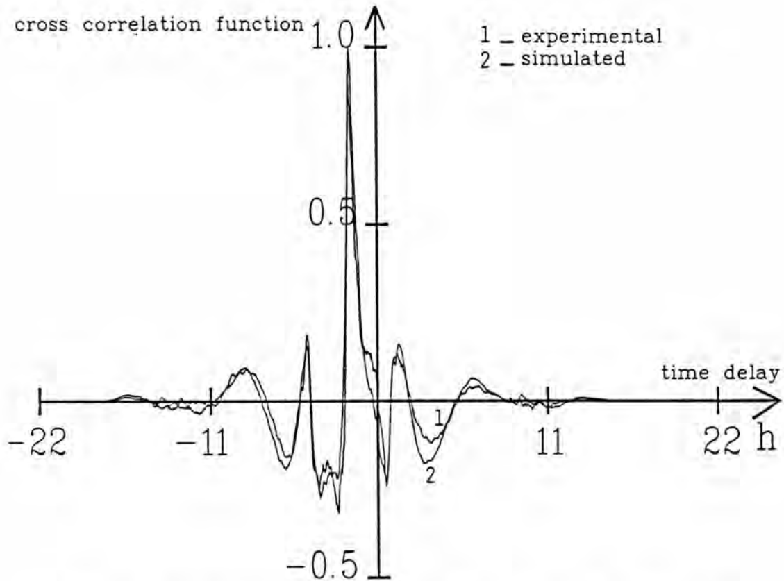
Figure 6b : Cross-correlation function (experimental) and convolution product simulated.
