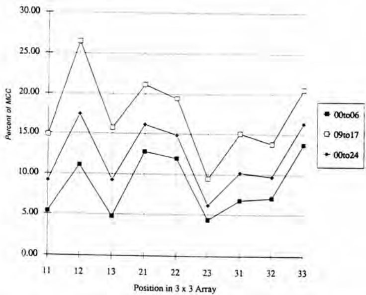
Figure 5. Effect of Occupant Induced Convection on HFT in Array ECC Increase in Percent of MCC
