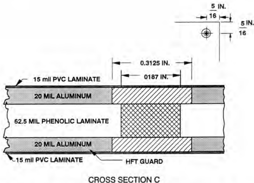
Figure 6. Cross section of heat-flux transducer guard showing holes for fasteners designed to prevent fastener contact with aluminum.
