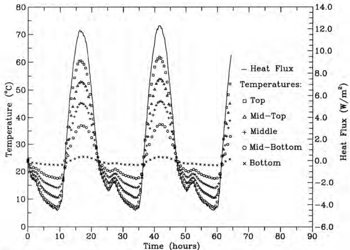
Figure 8. Heat flux and temperature profiles for test of expanded polystyrene with normal summer days yielding SUMEPS for PROPOR.
