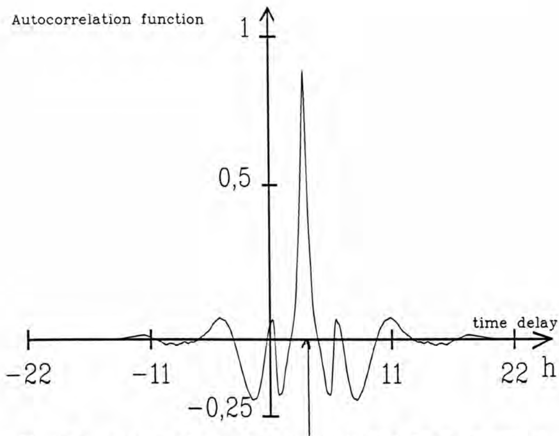
Figure 6a : Autocorrelation function of the high frequency content of the temperature difference.
