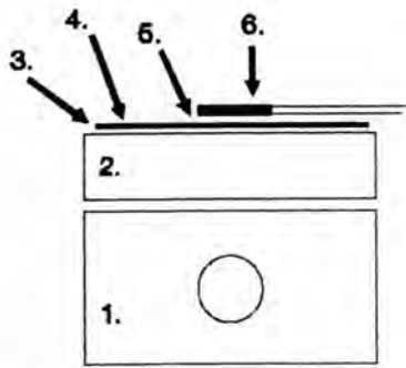
Hot Plate-Type Heat Source W/Low-k Substrate Setup Figure 3
