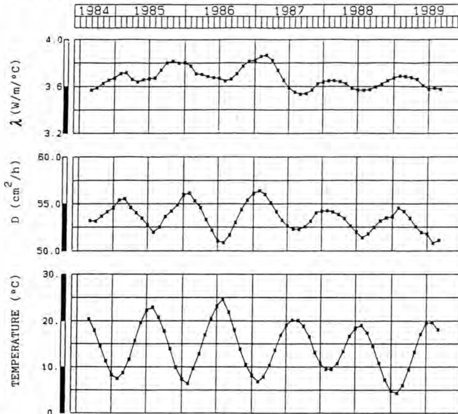
Figure 9. Thermal conductivity \lambda and thermal diffusivity D monitoring at the Ponte Cola Dam over the years 1984-1989.
