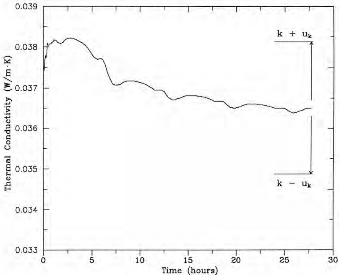
Figure 13. PROPOR analysis of CSUMEPS to estimate constant properties. Sequential values of thermal conductivity with confidence interval of final estimate.
