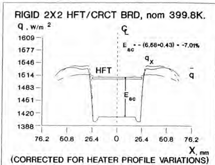
Average Heat Flux Variation vs. Distance "X" from Center Figure 11
