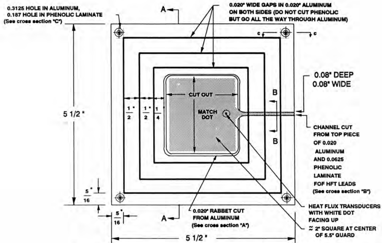
Figure 4. Top view of heat-flux transducer guard for 2- x 2-in. HFT.
