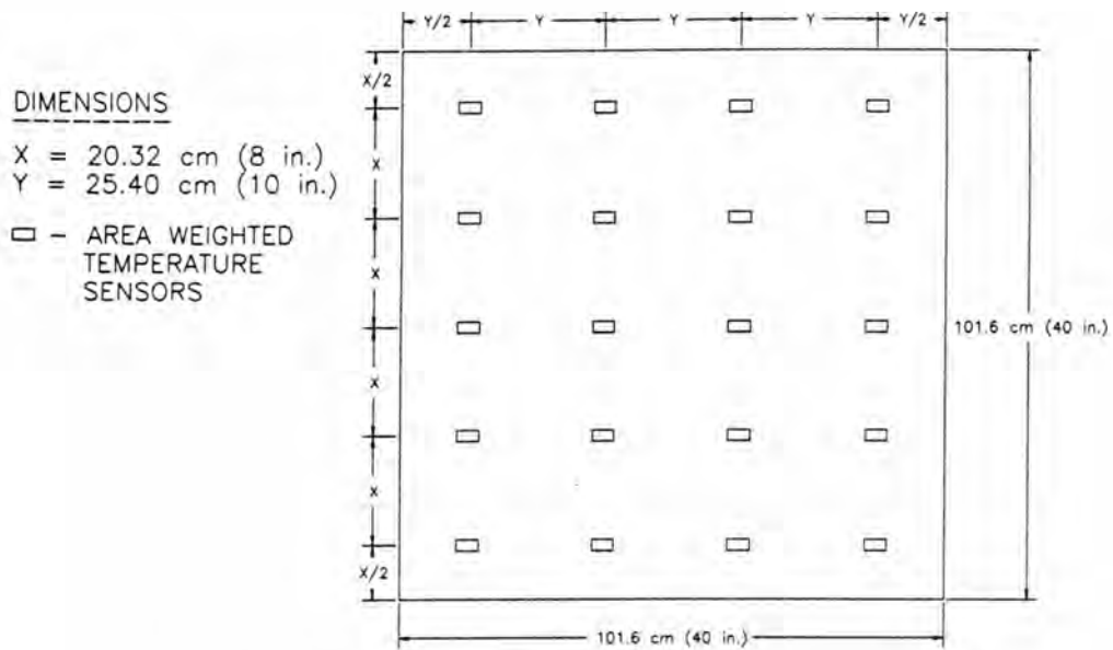
FIGURE 3. TEMPERATURE SENSOR LOCATION ON PROTOTYPE CALIBRATION TRANSFER STANDARD.
