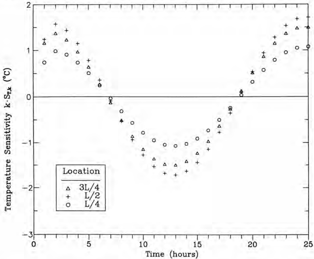
Figure 4. Test case for PROPOR. Temperature sensitivities at internal locations for H = 1 .
