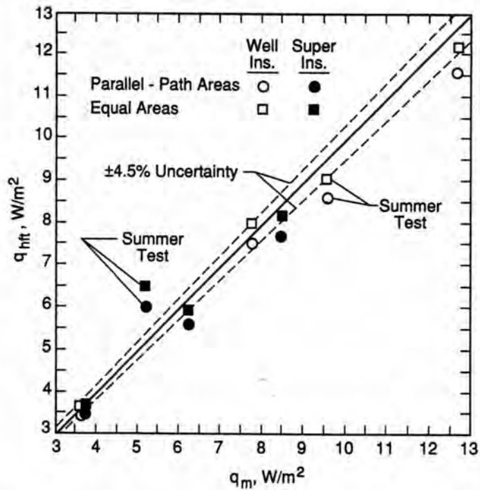
Figure 6. Comparison between the steady-state HFT and CHB measurements for the well-insulated and superinsulated wall specimens.
