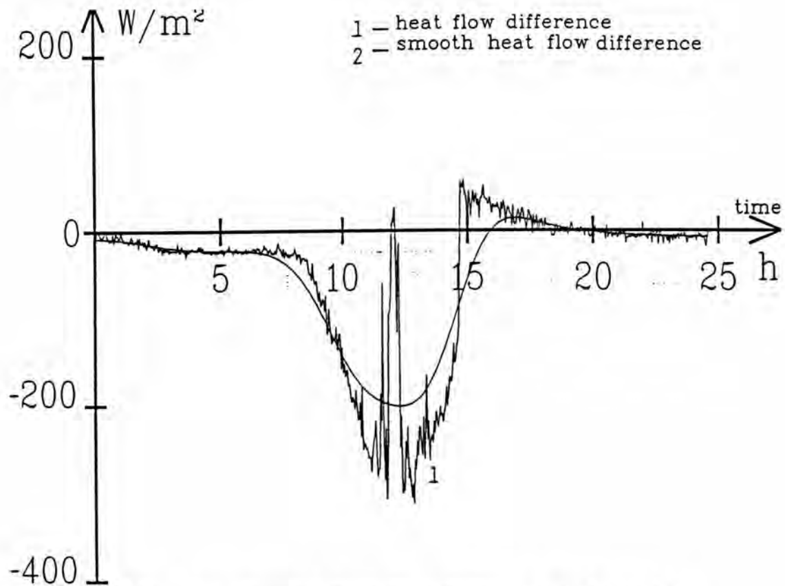
Figure 4b : Experimental heat flow difference and smooth heat flow difference.
