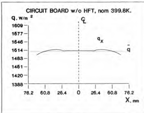
Figure 10a Average Heat Flux Variation vs. Distance "X" from Center
