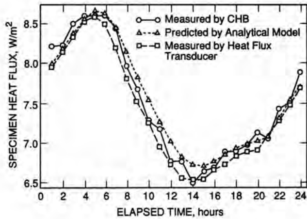
b. Plot of heat fluxes versus time.
