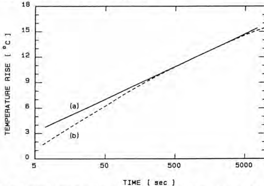
Figure 1. Comparison between the ideal linear heat source (a) and the experimental thermal probe response (b).
