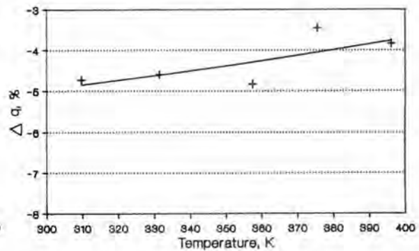
Figure 12b Film HFT Flux Error Trend (versus Surface Temperature)
