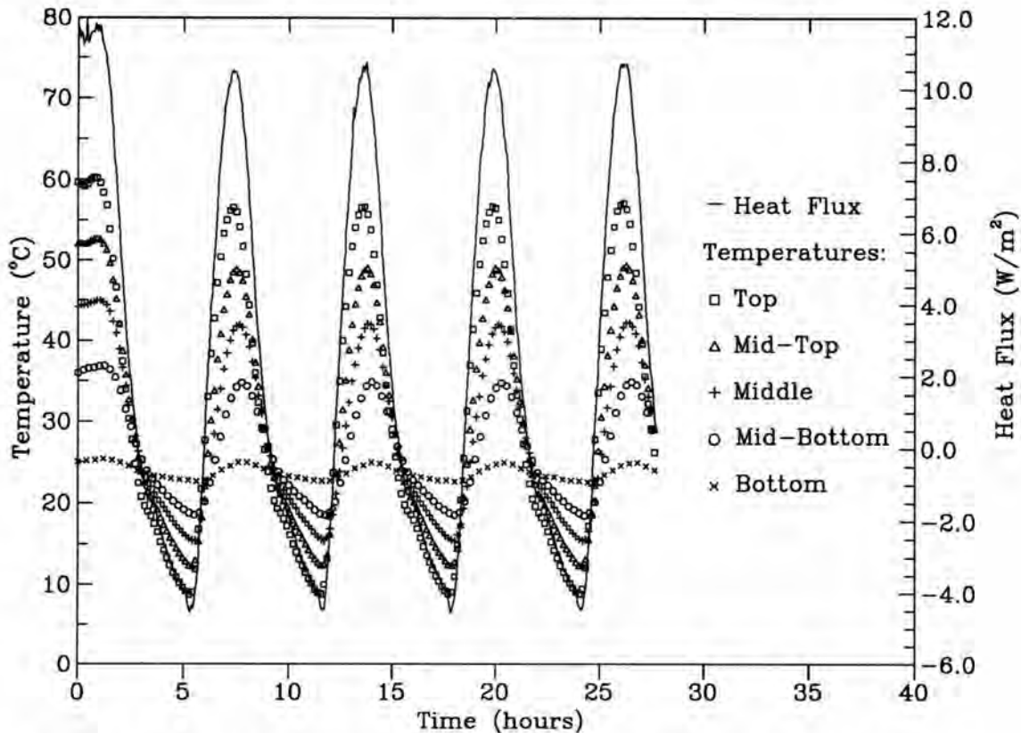
Figure 9. Heat flux and temperature profiles from test of expanded polystyrene with compressed summer days yielding CSUMEPS for PROPOR.
