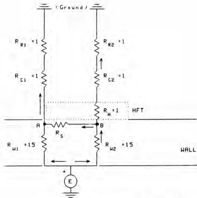
Resistances, Wall w/HFT Figure 2b
