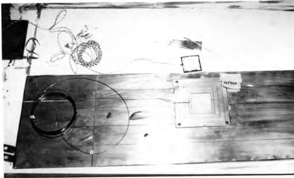
Figure 9. Larger plate with machined grooves and 0.14- x 0.14-m (5.5- x 5.5-in.) guard.
