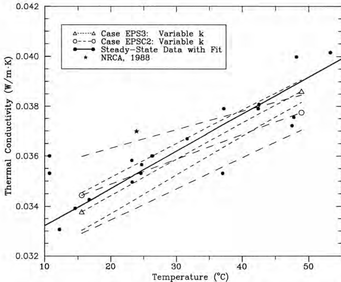
Figure 19. Summary of results from steady-state and dynamic data to estimate thermal conductivity of expanded polystyrene insulation.
