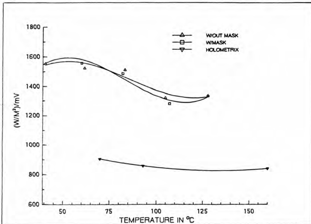
Figure 9. RdF #1285 calibration curves.
