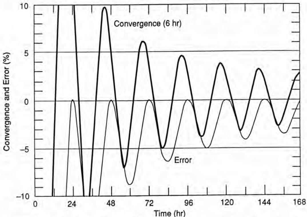
Figure 7. ERR(t) and CONV(t,6h) for the cryogenic storage case (Tables 3 and 4).
