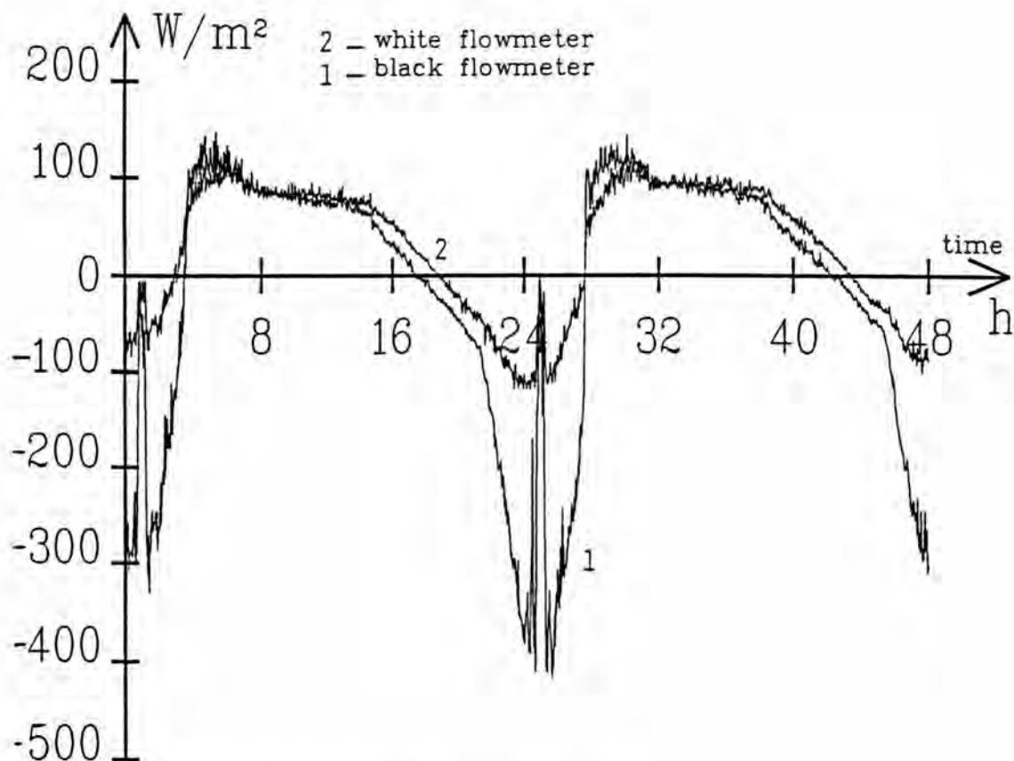
Figure 1a. Plot of the heat fluxes measured.
