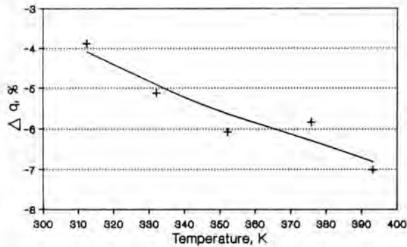
Figure 12a Rigid 2X2 HFT Flux Error Trend (versus Surface Temperature)
