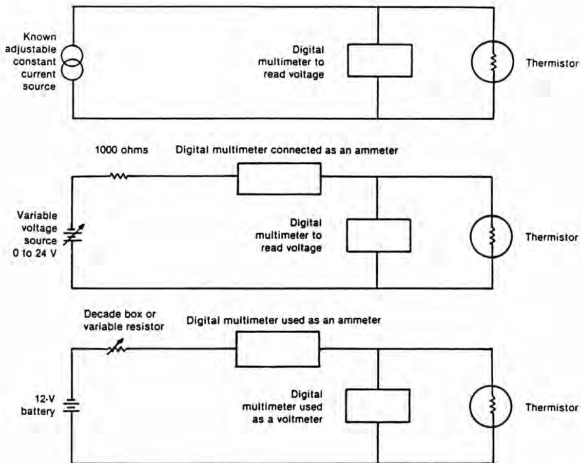
Figure 3. Three possible circuit configurations.
