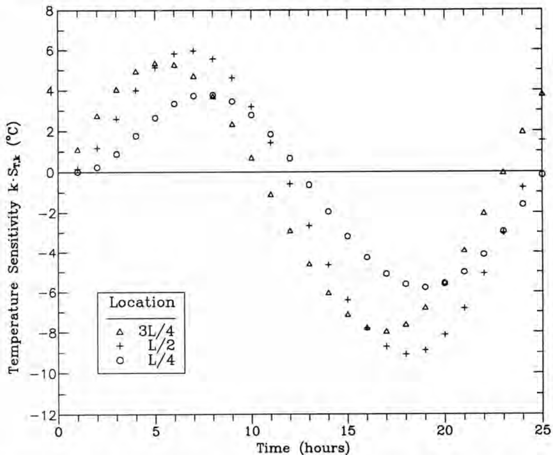
Figure 6. Test case for PROPOR. Temperature sensitivities at internal locations for H = 0.1 .
