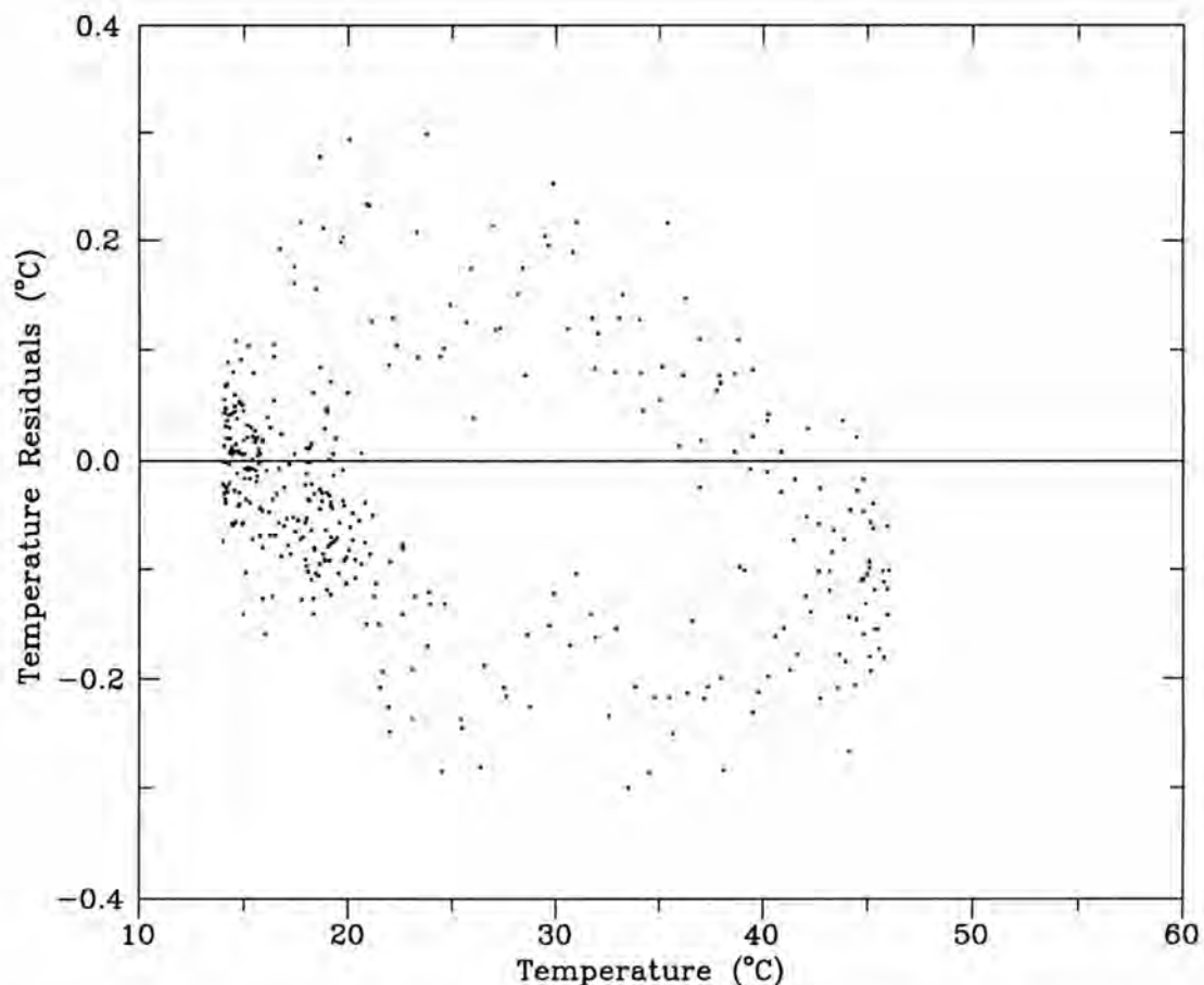
Figure 18. PROPOR analysis of SUMEPS to estimate the temperature dependence of thermal conductivity. Temperature residuals at mid-plane as a function of the measured temperature.
