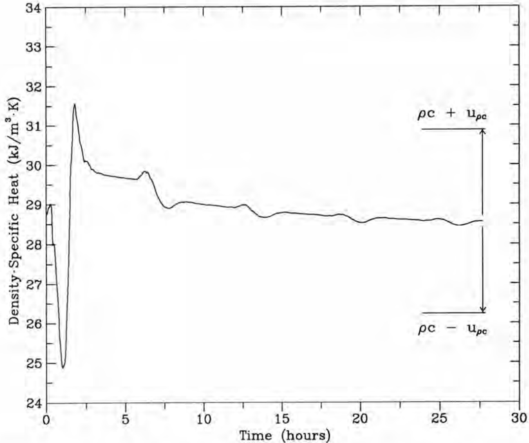
Figure 14. PROPOR analysis of CSUMEPS to estimate constant properties. Sequential values of density \times specific heat with confidence interval of final estimate.
