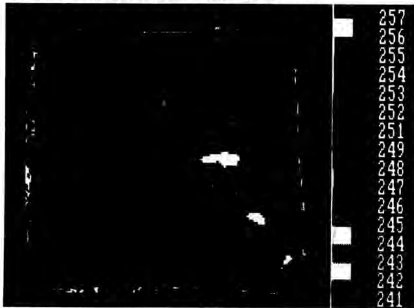
Temperature Map, Circuit Board W/O HFT, nom. 399.8K (260 ^{\circ}\text{F} ) Figure 5
