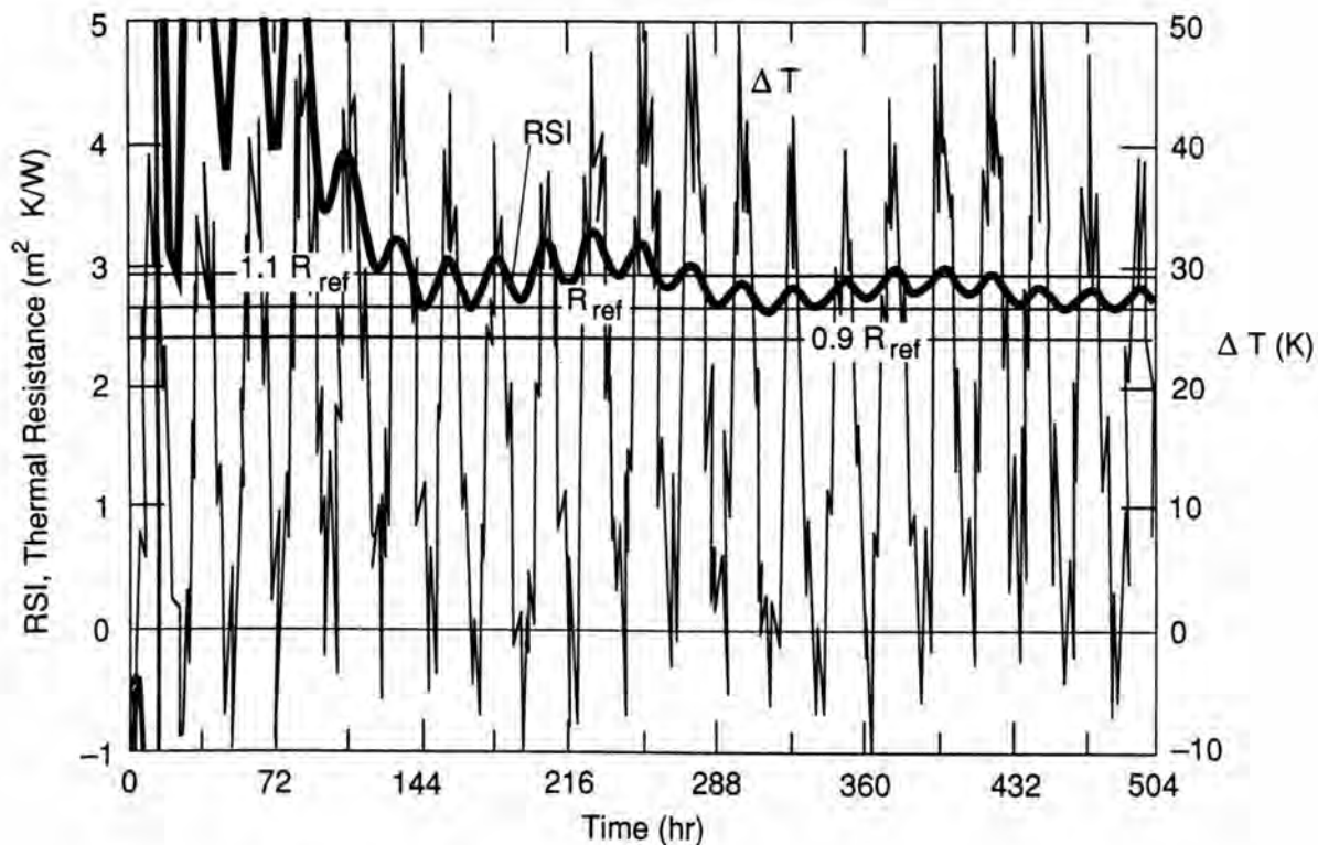
Figure 1. \Delta T and R_e for the lightweight, insulated wall example and the multiple-temperature frequency case (Table 4).
