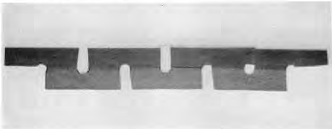
Figure 2 A bimetallic ribbon notched to form a series of thermocouples for the thermopile in the heat flux transducers.
