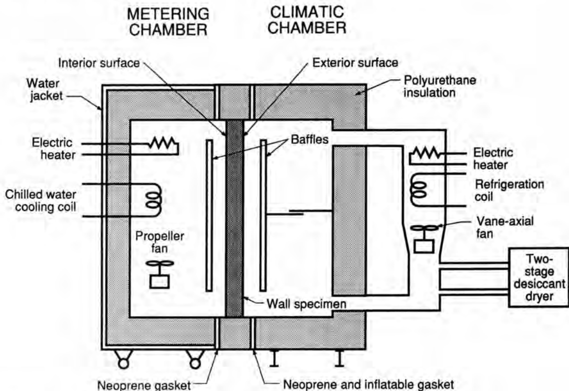
Figure 4. Calibrated-Hot-Box test procedure.
