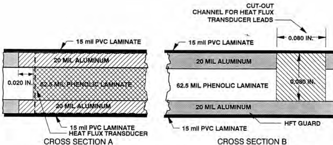
Figure 5. Cross section of heat-flux transducer guard showing lead wire channel and rabbet cut around the HFT opening to prevent aluminum from contacting the HFT.
