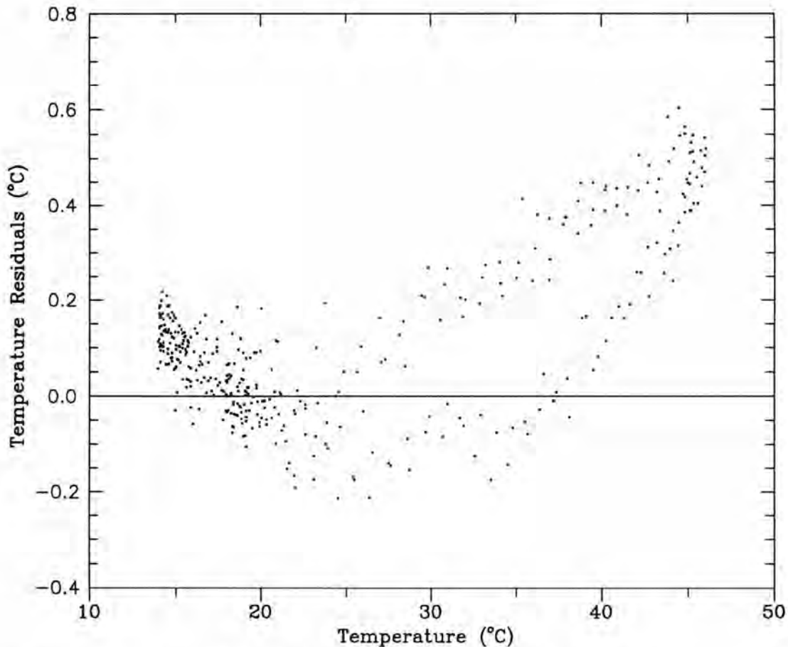
Figure 11. PROPOR analysis of SUMEPS to estimate constant properties. Temperature residuals at mid-plane as a function of the measured temperature.
