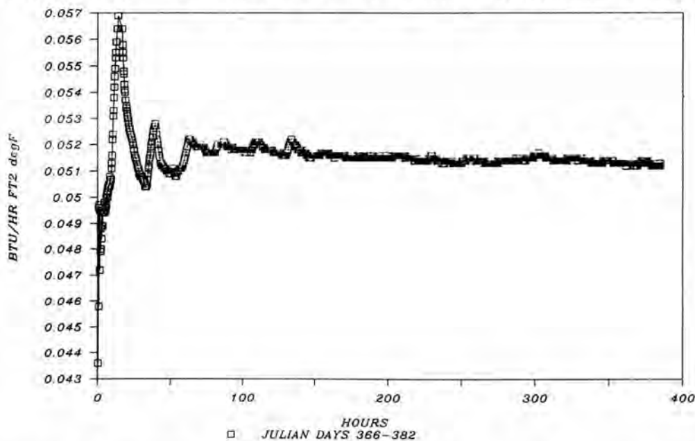
Figure 7. Quotients of Successive Heat Flux Sums over Successive Inside Air-Outside Air Temperature Differences
