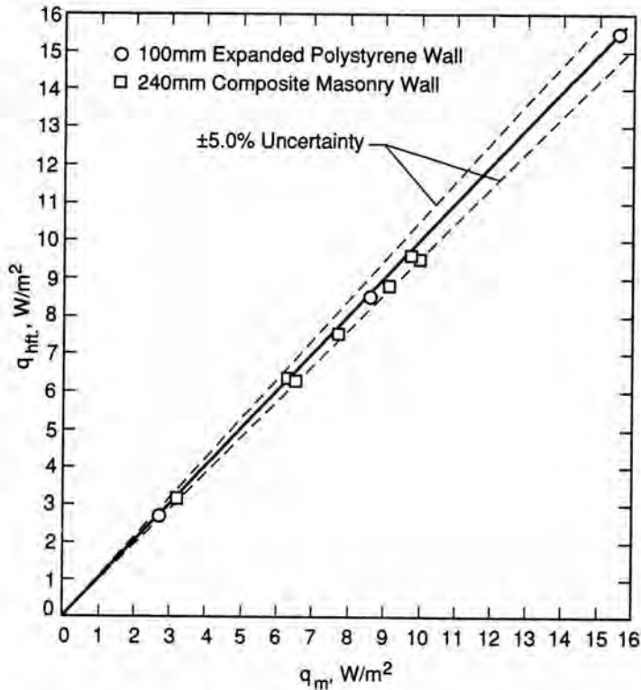
Figure 5. Comparison between the steady-state HFT and CHB measurements for the polystyrene and composite masonry walls.
