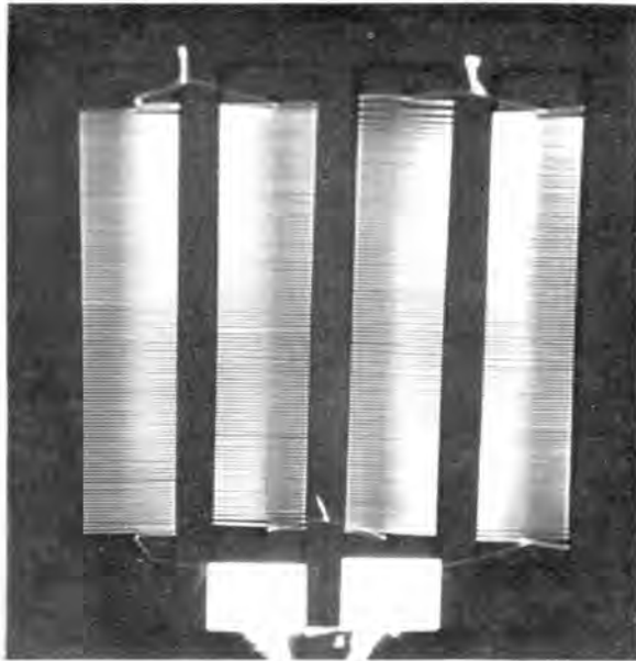
Figure 13a X-Ray of Rigid 2X2 HFT
