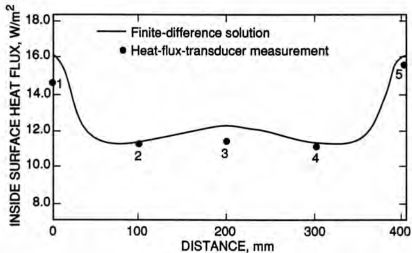
Figure 7. Comparison between steady-state HFT measurements and predictions using a finite-difference model.
