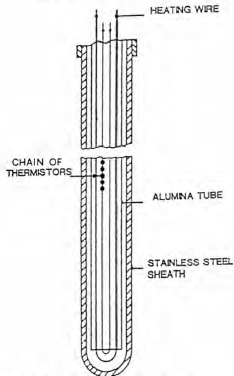
Figure 4. Details of the heating probe.
