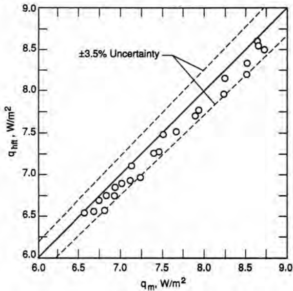
c. Heat flux comparison.
