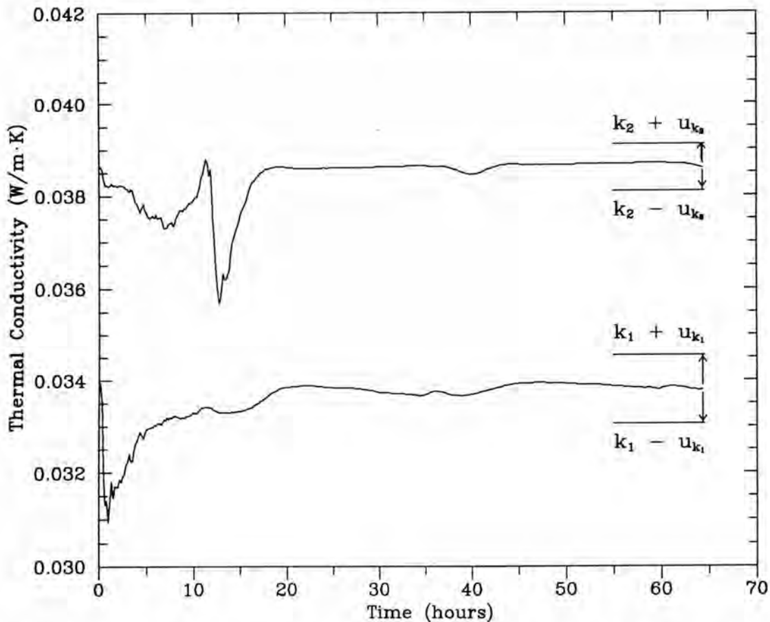
Figure 16. PROPOR analysis of SUMEPS to estimate variable thermal conductivity. Sequential values of thermal conductivities with confidence intervals of final estimates.
