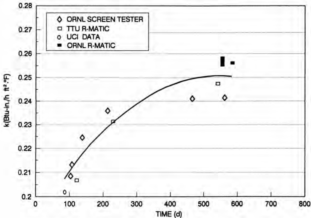
Figure 15. Laboratory thermal conductivity measurements of experimental XEPS and thermal aging predictions.
