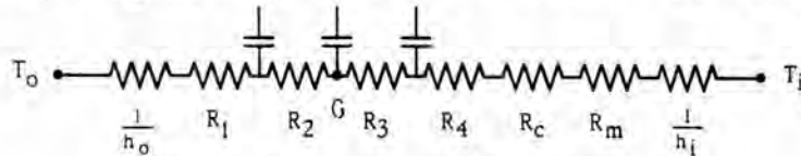
Figure 1. Envelope Thermal Circuit
