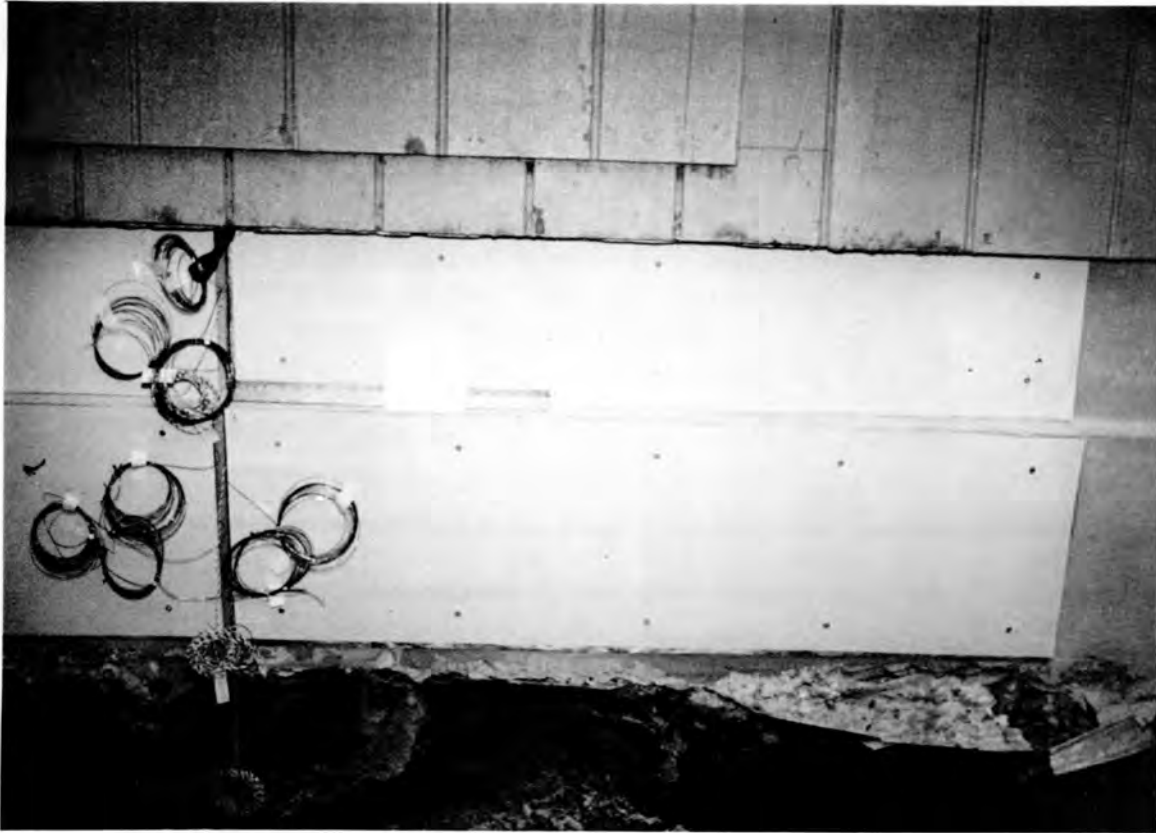
Figure 13. Plates fastened to foundation wall.
