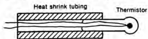
Figure 2. Thermal conductivity probe.
