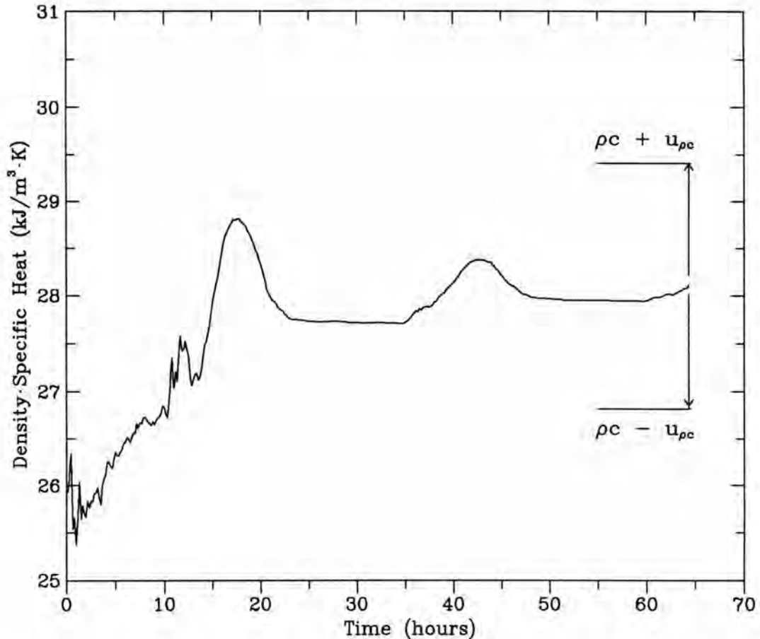
Figure 17. PROPOR analysis of SUMEPS to estimate the temperature dependence of thermal conductivity. Sequential values of the product of density \times specific heat with confidence interval of final estimate.
