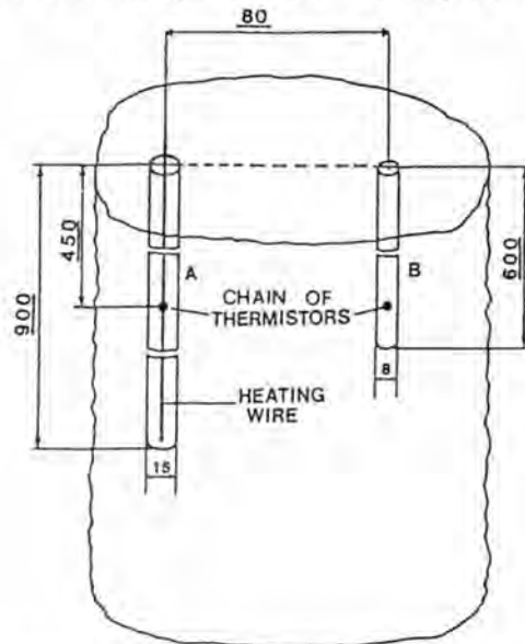
Figure 5. Configuration of the TLPP test (all the dimensions in mm).
