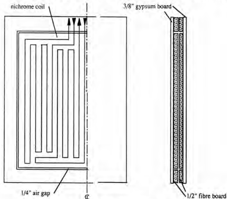
Figure 2. Heated Test Panel
