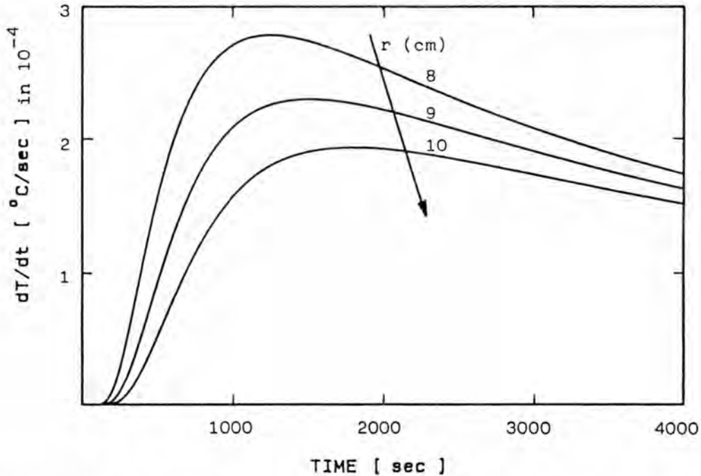
Figure 2. Plot of equation 3 for \lambda = 3.6 (W/m/°C), D = 50 (cm 2 /h), q = 0.34 (W/cm).
