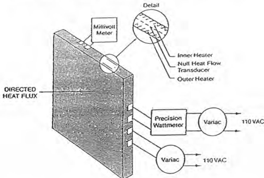
Figure 1. Series 1000-S Heat Flux Standard Assembly (Courtesy of ITI).
