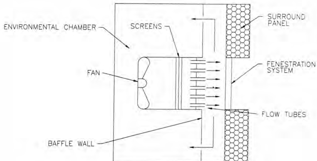
FIGURE 6. HOT BOX ENVIRONMENTAL CHAMBER, PERPENDICULAR FLOW.
