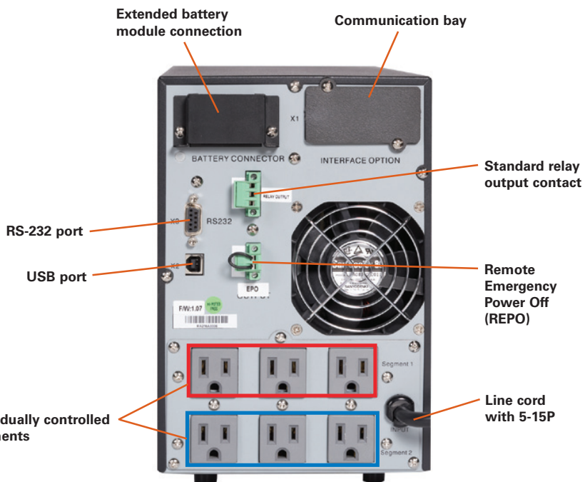
UPS rear panel (PW9130L1500T-XL)
